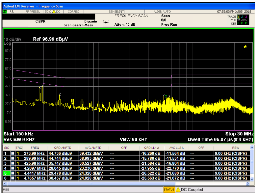
Plot 7-14. Line Conducted Plot (N, Keyboard)
