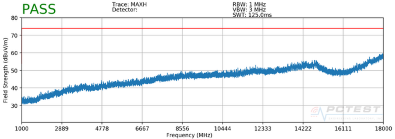
Plot 7-8. Radiated Spurious Plot above 1GHz (S-Pen)
