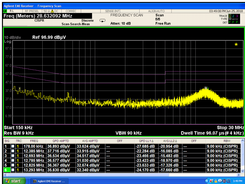
Plot 7-9. Line Conducted Plot (L1, Data Transfer via USB)
