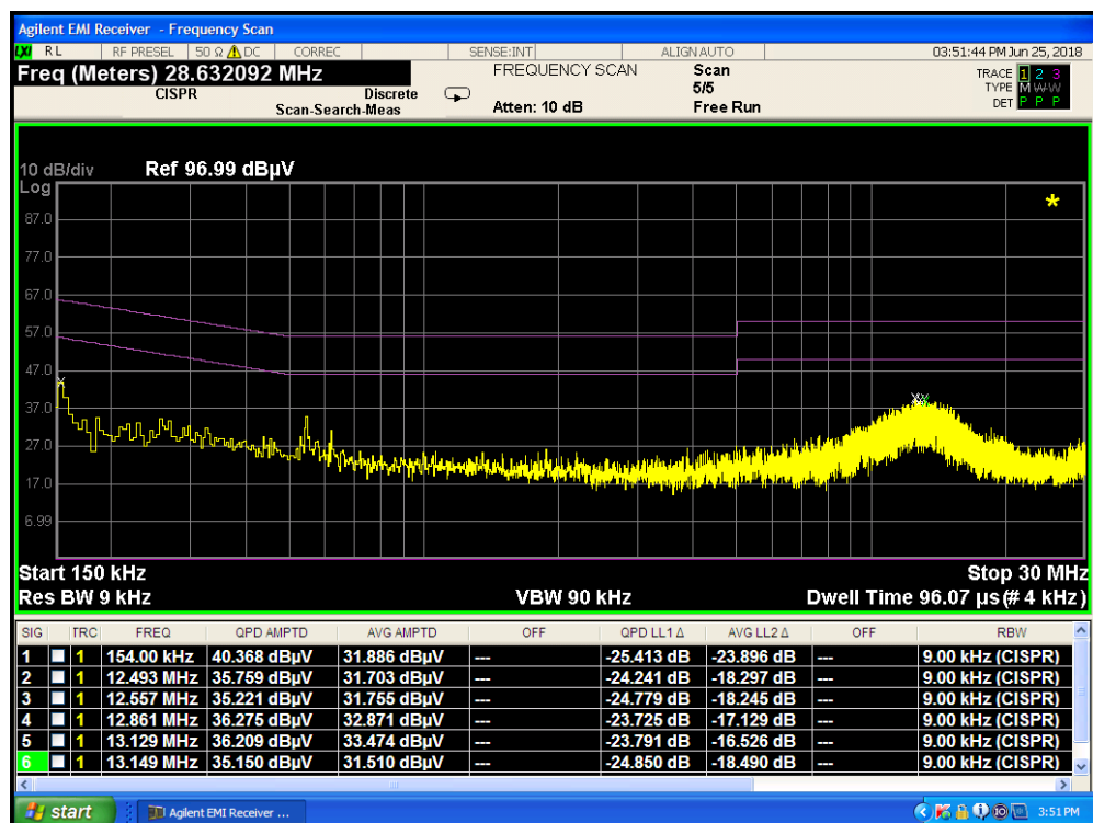
Plot 7-10. Line Conducted Plot (N, Data Transfer via USB)
