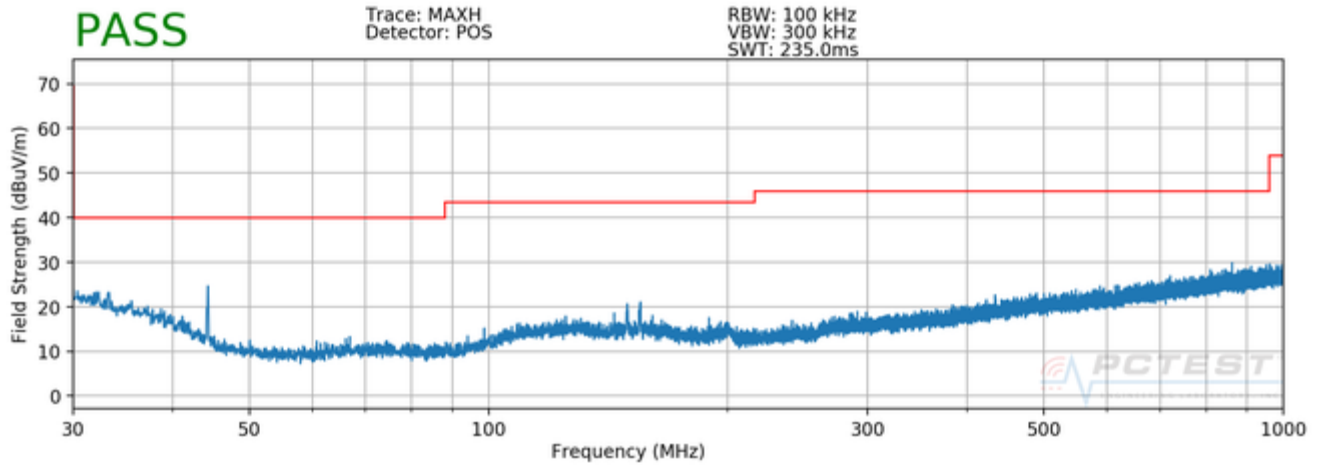
Plot 7-7. Radiated Spurious Plot below 1GHz (S-Pen)
