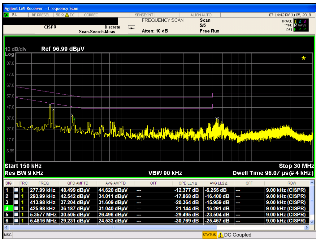
Plot 7-16. Line Conducted Plot (N, S-Pen)
