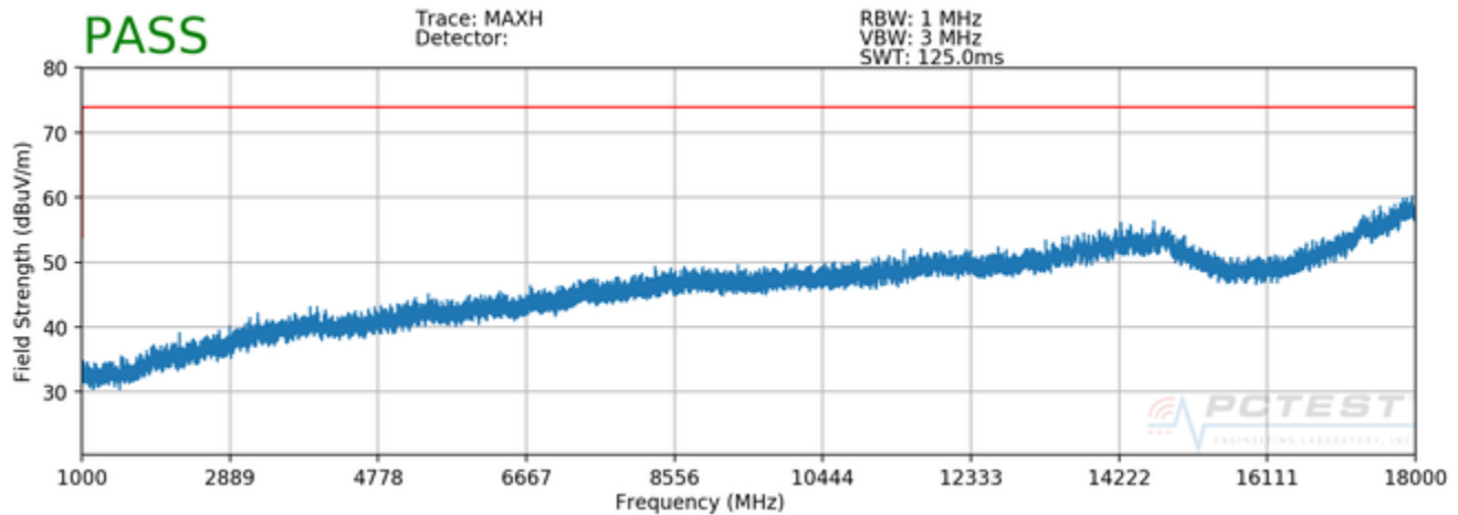
Plot 7-6. Radiated Spurious Plot above 1GHz (Keyboard)
