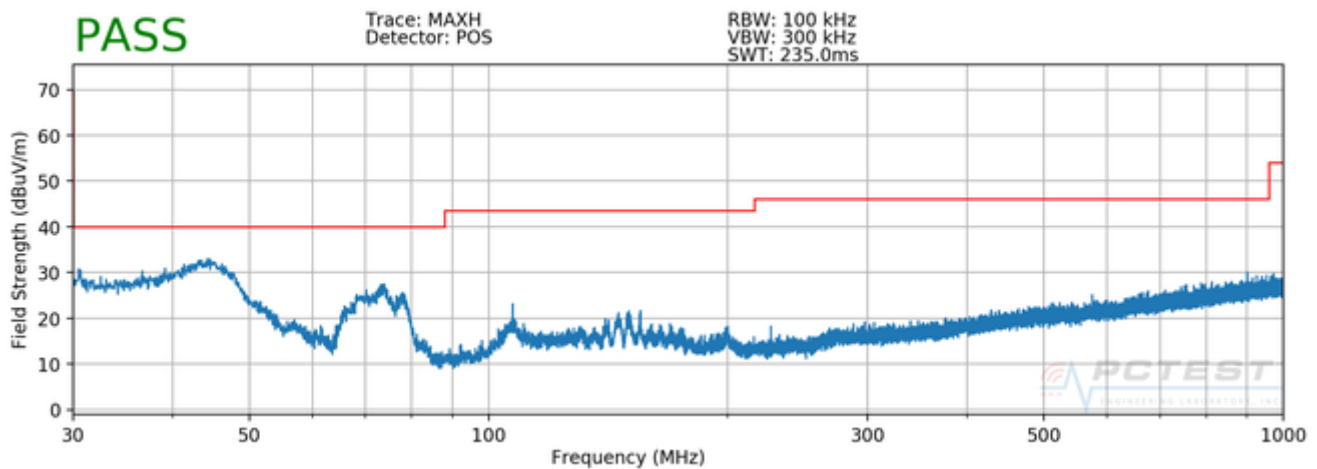
Plot 7-3. Radiated Spurious Plot below 1GHz (Charging Dock)
