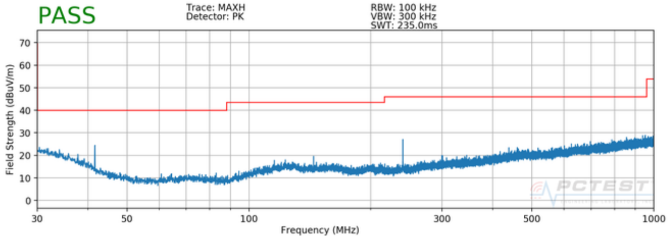
Plot 7-1. Radiated Spurious Plot below 1GHz (Data Transfer via USB)
