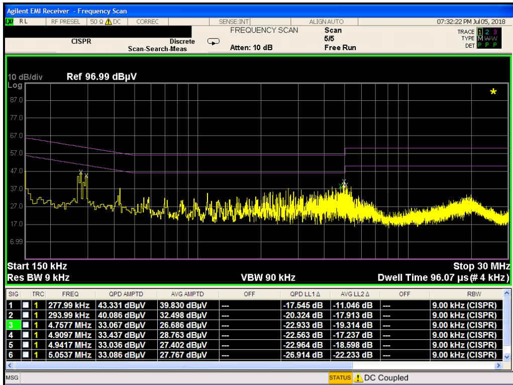
Plot 7-13. Line Conducted Plot (L1, Keyboard)
