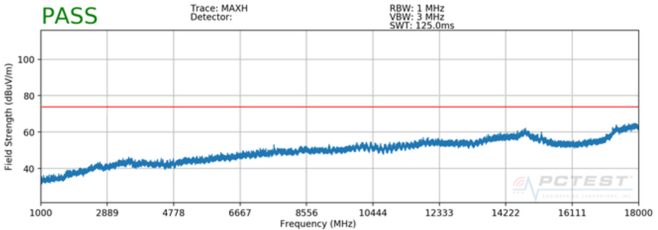
Plot 7-2. Radiated Spurious Plot above 1GHz (Data Transfer via USB)
