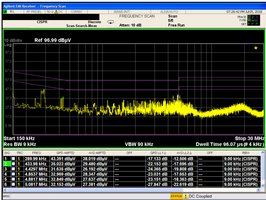
Plot 7-11. Line Conducted Plot (L1, Charging Dock)
