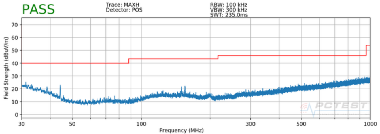
Plot 7-5. Radiated Spurious Plot below 1GHz (Keyboard)
