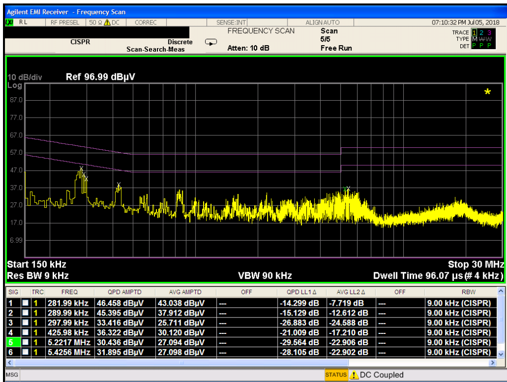
Plot 7-15. Line Conducted Plot (L1, S-Pen)
