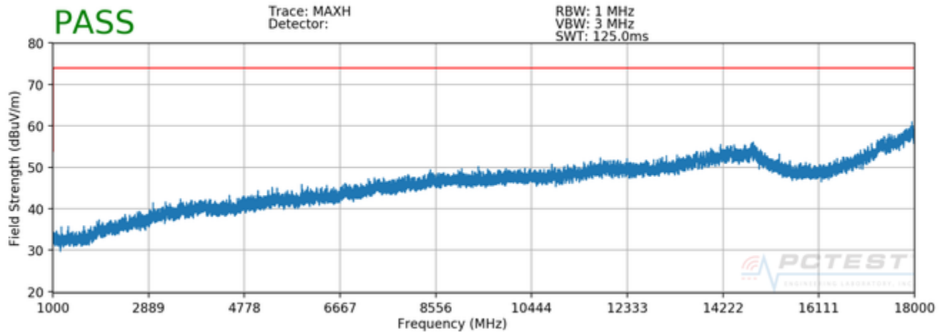
Plot 7-4. Radiated Spurious Plot above 1GHz (Charging Dock)
