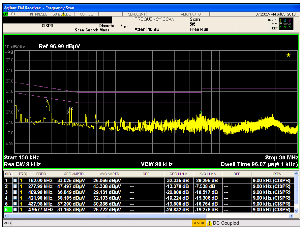
Plot 7-12. Line Conducted Plot (N, Charging Dock)
