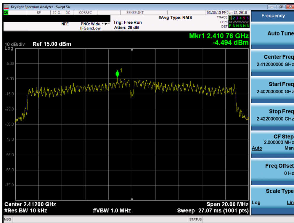
Plot 7-34. Power Spectral Density Plot SISO ANT2 (802.11n (2.4GHz) – Ch. 1)
