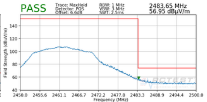
Plot 7-80. Radiated Restricted Upper Band Edge Measurement MIMO (Peak)
