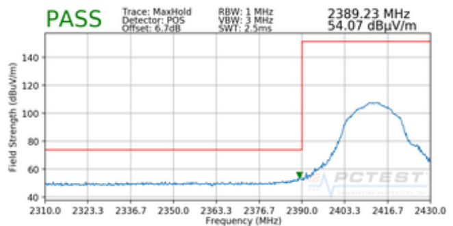
Plot 7-78. Radiated Restricted Lower Band Edge Measurement MIMO (Peak)
