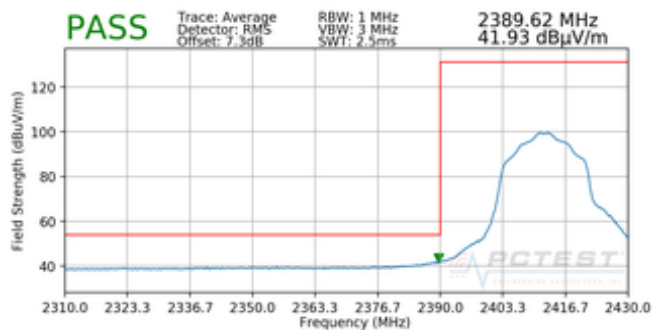
Plot 7-77. Radiated Restricted Lower Band Edge Measurement MIMO (Average)
