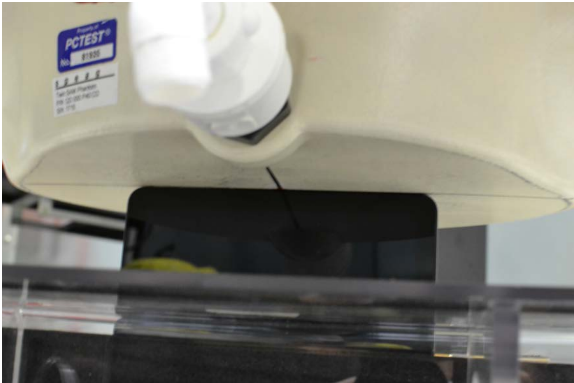
SAR Test Setup Photo 8 – Bottom Edge at 0.0 cm (Unlicensed Modes)
