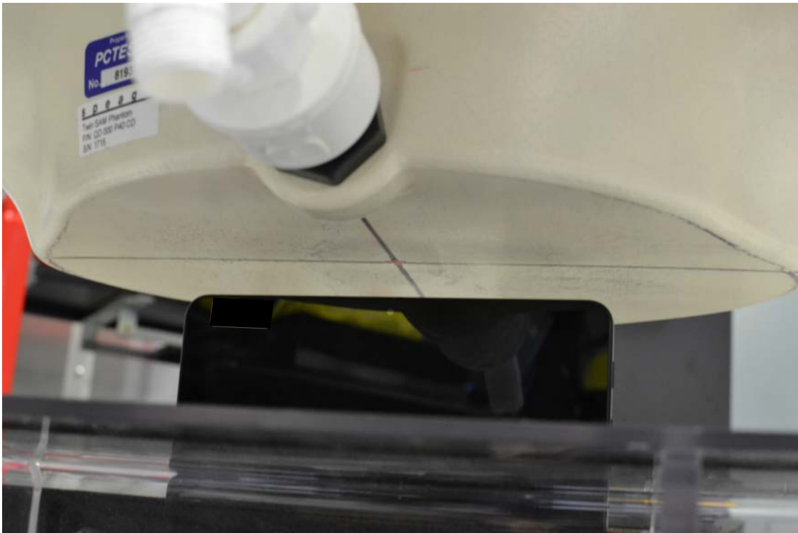
SAR Test Setup Photo 6 – Top Edge at 1.6 cm (Licensed Modes)
