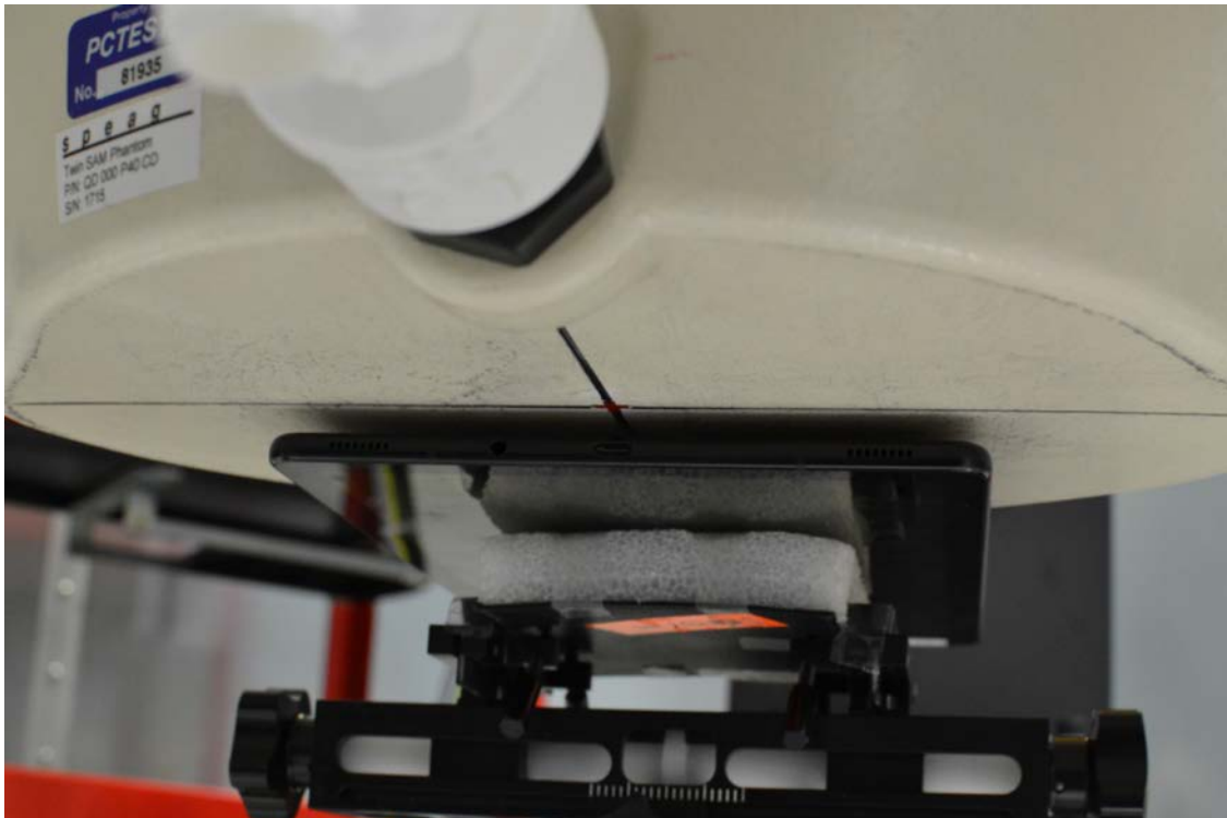
SAR Test Setup Photo 2 – Back Side at 0.5 cm (Unlicensed Modes)
