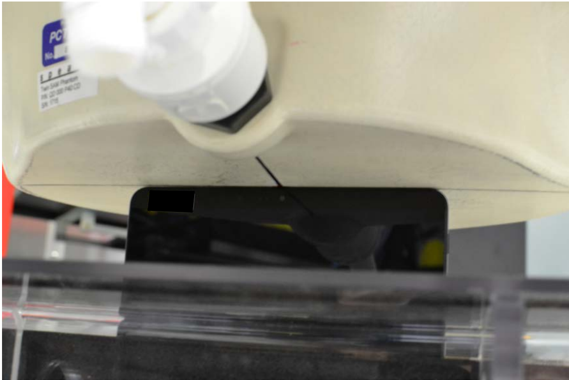
SAR Test Setup Photo 7 – Top Edge at 0.0 cm (Licensed and Unlicensed Modes)
