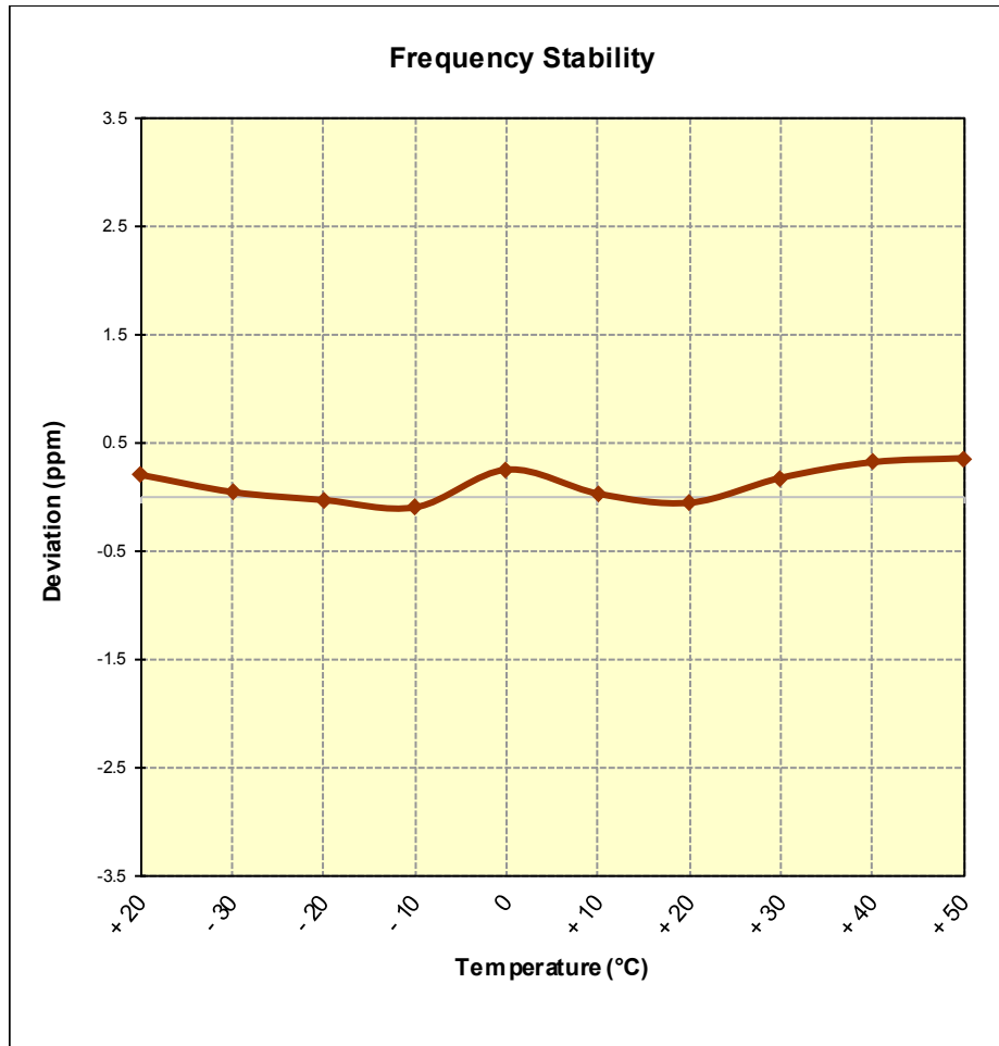
Figure 7-6. CDMA BC10 Frequency Stability Graph (CDMA, Ch. 476)
