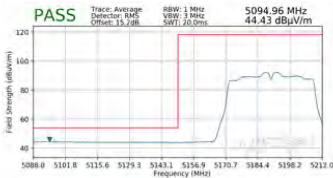
Plot 7-179. Radiated Lower Band Edge Plot (Average – UNII Band 1)
