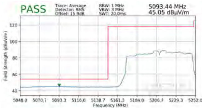
Plot 7-186. Radiated Lower Band Edge Plot (Average – UNII Band 1)
