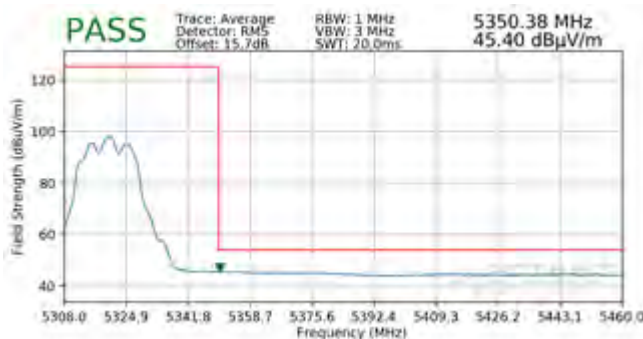
Plot 7-223. Radiated Upper Band Edge Plot (Average – UNII Band 2A)
