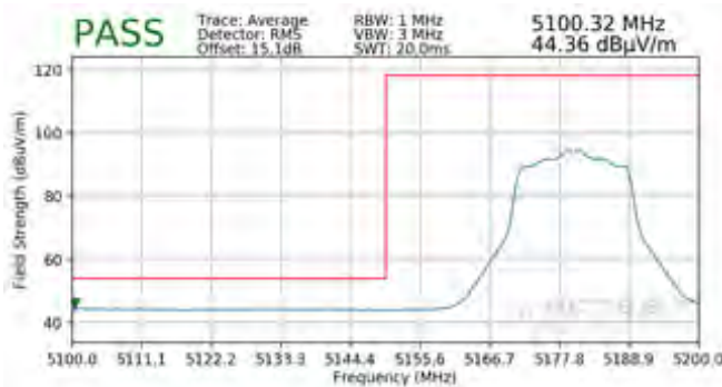
Plot 7-193. Radiated Lower Band Edge Plot (Average – UNII Band 1)
