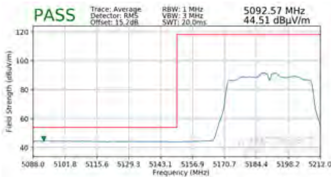
Plot 7-200. Radiated Lower Band Edge Plot (Average – UNII Band 1)
