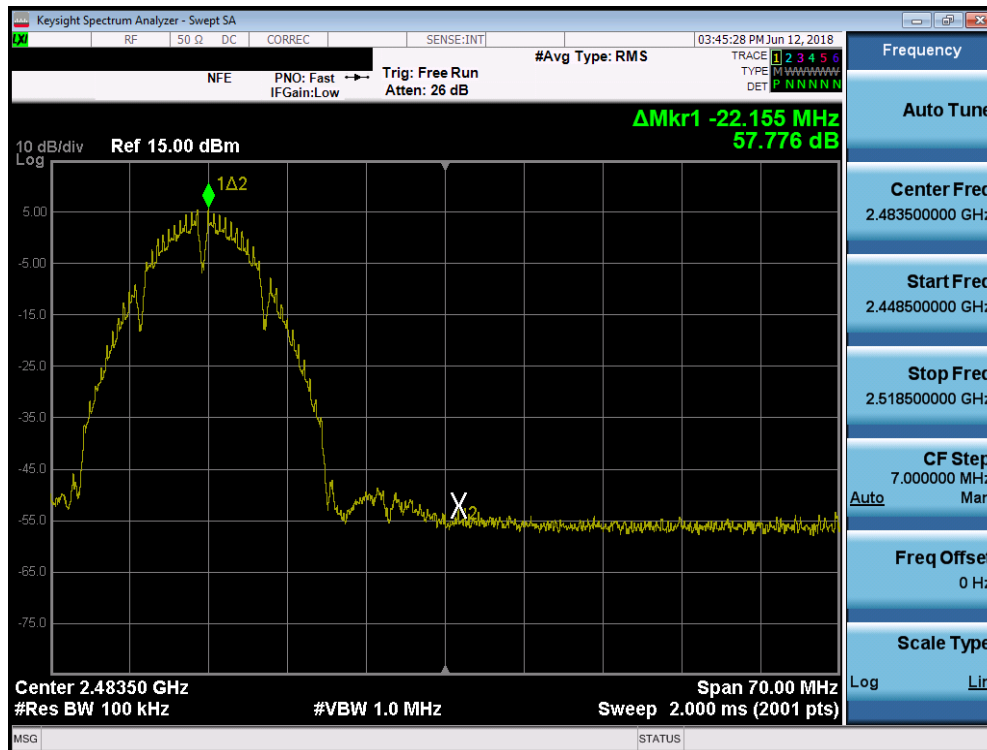
Plot 7-44. Band Edge Plot SISO ANT2 (802.11b – Ch. 11)
