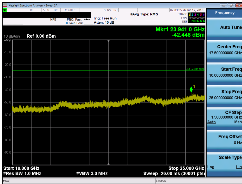
Plot 7-52. Conducted Spurious Plot SISO ANT1 (802.11b – Ch. 6)
