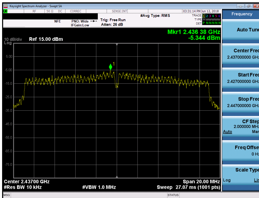
Plot 7-35. Power Spectral Density Plot SISO ANT2 (802.11n (2.4GHz) – Ch. 6)
