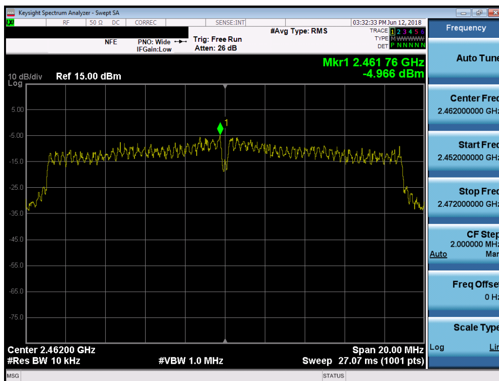
Plot 7-36. Power Spectral Density Plot SISO ANT2 (802.11n (2.4GHz) – Ch. 11)
