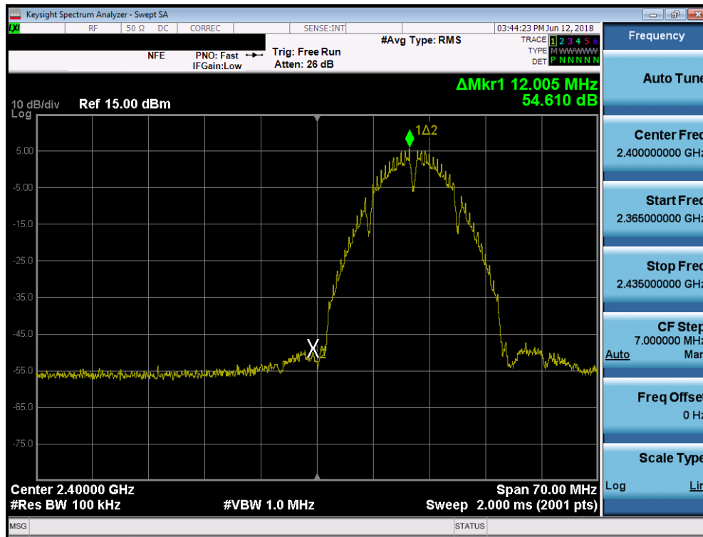
Plot 7-43. Band Edge Plot SISO ANT2 (802.11b – Ch. 1)
