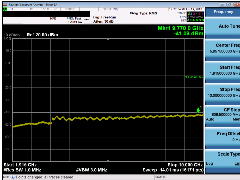
Plot 7-39. Conducted Spurious Plot (PCS CDMA Mode - High Channel)
