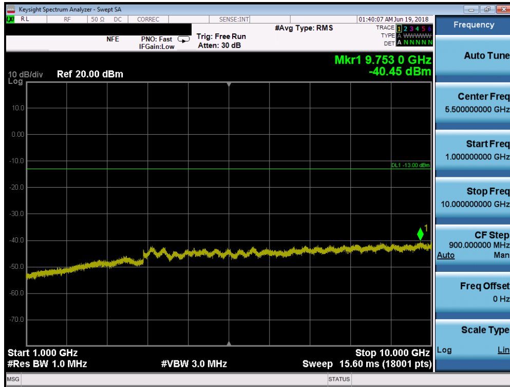
Plot 7-13. Conducted Spurious Plot (Cellular WCDMA Mode - High Channel)
