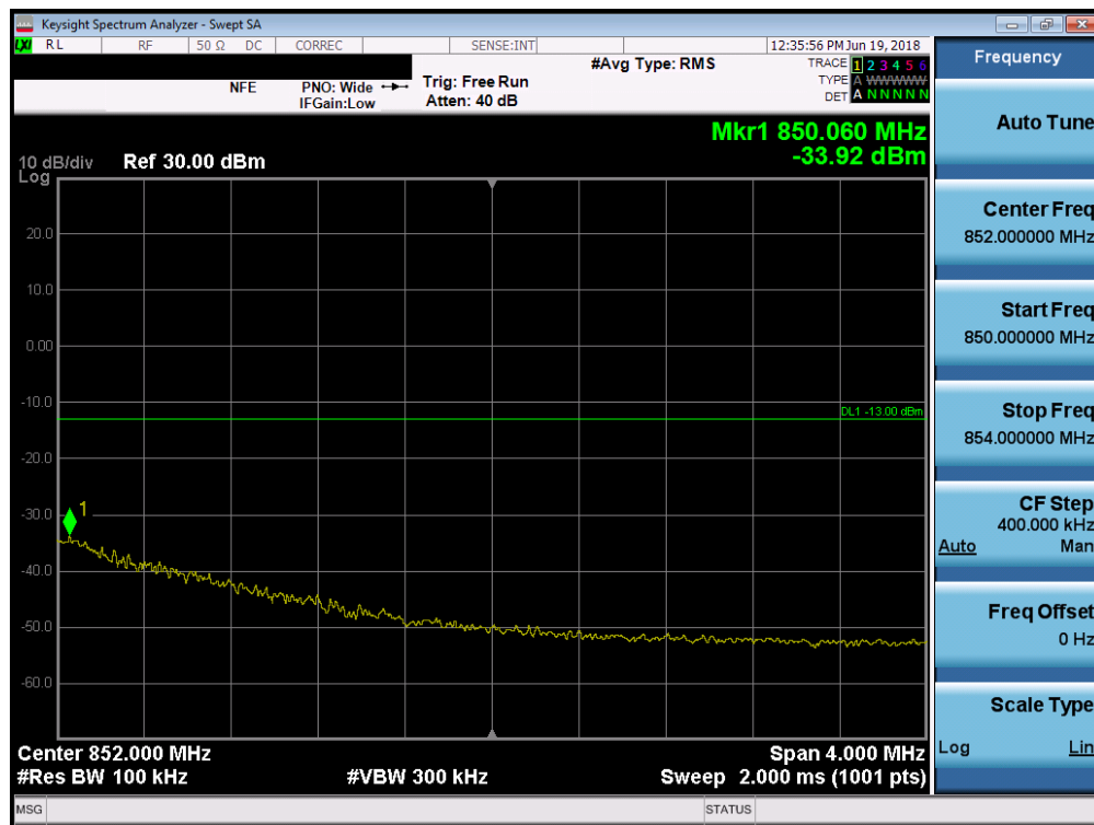
Plot 7-50. 4MHz Span Plot (Cellular CDMA Mode - High Channel)
