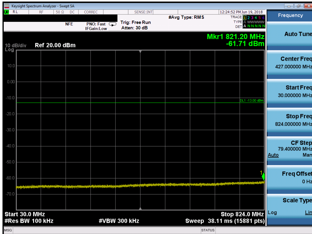
Plot 7-26. Conducted Spurious Plot (Cellular CDMA Mode - Mid Channel)
