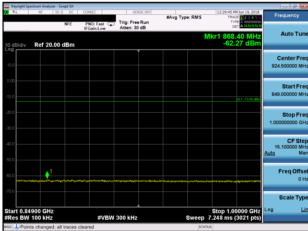
Plot 7-24. Conducted Spurious Plot (Cellular CDMA Mode - Low Channel)
