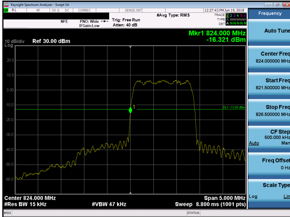
Plot 7-47. Band Edge Plot (Cellular CDMA Mode - Low Channel)
