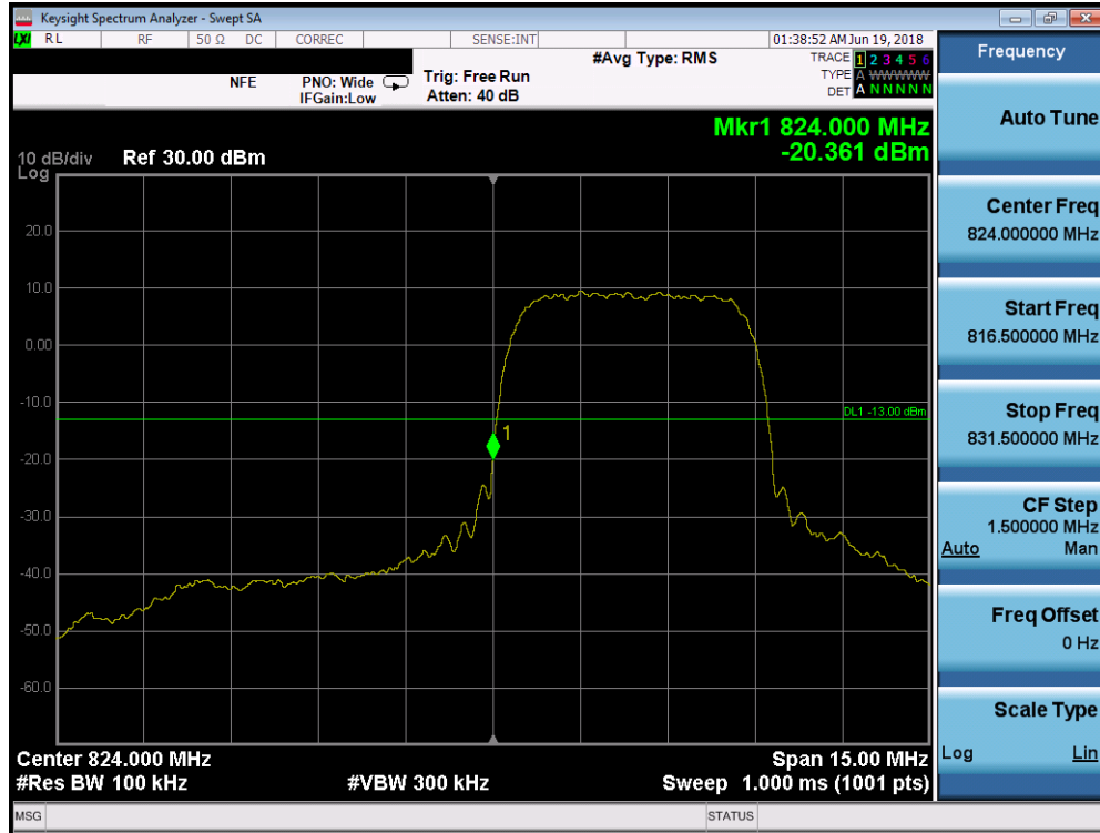
Plot 7-41. Band Edge Plot (Cellular WCDMA Mode - Low Channel)
