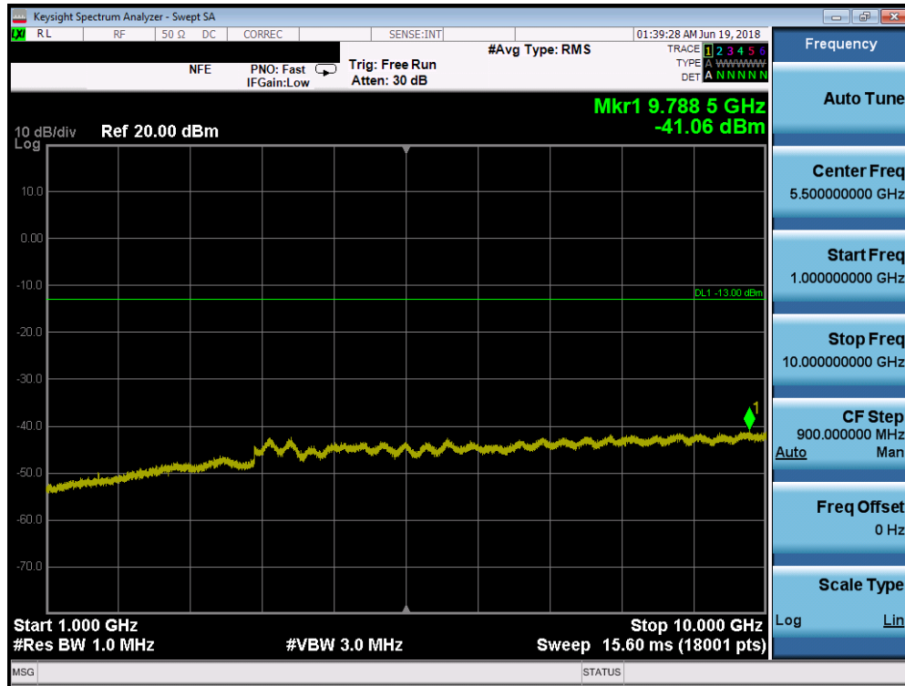
Plot 7-7. Conducted Spurious Plot (Cellular WCDMA Mode - Low Channel)
