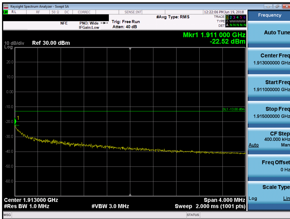
Plot 7-54. 4MHz Span Plot (PCS CDMA Mode - High Channel)
