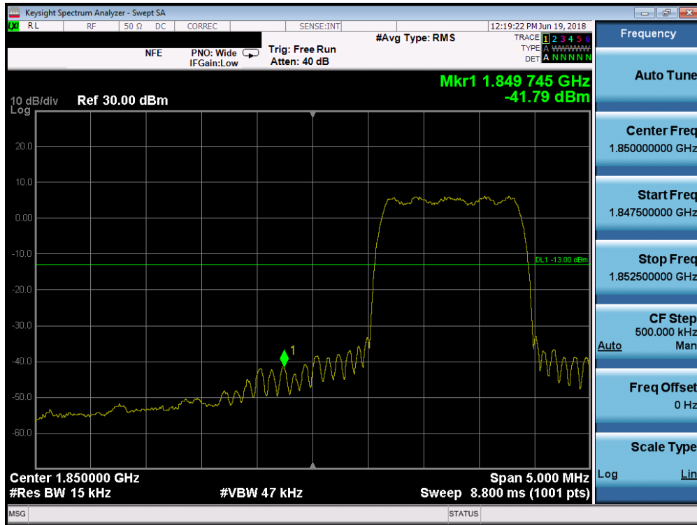
Plot 7-51. Band Edge Plot (PCS CDMA Mode - Low Channel)
