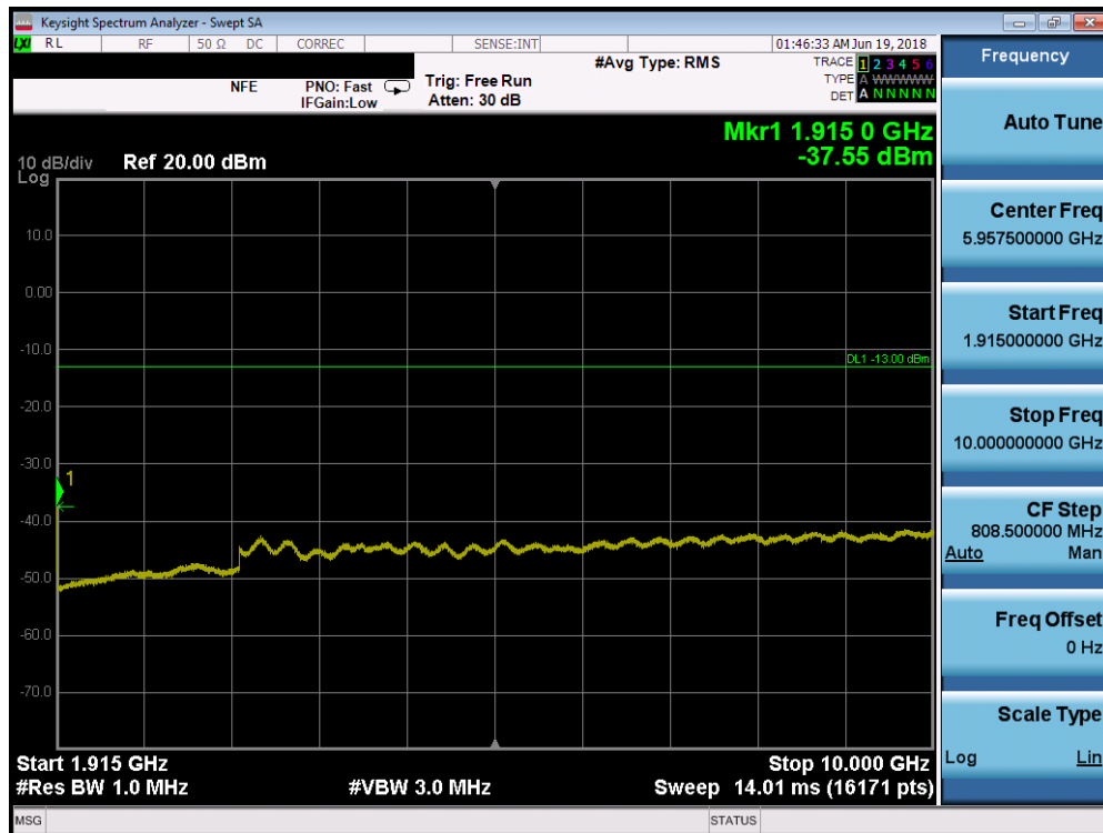
Plot 7-21. Conducted Spurious Plot (PCS WCDMA Mode - High Channel)
