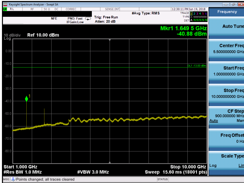
Plot 7-25. Conducted Spurious Plot (Cellular CDMA Mode - Low Channel)
