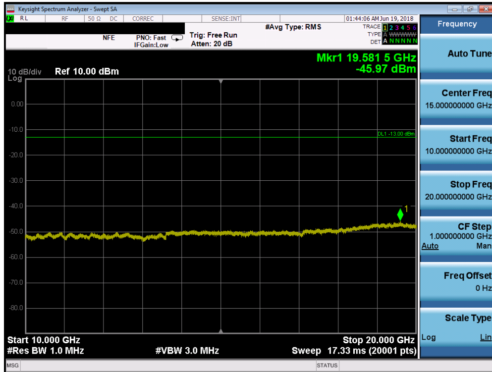
Plot 7-16. Conducted Spurious Plot (PCS WCDMA Mode - Low Channel)
