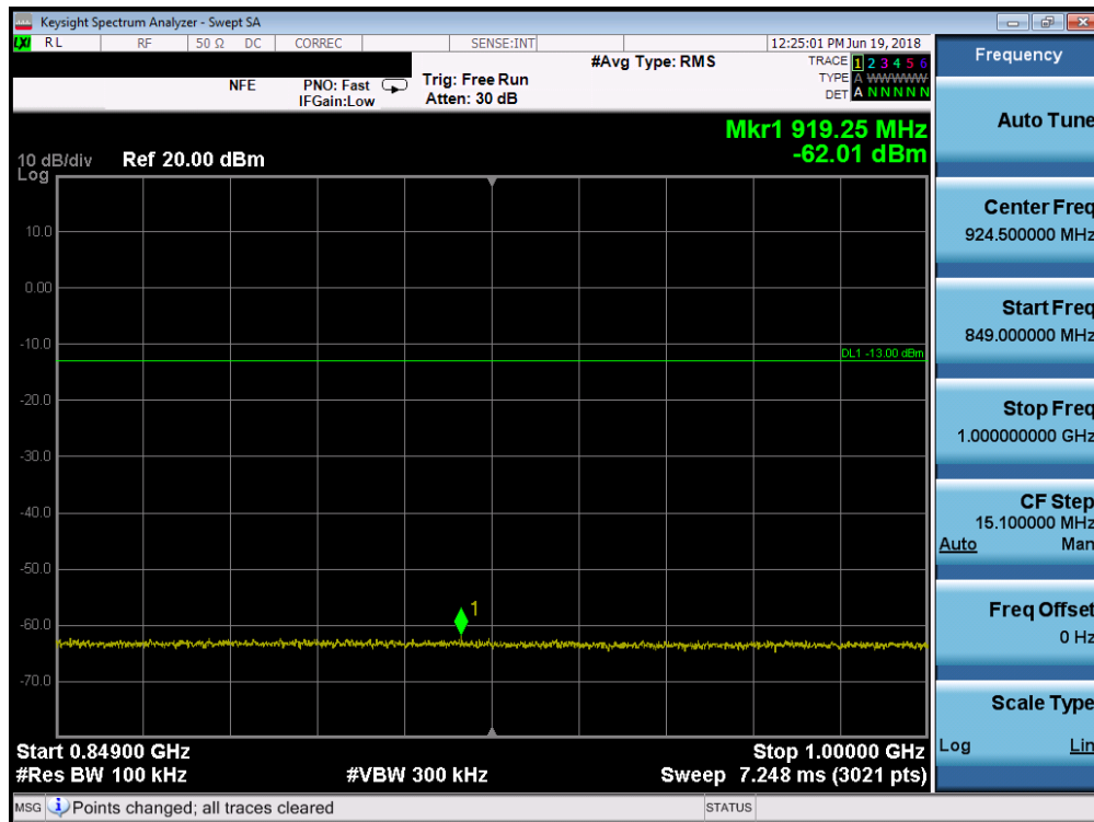
Plot 7-27. Conducted Spurious Plot (Cellular CDMA Mode - Mid Channel)
