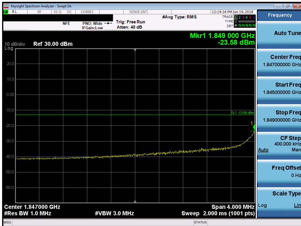
Plot 7-52. 4MHz Span Plot (PCS CDMA Mode - Low Channel)
