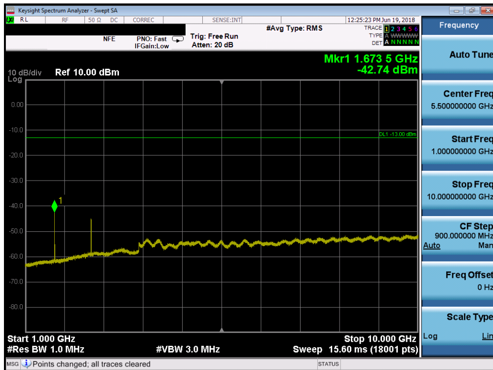
Plot 7-28. Conducted Spurious Plot (Cellular CDMA Mode - Mid Channel)
