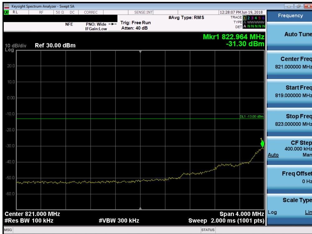
Plot 7-48. 4MHz Span Plot (Cellular CDMA Mode - Low Channel)
