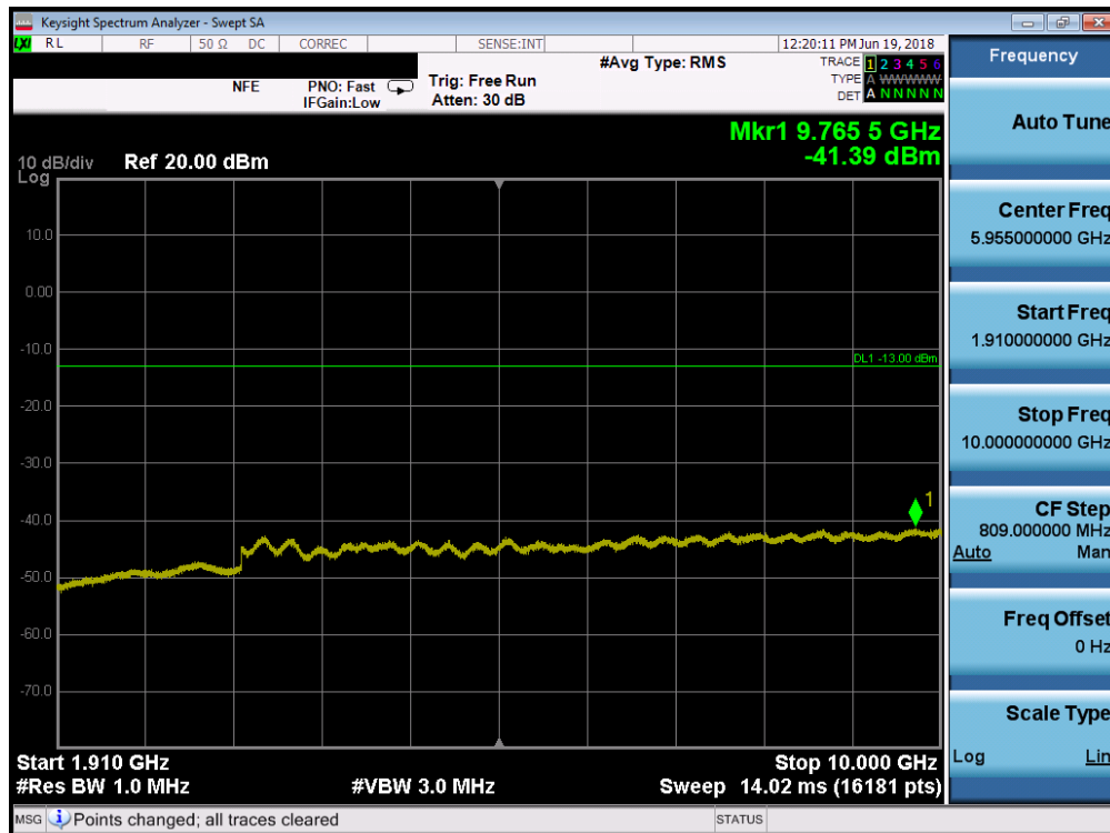
Plot 7-33. Conducted Spurious Plot (PCS CDMA Mode - Low Channel)
