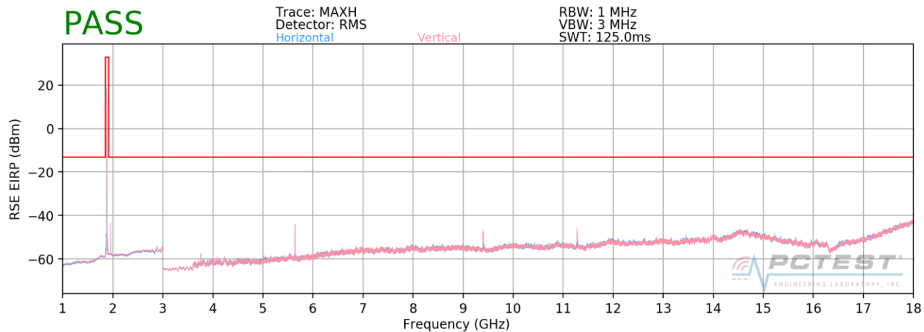
Plot 7-59. Radiated Spurious Plot (PCS WCDMA Mode)
