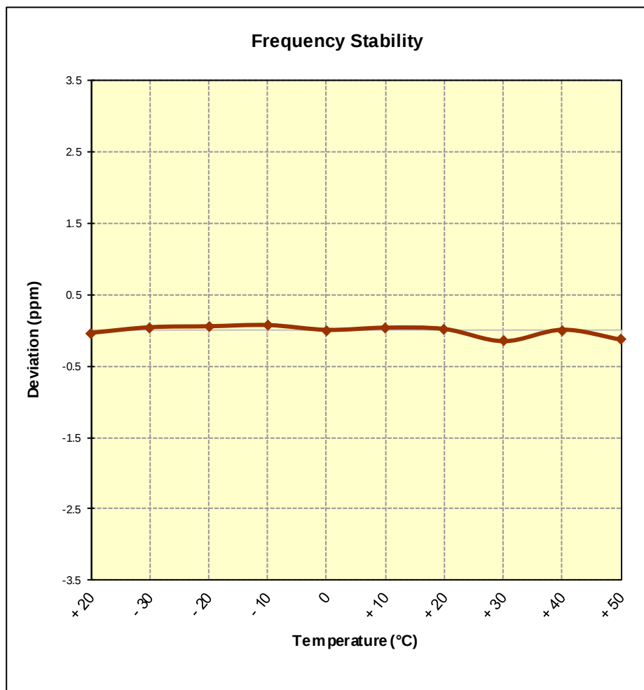
Figure 7-11. Frequency Stability Graph (PCS CDMA Mode – Ch. 600)
