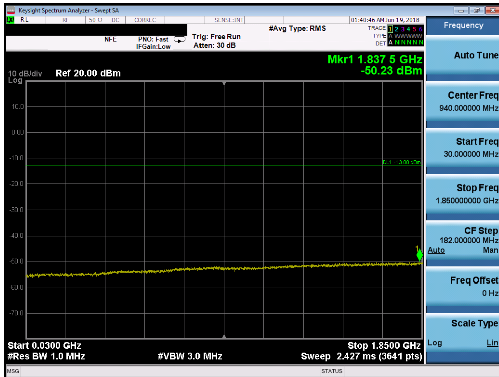
Plot 7-17. Conducted Spurious Plot (PCS WCDMA Mode - Mid Channel)
