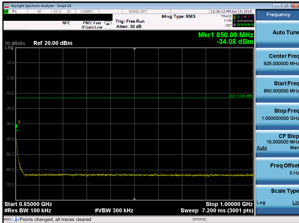
Plot 7-30. Conducted Spurious Plot (Cellular CDMA Mode - High Channel)
