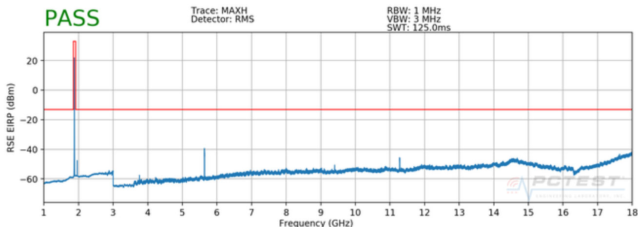
Plot 7-61. Radiated Spurious Plot (PCS CDMA Mode)
