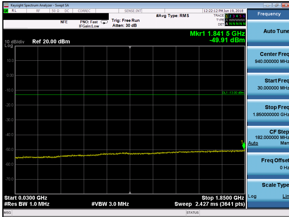
Plot 7-38. Conducted Spurious Plot (PCS CDMA Mode - High Channel)
