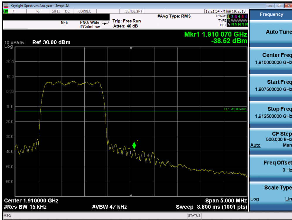
Plot 7-53. Band Edge Plot (PCS CDMA Mode - High Channel)
