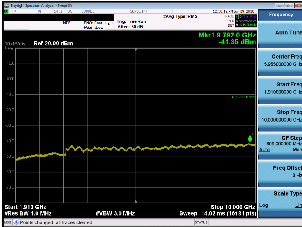
Plot 7-36. Conducted Spurious Plot (PCS CDMA Mode - Mid Channel)
