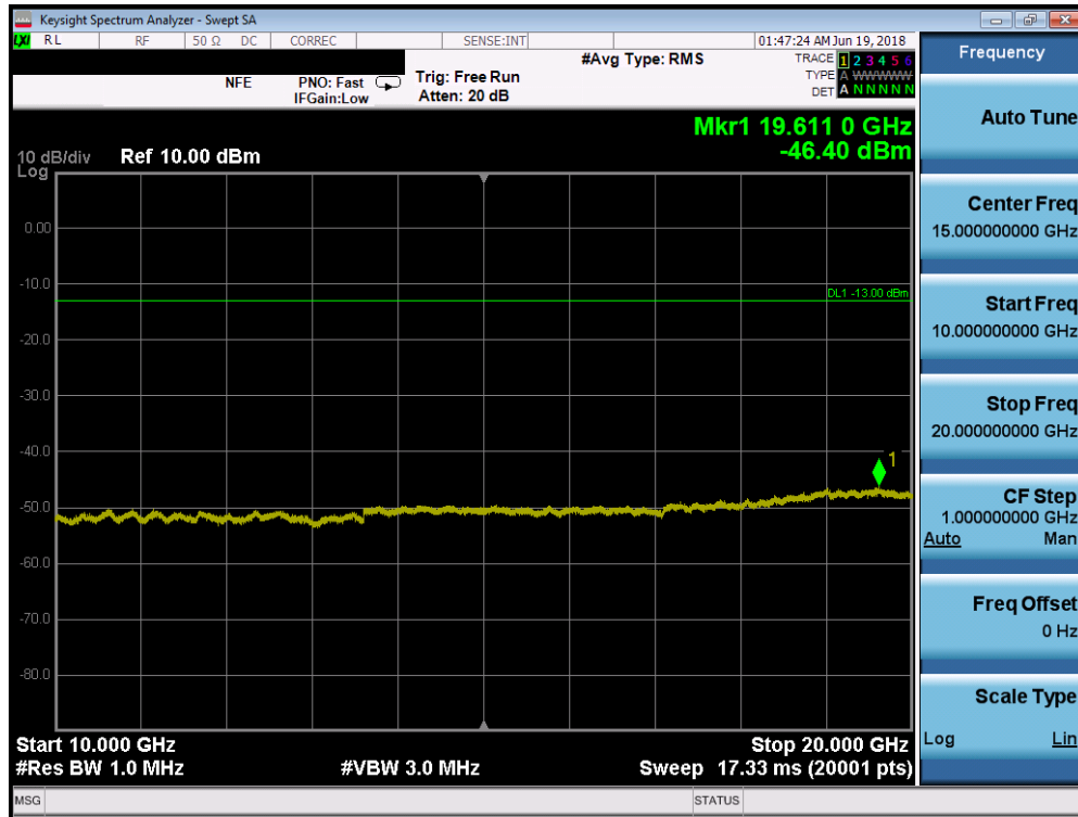
Plot 7-22. Conducted Spurious Plot (PCS WCDMA Mode - High Channel)
