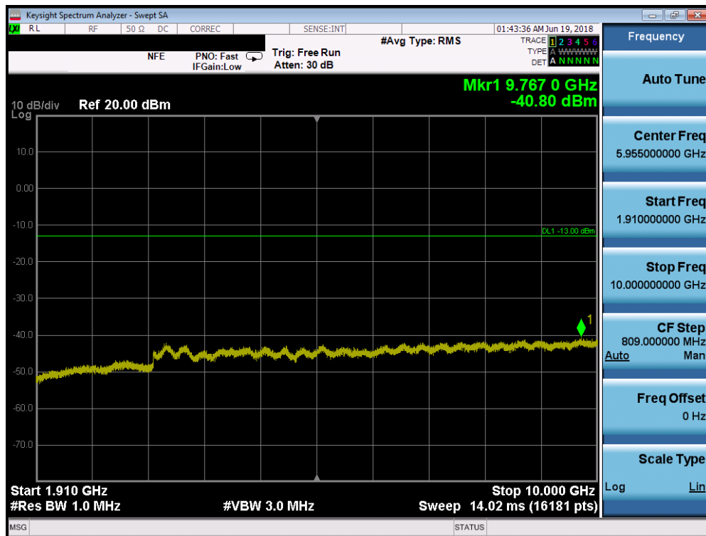
Plot 7-15. Conducted Spurious Plot (PCS WCDMA Mode - Low Channel)
