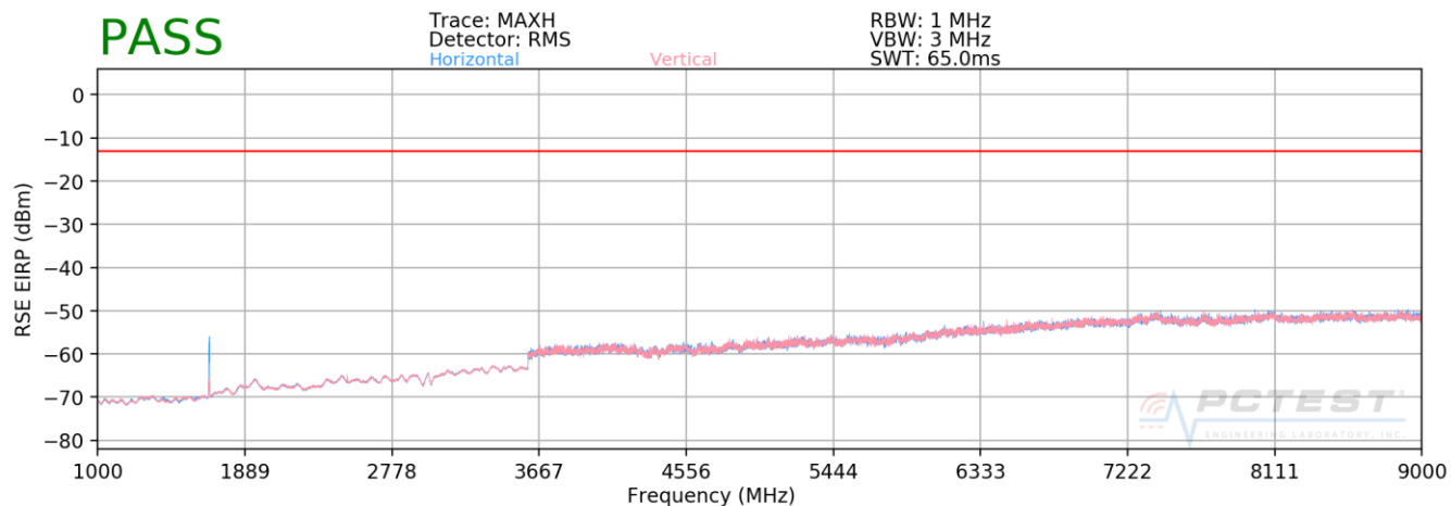
Plot 7-58. Radiated Spurious Plot (Cellular WCDMA Mode)
