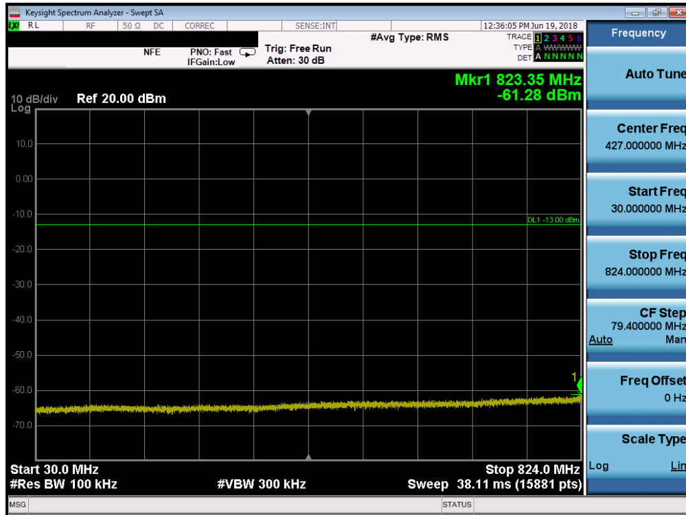
Plot 7-29. Conducted Spurious Plot (Cellular CDMA Mode - High Channel)
