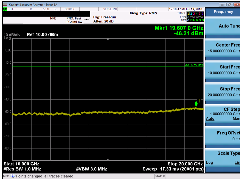
Plot 7-37. Conducted Spurious Plot (PCS CDMA Mode - Mid Channel)
