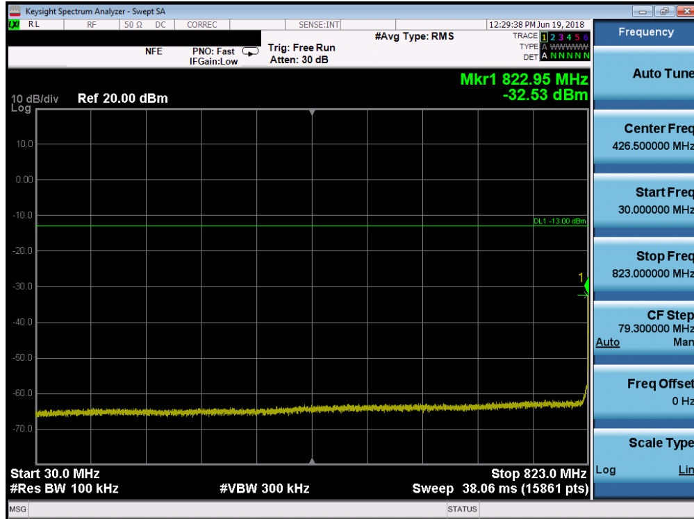
Plot 7-23. Conducted Spurious Plot (Cellular CDMA Mode - Low Channel)
