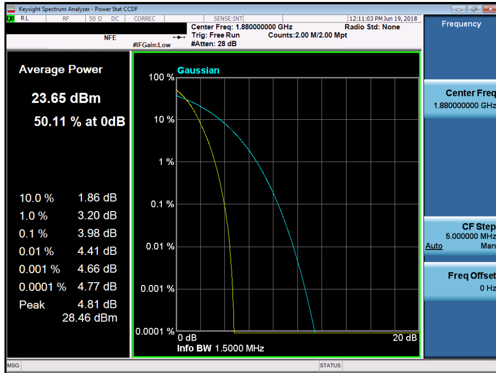
Plot 7-57. Peak-Average Ratio Plot (PCS CDMA Mode)
