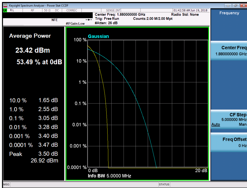
Plot 7-56. Peak-Average Ratio Plot (PCS WCDMA Mode)
