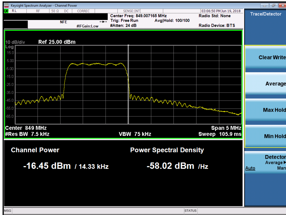
Plot 7-49. Band Edge Plot (Cellular CDMA Mode - High Channel)
