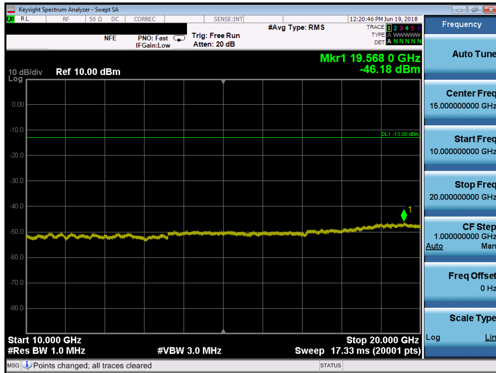
Plot 7-34. Conducted Spurious Plot (PCS CDMA Mode - Low Channel)
