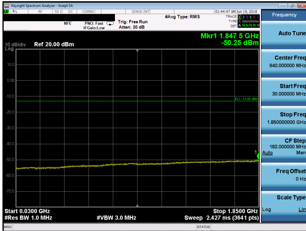
Plot 7-20. Conducted Spurious Plot (PCS WCDMA Mode - High Channel)
