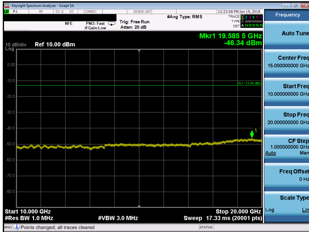
Plot 7-40. Conducted Spurious Plot (PCS CDMA Mode - High Channel)
