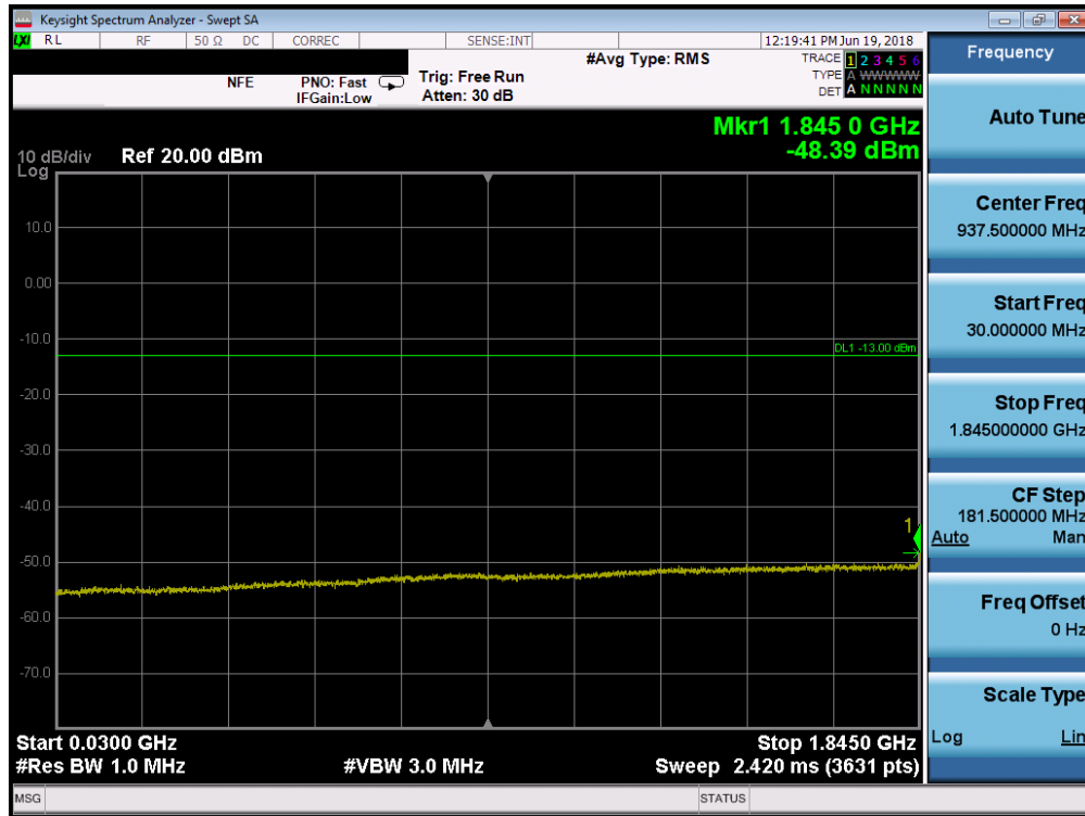
Plot 7-32. Conducted Spurious Plot (PCS CDMA Mode - Low Channel)
