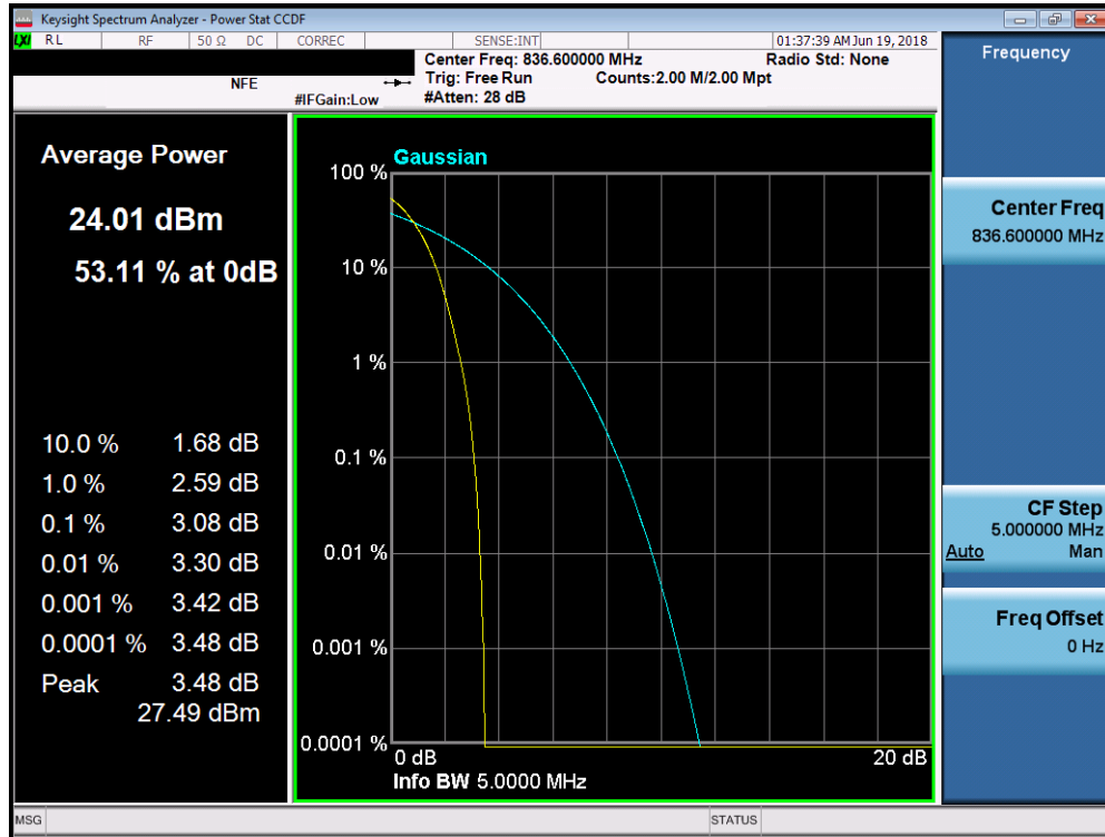
Plot 7-55. Peak-Average Ratio Plot (CELL WCDMA Mode)
