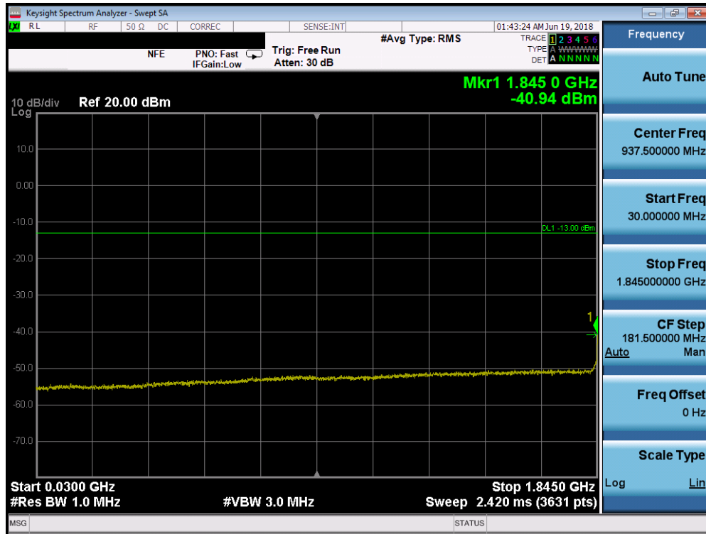
Plot 7-14. Conducted Spurious Plot (PCS WCDMA Mode - Low Channel)
