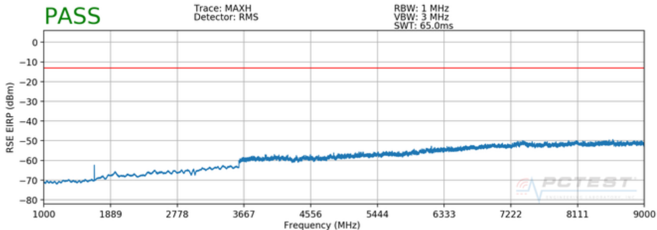
Plot 7-60. Radiated Spurious Plot (Cellular CDMA Mode)
