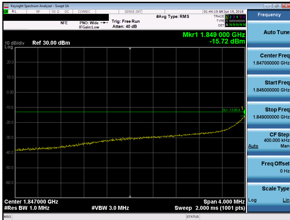
Plot 7-44. 4MHz Span Plot (PCS WCDMA Mode - Low Channel)
