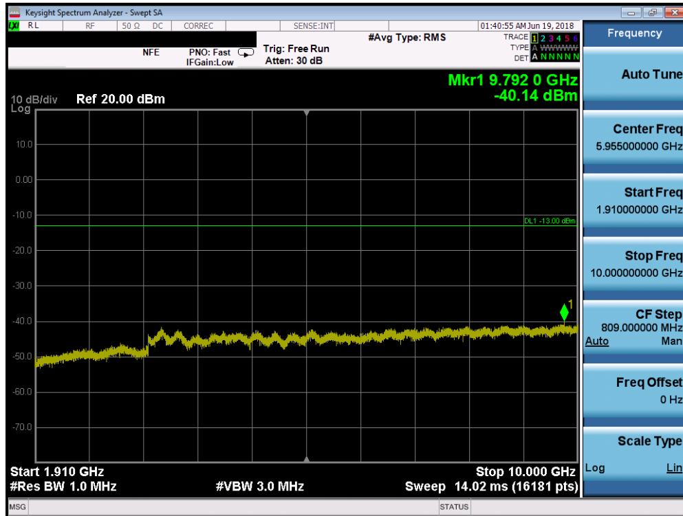
Plot 7-18. Conducted Spurious Plot (PCS WCDMA Mode - Mid Channel)
