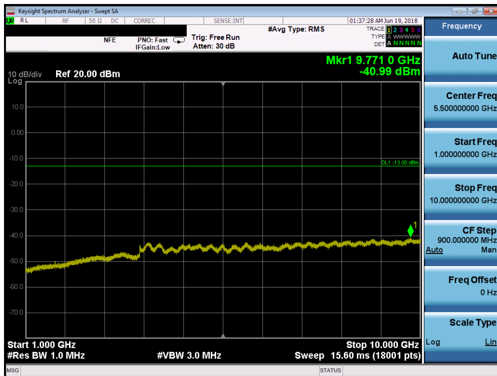
Plot 7-10. Conducted Spurious Plot (Cellular WCDMA Mode - Mid Channel)
