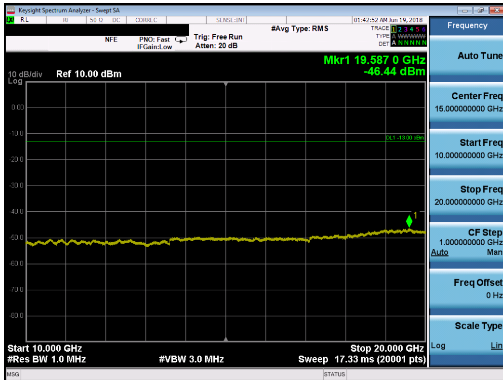
Plot 7-19. Conducted Spurious Plot (PCS WCDMA Mode - Mid Channel)
