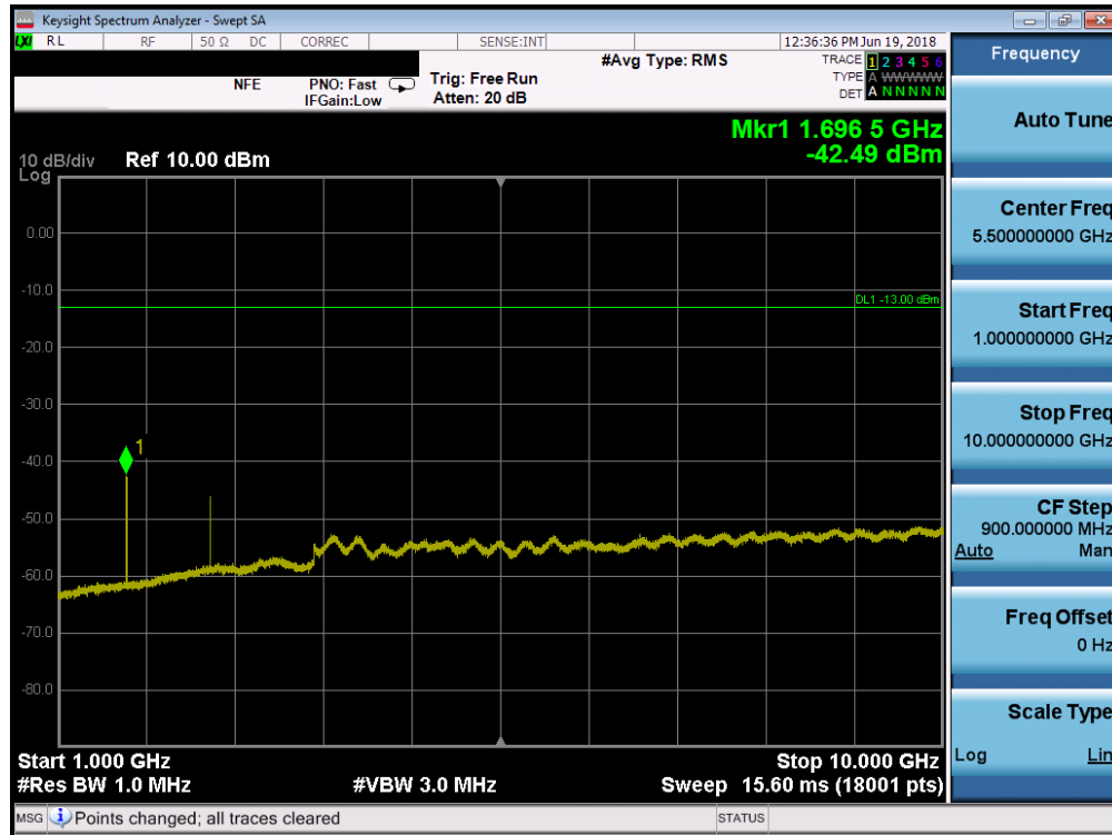
Plot 7-31. Conducted Spurious Plot (Cellular CDMA Mode - High Channel)
