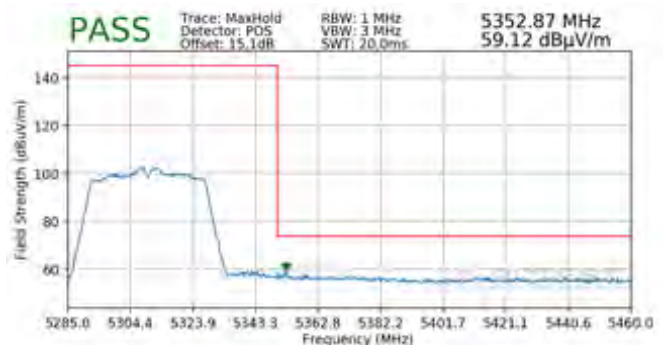
Plot 7-203. Radiated Upper Band Edge Plot (Peak – UNII Band 2A)
