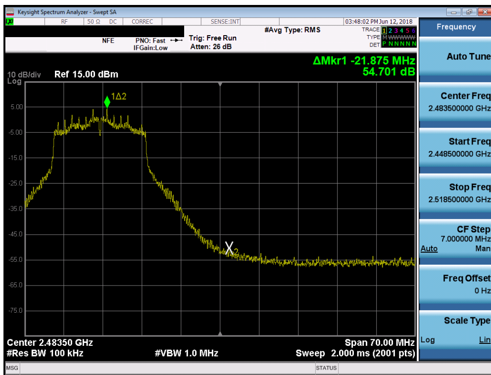
Plot 7-46. Band Edge Plot SISO ANT2 (802.11g - Ch. 11)
