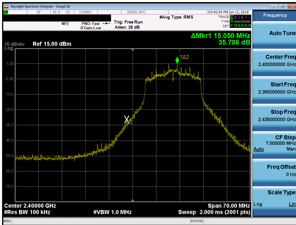
Plot 7-45. Band Edge Plot SISO ANT2 (802.11g- Ch. 1)
