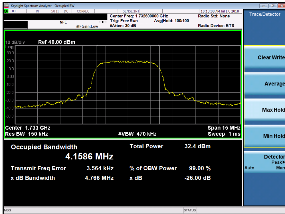
Plot 7-3. Occupied Bandwidth Plot (AWS WCDMA Mode)
