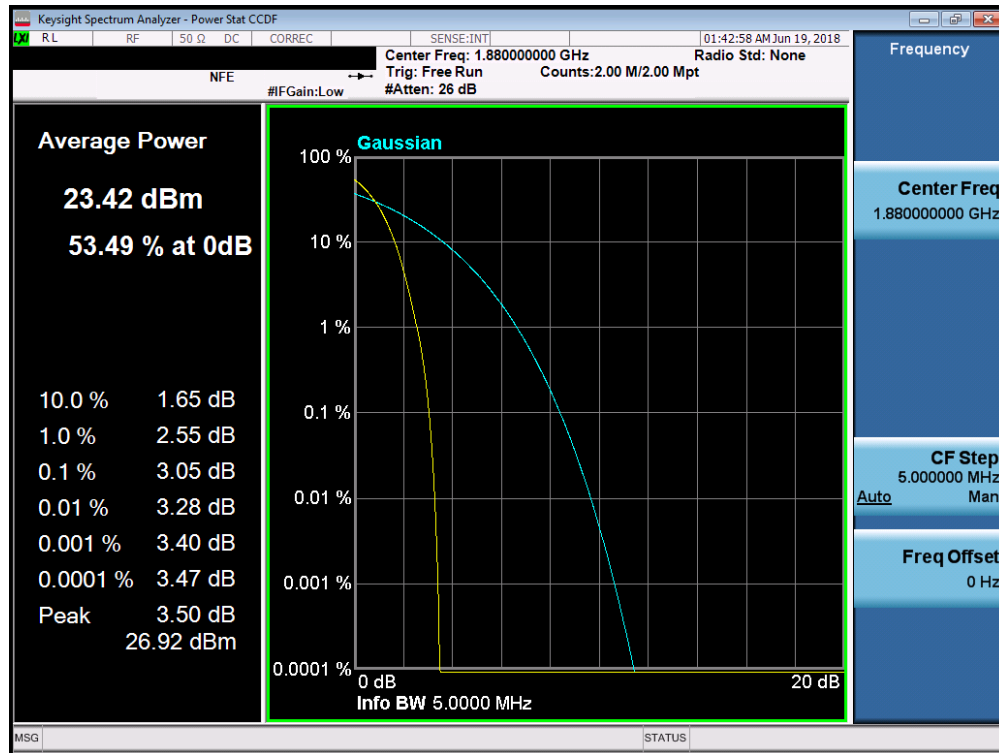
Plot 7-41. Peak-Average Ratio Plot (PCS WCDMA Mode)
