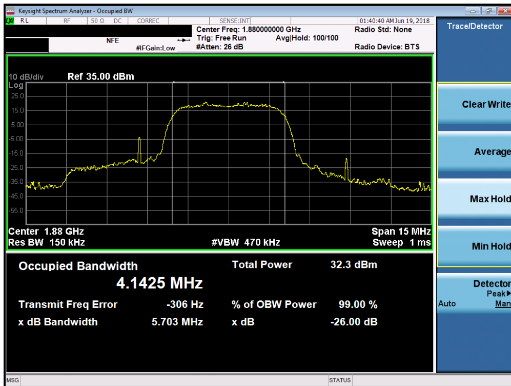
Plot 7-2. Occupied Bandwidth Plot (PCS WCDMA Mode)
