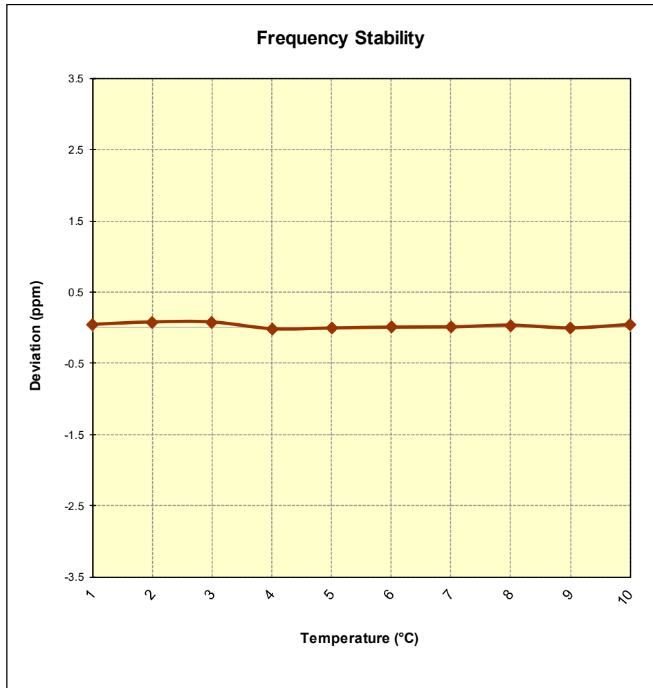
Figure 7-10. Frequency Stability Graph (PCS WCDMA Mode – Ch. 9400)
