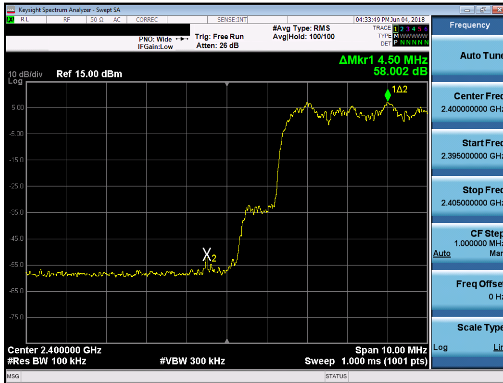
Plot 7-30. Band Edge Plot (Bluetooth with Hopping Enabled, 3 Mbps)
