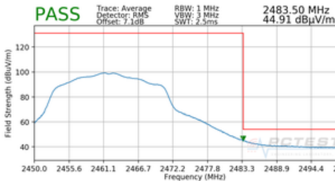
Plot 7-79. Radiated Restricted Upper Band Edge Measurement MIMO (Average)
