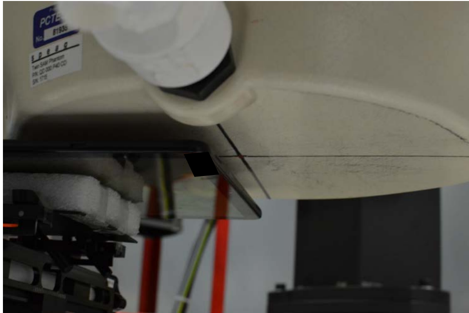
SAR Test Setup Photo 1 – Back Side at 1.6 cm (Licensed Modes)
