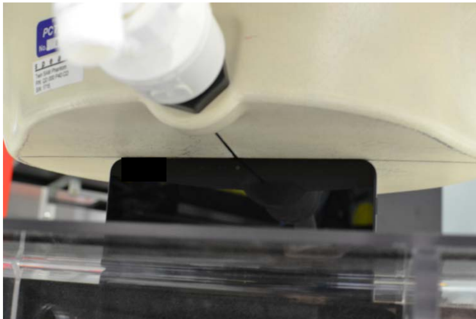
SAR Test Setup Photo 8 – Top Edge at 0.0 cm (Licensed and Unlicensed Modes)
