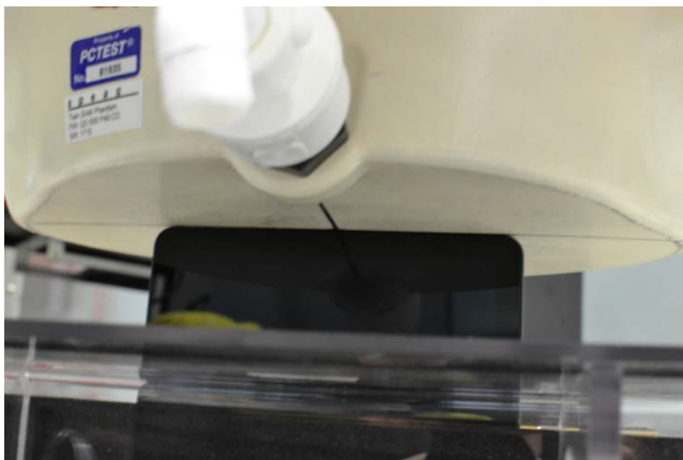
SAR Test Setup Photo 9 – Bottom Edge at 0.0 cm, (Unlicensed Modes)
