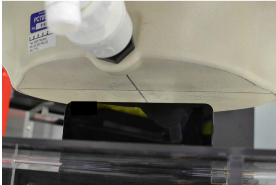
SAR Test Setup Photo 7 – Top Edge at 1.6 cm (Licensed Modes)
