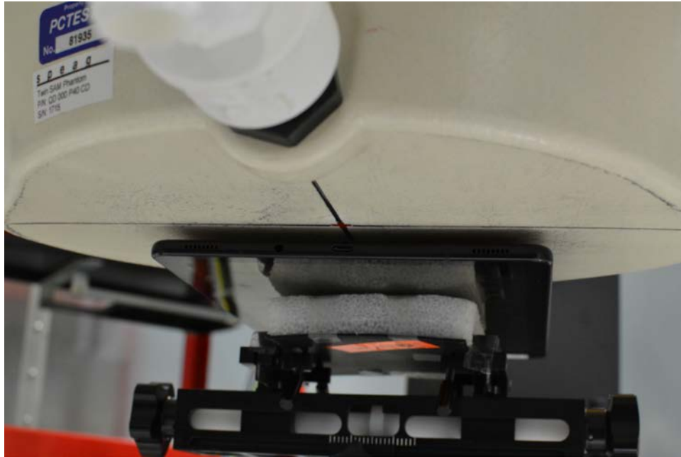
SAR Test Setup Photo 3 – Back Side at 0.5 cm (5GHz WLAN)
