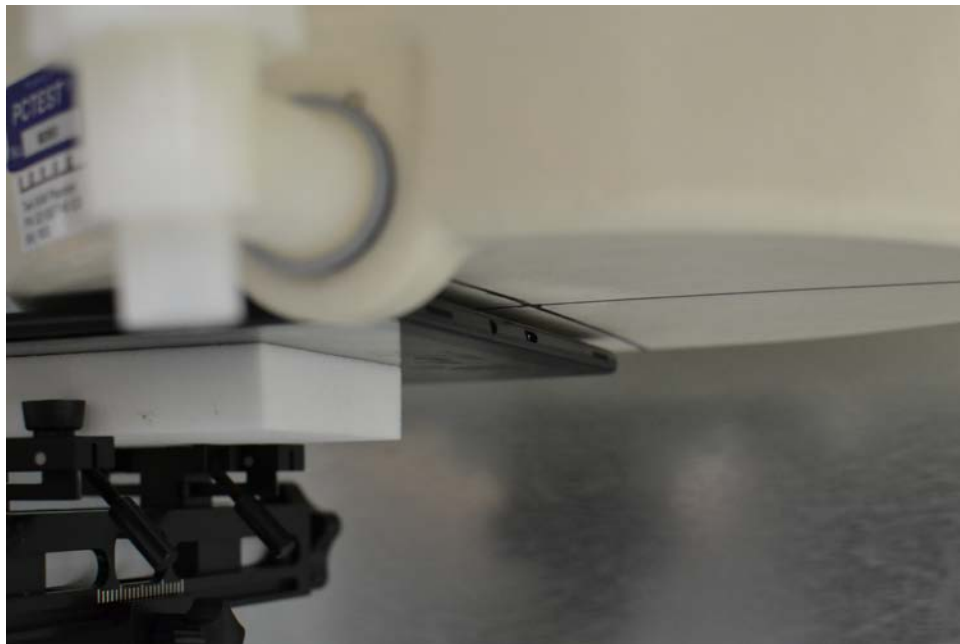
SAR Test Setup Photo 2 – Back Side at 0.5 cm (2.4GHz WLAN)
