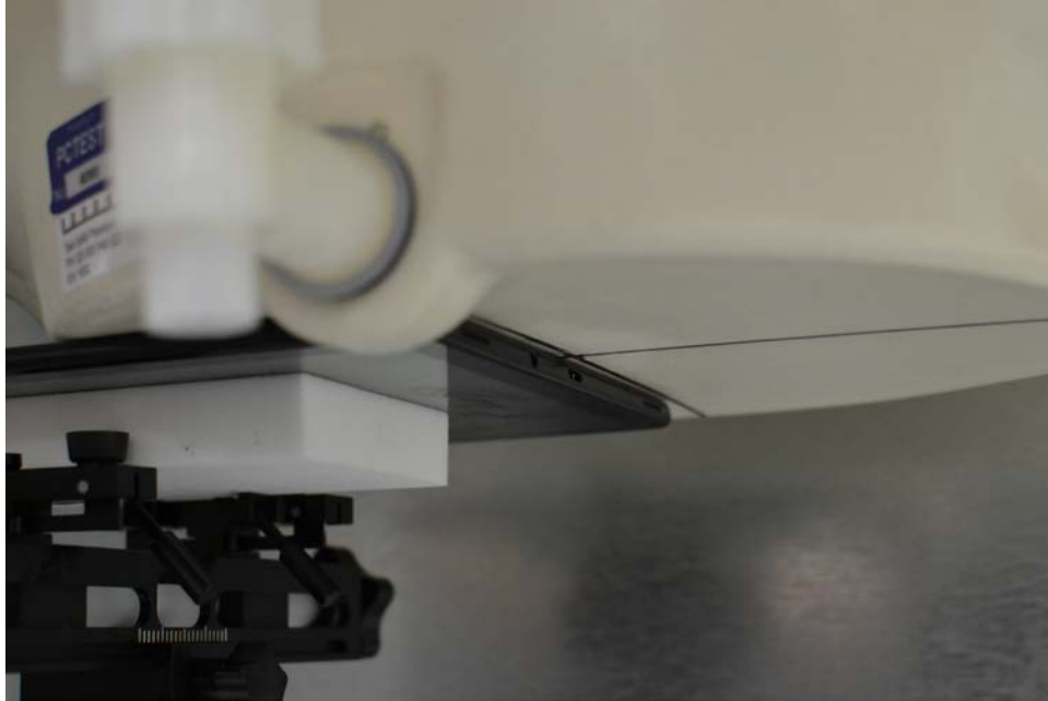
SAR Test Setup Photo 5 – Back Side at 0.0 cm (2.4GHz WLAN/BT)
