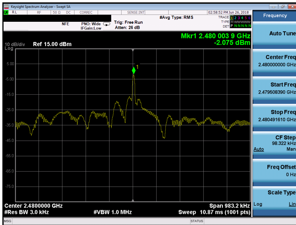
Plot 7-18. Power Spectral Density Plot (Bluetooth (LE), 2Mbps – Ch. 39)
