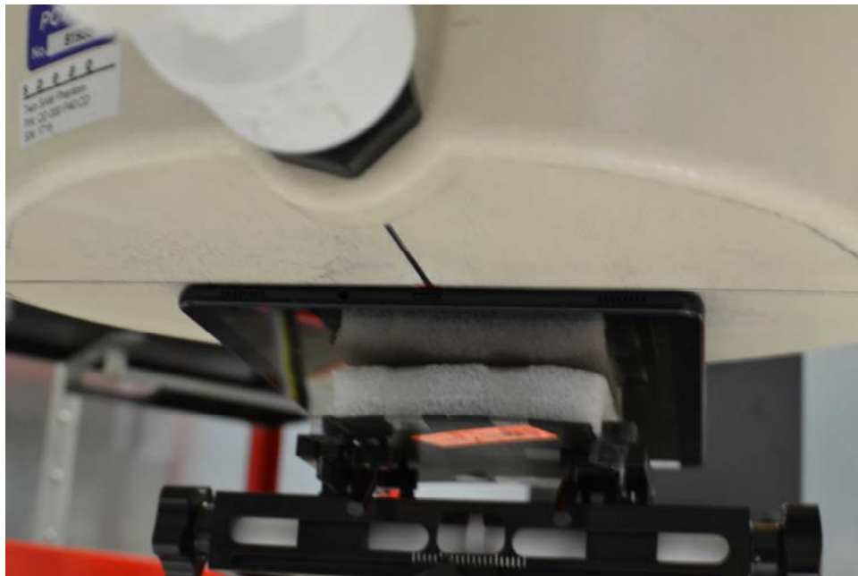
SAR Test Setup Photo 4 – Back Side at 0.0 cm (Unlicensed Modes)
