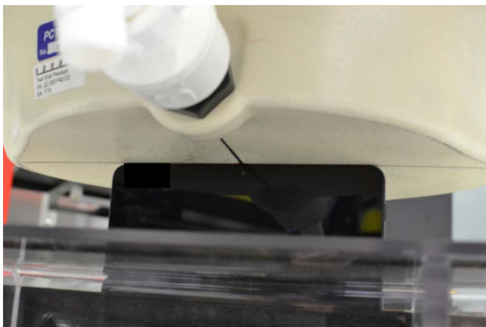
SAR Test Setup Photo 6 – Top Edge at 0.0 cm (Licensed and Unlicensed Modes)
