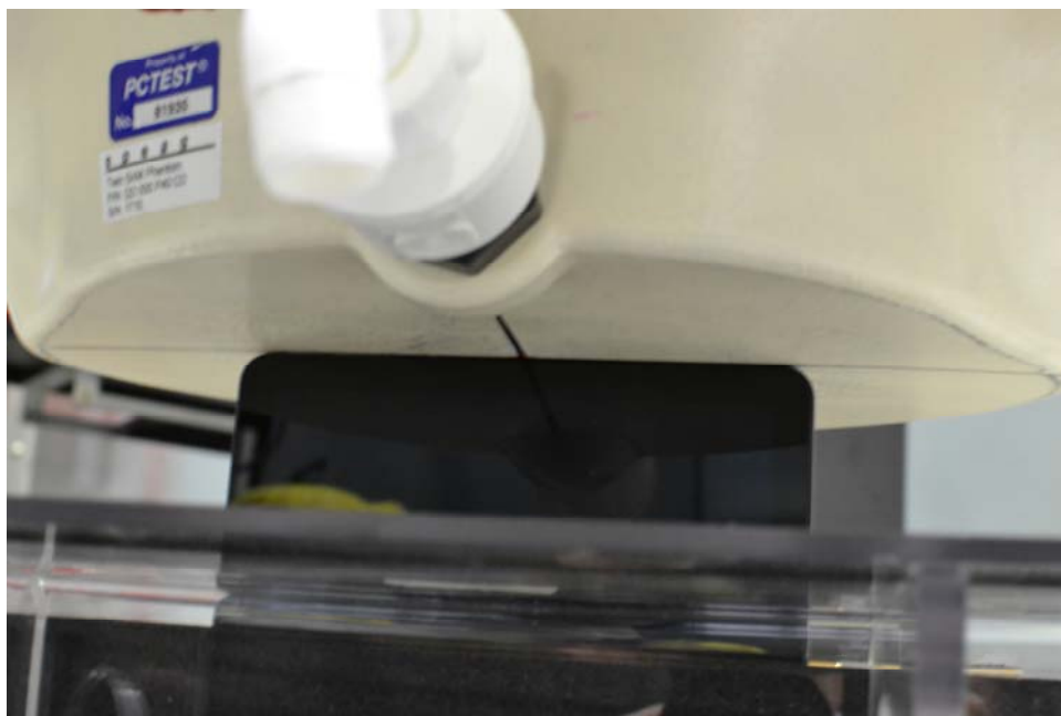
SAR Test Setup Photo 7 – Bottom Edge at 0.0 cm, (Unlicensed Modes)
