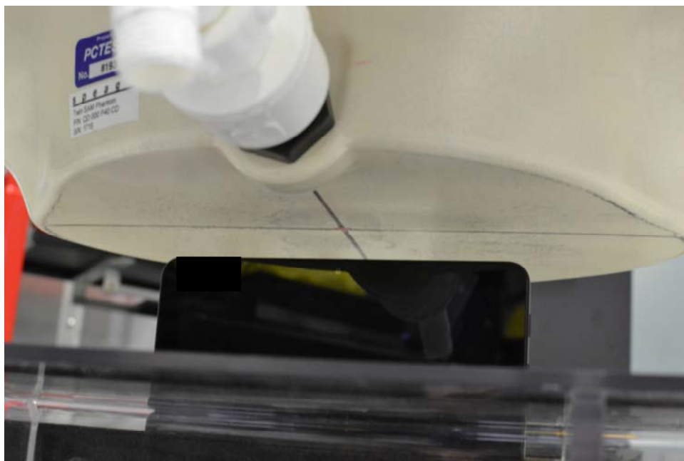
SAR Test Setup Photo 5 – Top Edge at 1.6 cm (Licensed Modes)
