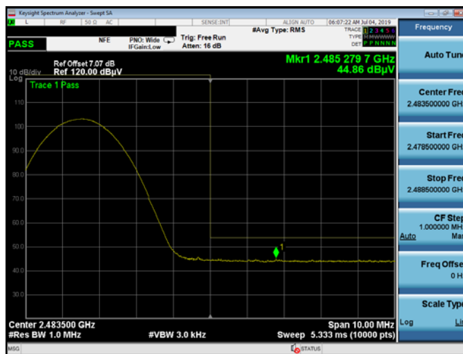
Plot 7-45. Radiated Restricted Upper Band Edge Measurement (Average)
