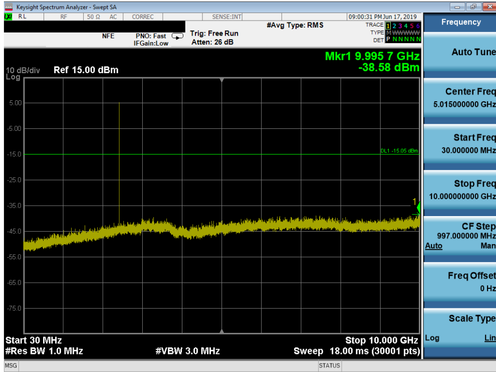
Plot 7-41. Conducted Spurious Plot (Bluetooth (LE), 2Mbps – Ch. 19)
