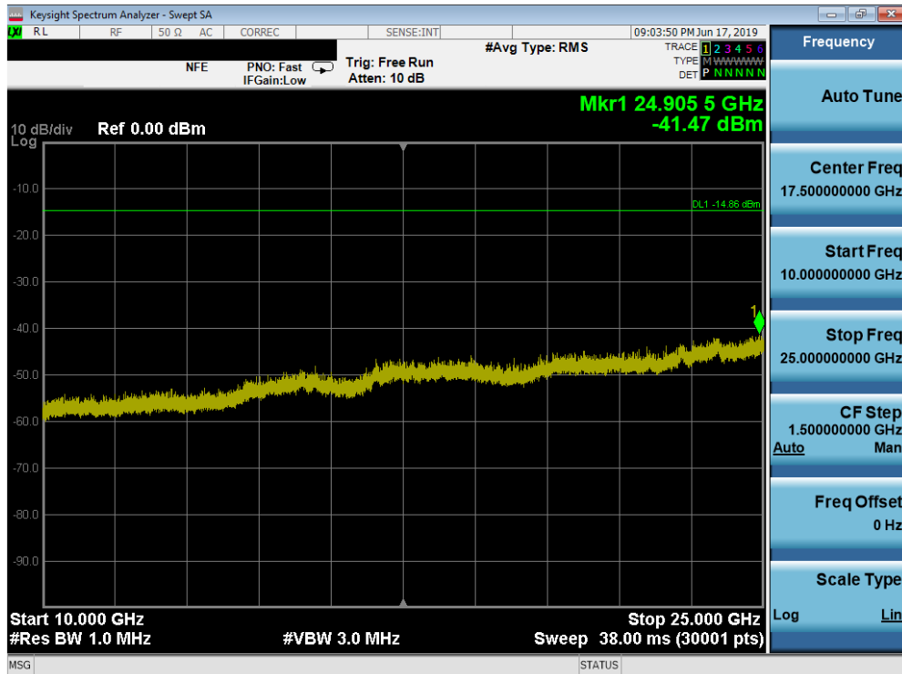
Plot 7-44. Conducted Spurious Plot (Bluetooth (LE), 2Mbps – Ch. 39)
