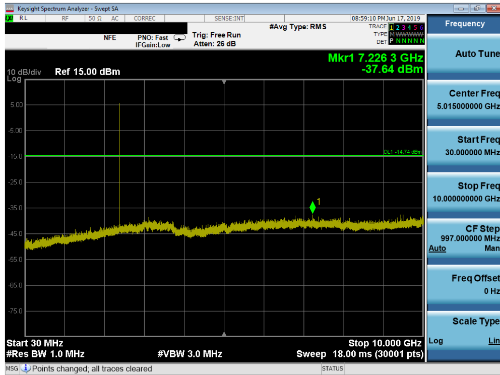
Plot 7-39. Conducted Spurious Plot (Bluetooth (LE), 2Mbps – Ch. 0)
