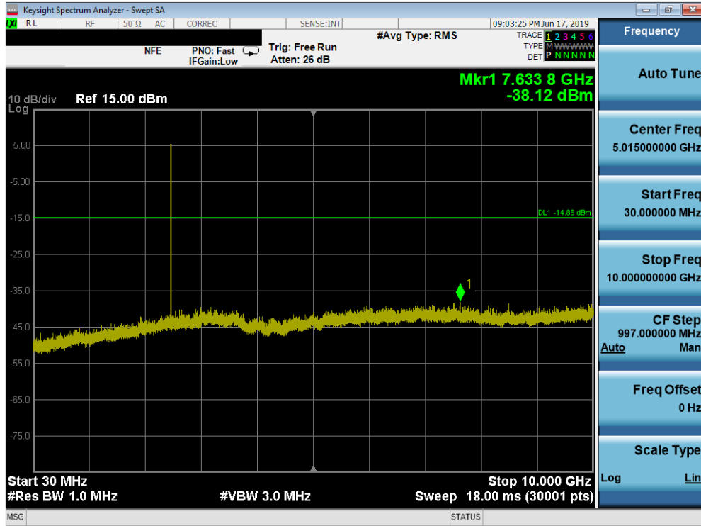
Plot 7-43. Conducted Spurious Plot (Bluetooth (LE), 2Mbps – Ch. 39)
