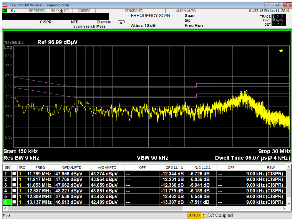
Plot 7-47. Line Conducted Plot with Bluetooth LE (L1)
