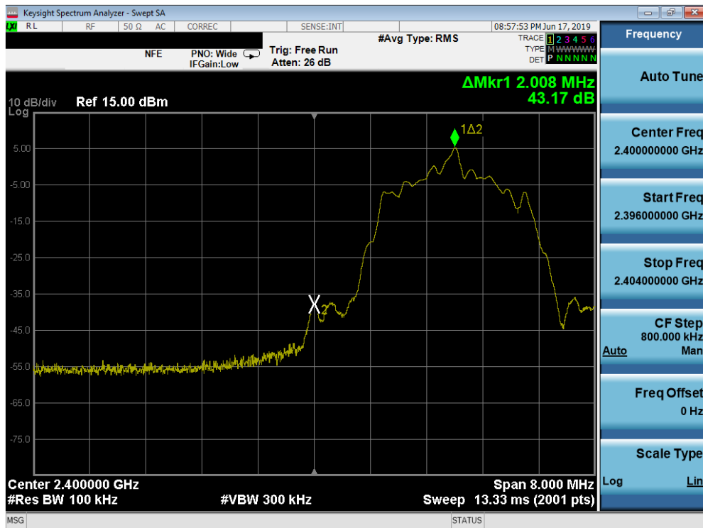
Plot 7-37. Band Edge Plot (Bluetooth (LE), 2Mbps – Ch. 0)
