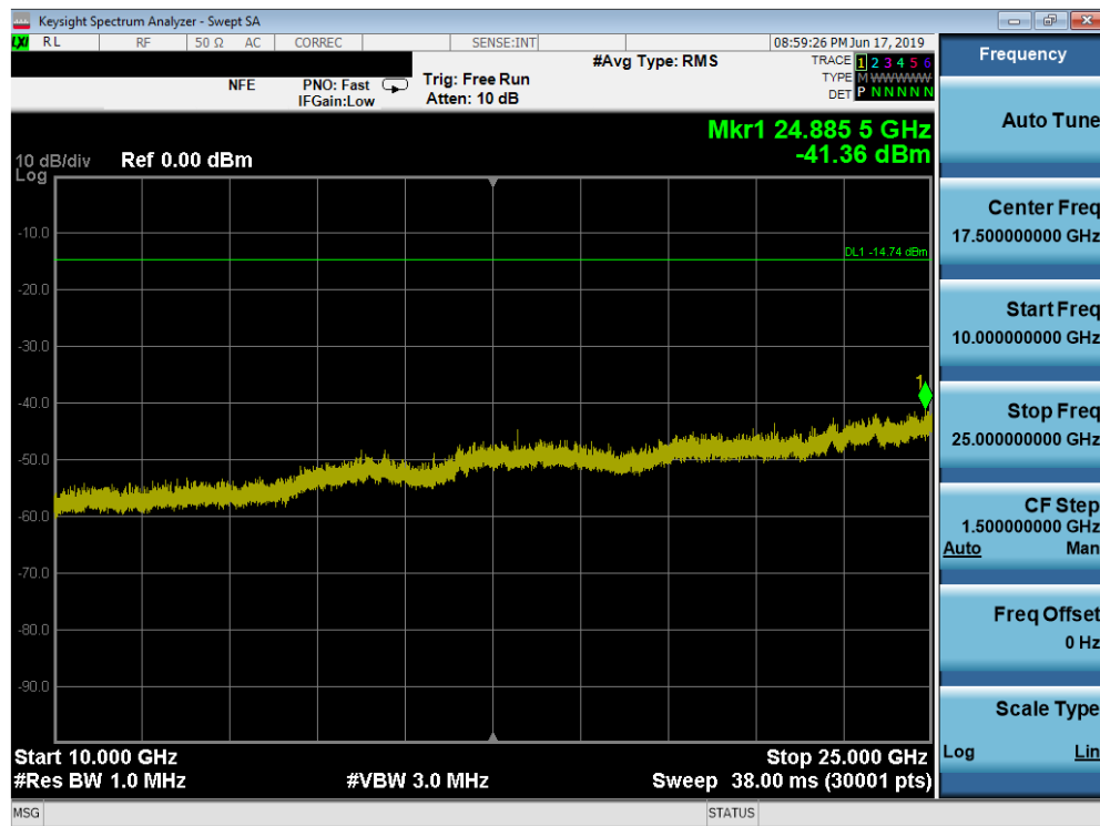
Plot 7-40. Conducted Spurious Plot (Bluetooth (LE), 2Mbps – Ch. 0)
