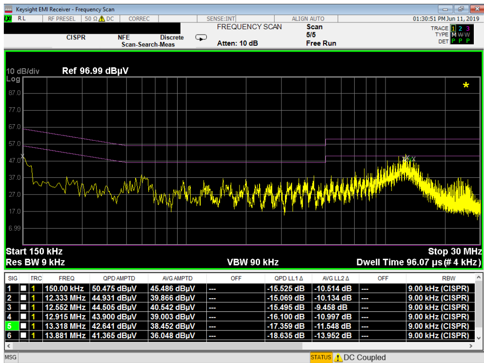
Plot 7-48. Line Conducted Plot with Bluetooth LE (N)
