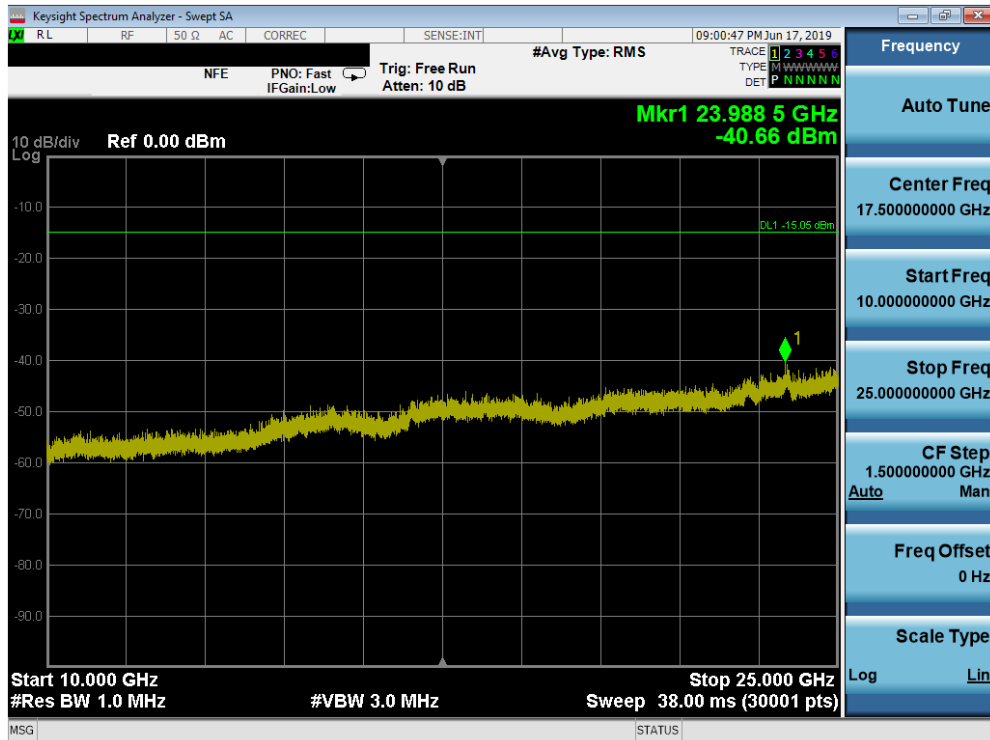
Plot 7-42. Conducted Spurious Plot (Bluetooth (LE), 2Mbps – Ch. 19)
