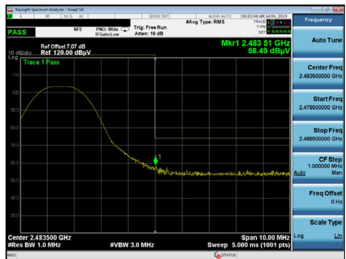
Plot 7-46. Radiated Restricted Upper Band Edge Measurement (Peak)
