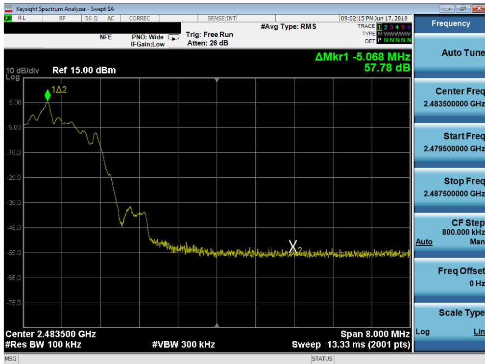
Plot 7-38. Band Edge Plot (Bluetooth (LE), 2Mbps – Ch. 39)
