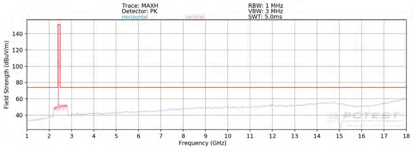
Plot 7-92. Radiated Spurious Plot above 1GHz SISO ANT1 (802.11b – Ch. 1)
