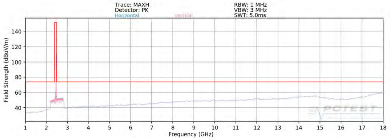
Plot 7-94. Radiated Spurious Plot above 1GHz SISO ANT1 (802.11b – Ch. 11)
