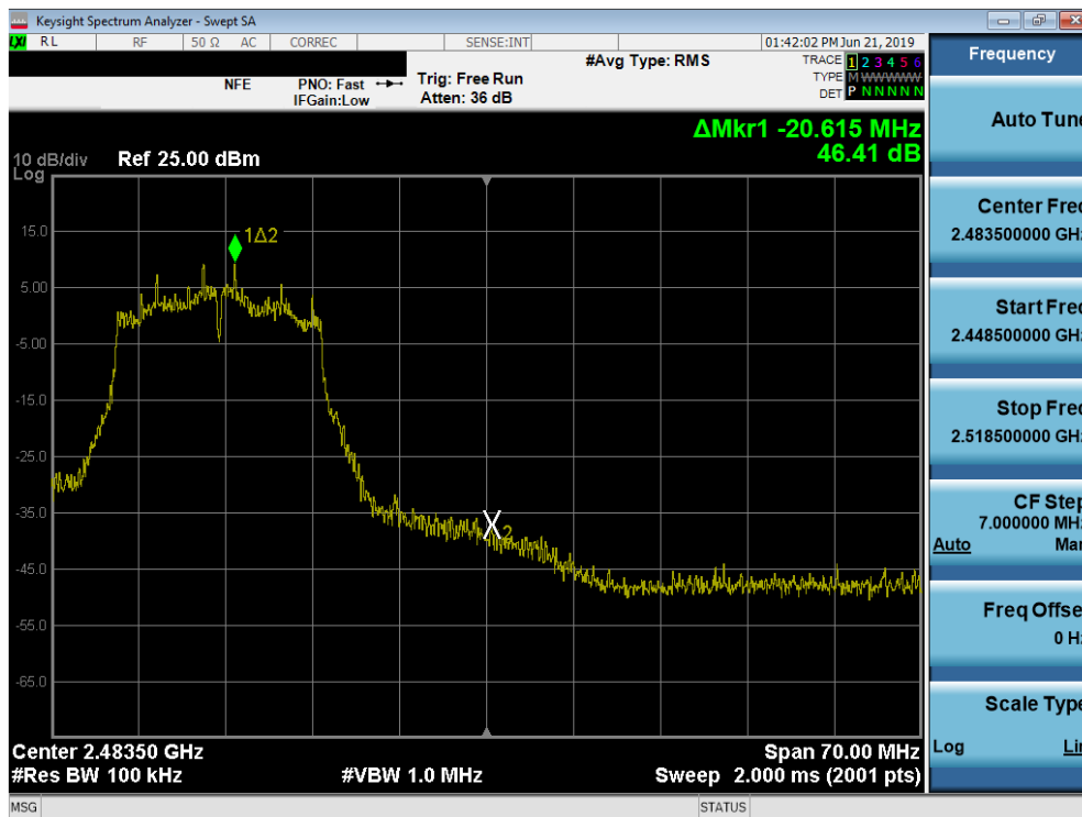
Plot 7-47. Band Edge Plot SISO ANT1 (802.11g – Ch. 11)
