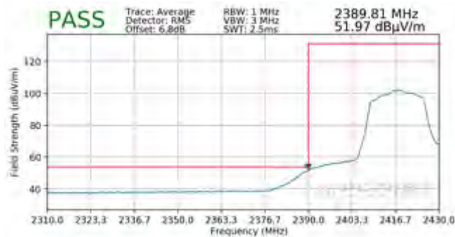
Plot 7-106. Radiated Restricted Lower Band Edge Measurement SISO ANT1 (Average)
