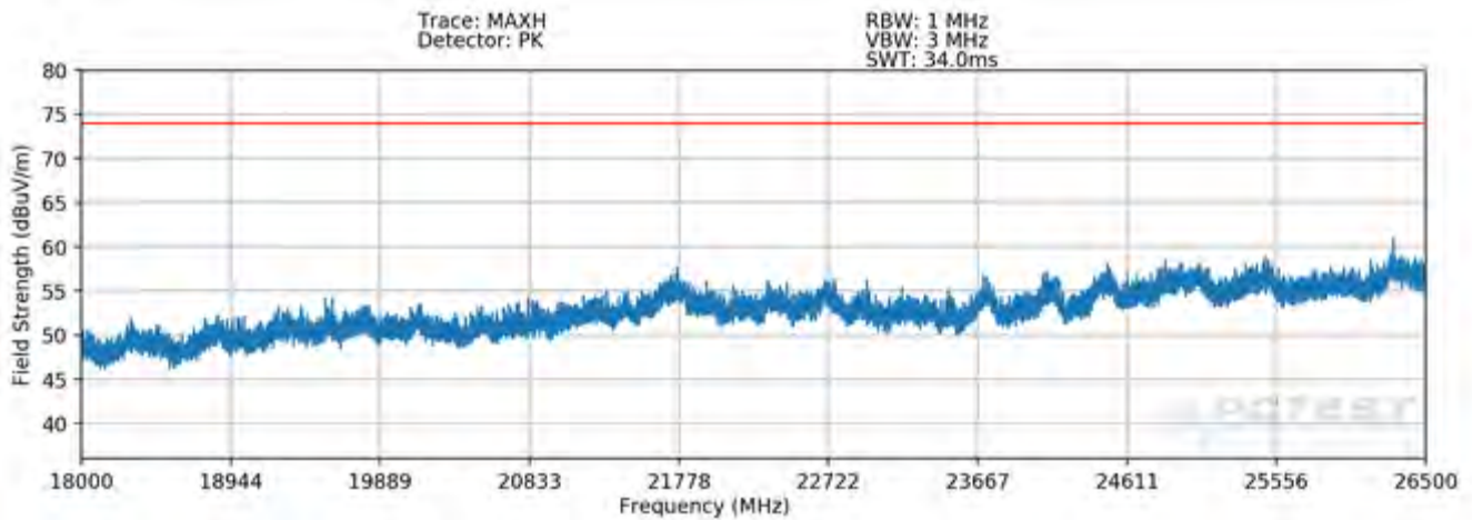
Plot 7-103. Radiated Spurious Plot above 18GHz MIMO/CDD
