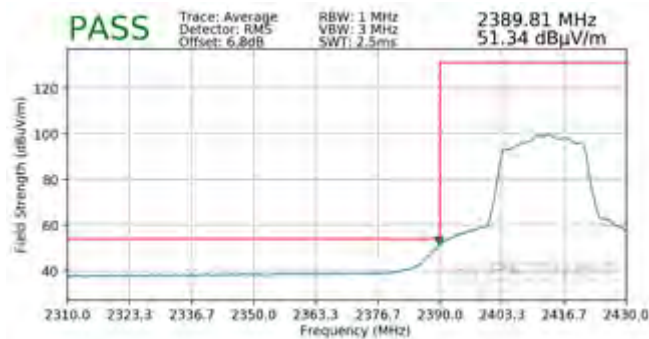
Plot 7-104. Radiated Restricted Lower Band Edge Measurement SISO ANT1 (Average)
