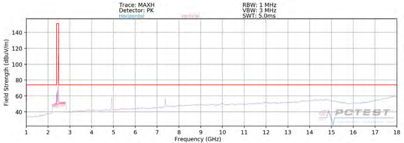
Plot 7-98. Radiated Spurious Plot above 1GHz SISO ANT2 (802.11b – Ch. 11)
