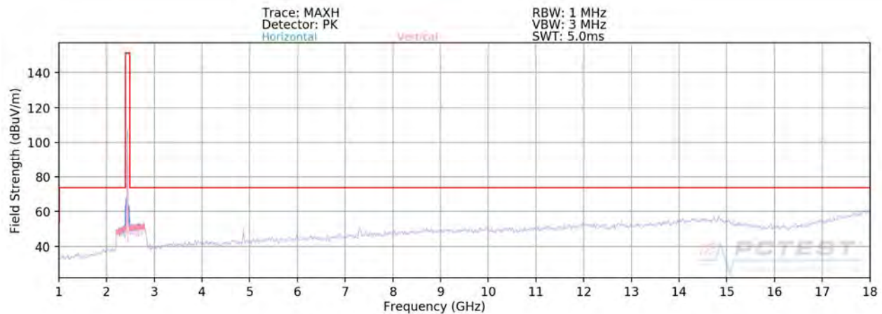
Plot 7-101. Radiated Spurious Plot above 1GHz MIMO/CDD (802.11g – Ch. 6)
