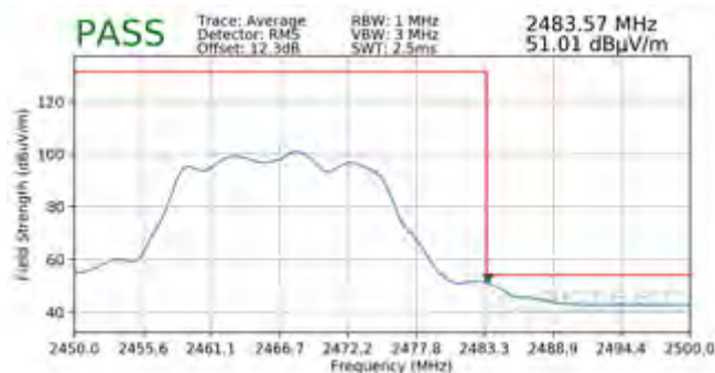
Plot 7-144. Radiated Restricted Upper Band Edge Measurement MIMO (Average)
