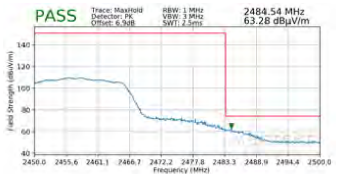
Plot 7-115. Radiated Restricted Upper Band Edge Measurement SISO ANT1 (Peak)
