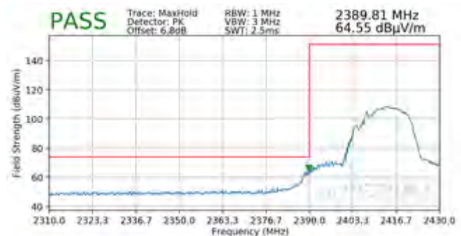
Plot 7-135. Radiated Restricted Lower Band Edge Measurement MIMO (Peak)
