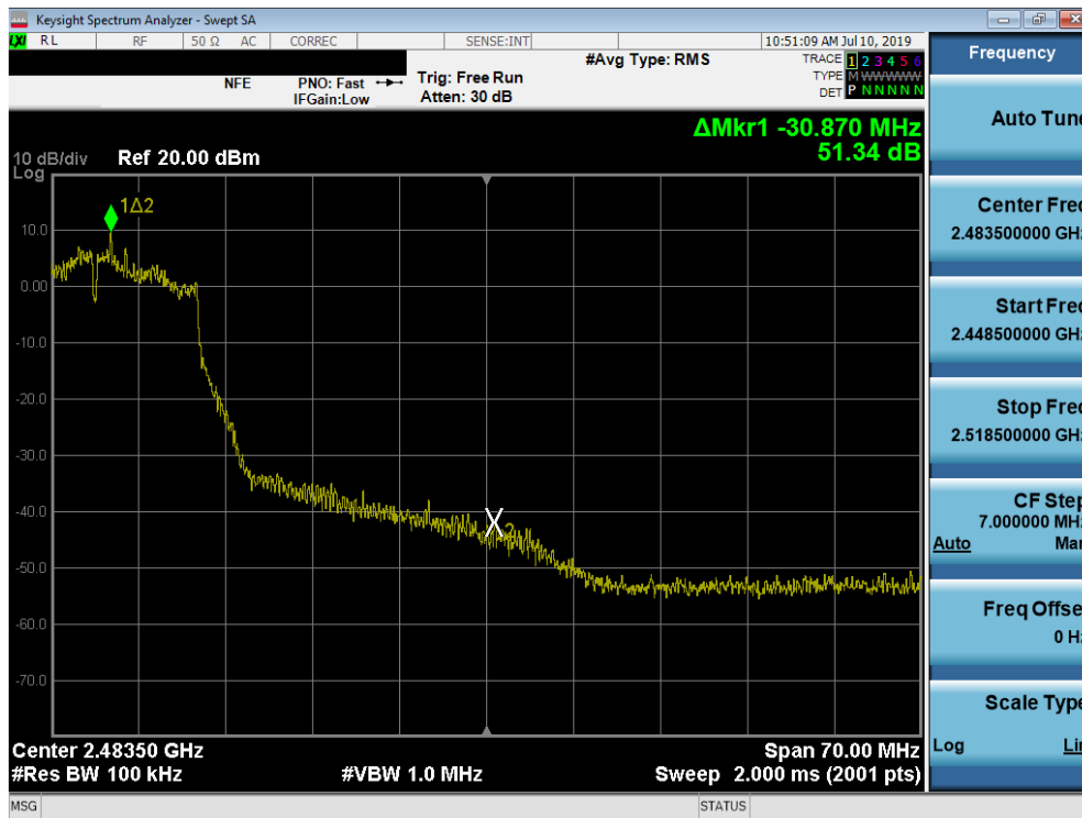
Plot 7-45. Band Edge Plot SISO ANT1 (802.11g - Ch. 9)
