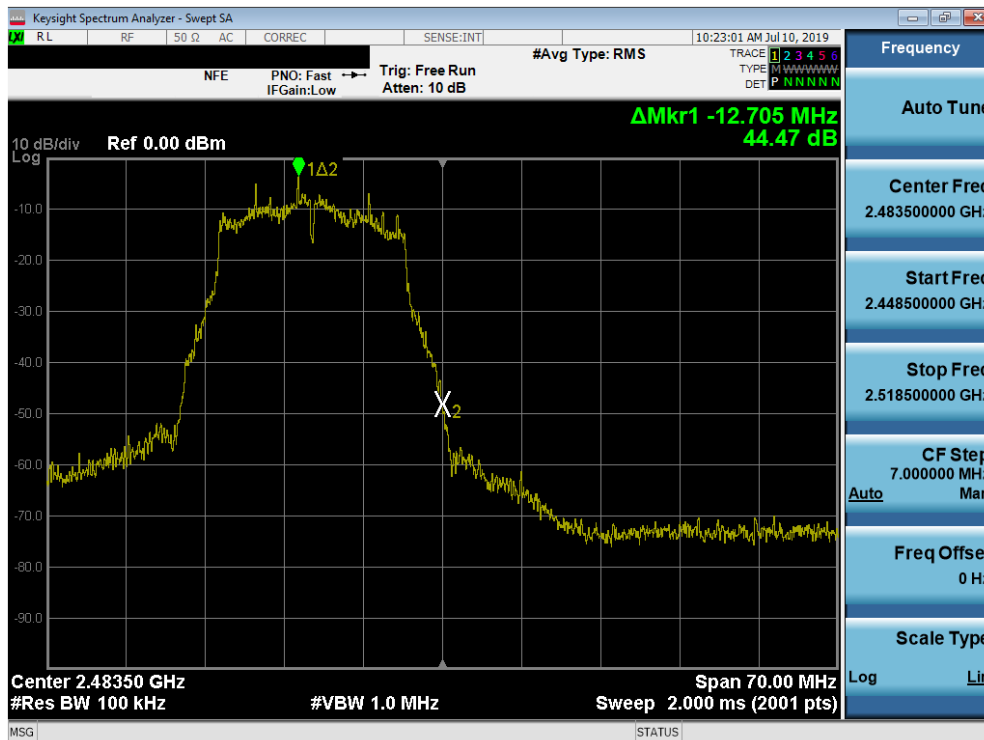
Plot 7-70. Band Edge Plot SISO ANT2 (802.11g – Ch. 13)
