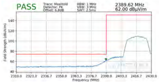
Plot 7-107. Radiated Restricted Lower Band Edge Measurement SISO ANT1 (Peak)
