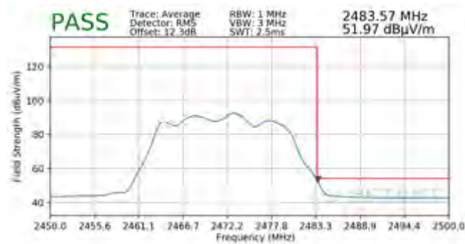
Plot 7-146. Radiated Restricted Upper Band Edge Measurement MIMO (Average)
