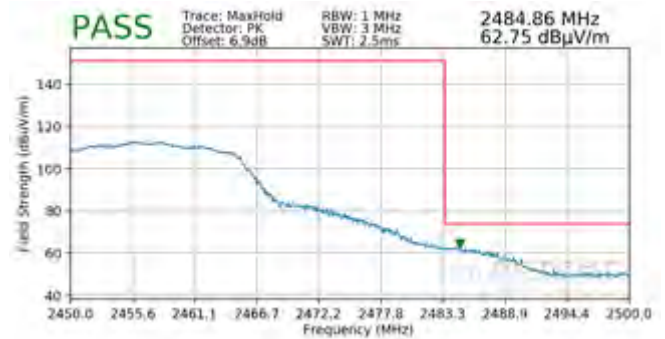
Plot 7-127. Radiated Restricted Upper Band Edge Measurement SISO ANT2 (Peak)
