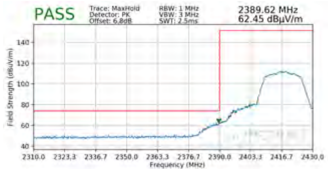
Plot 7-125. Radiated Restricted Lower Band Edge Measurement SISO ANT2 (Peak)
