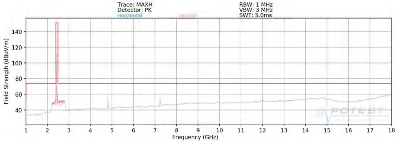
Plot 7-96. Radiated Spurious Plot above 1GHz SISO ANT2 (802.11b – Ch. 1)
