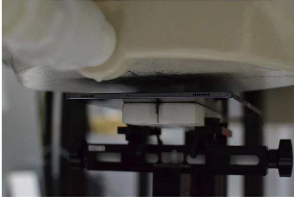
SAR Test Setup Photo 1: Back at 15.0 mm
