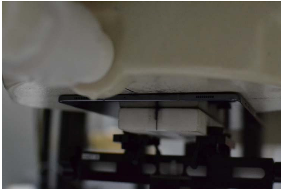
SAR Test Setup Photo 2: Back at 0.0 mm
