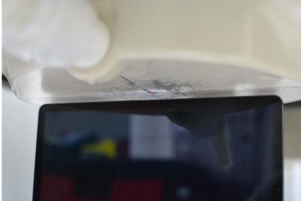
SAR Test Setup Photo 5: Right at 6.0 mm
