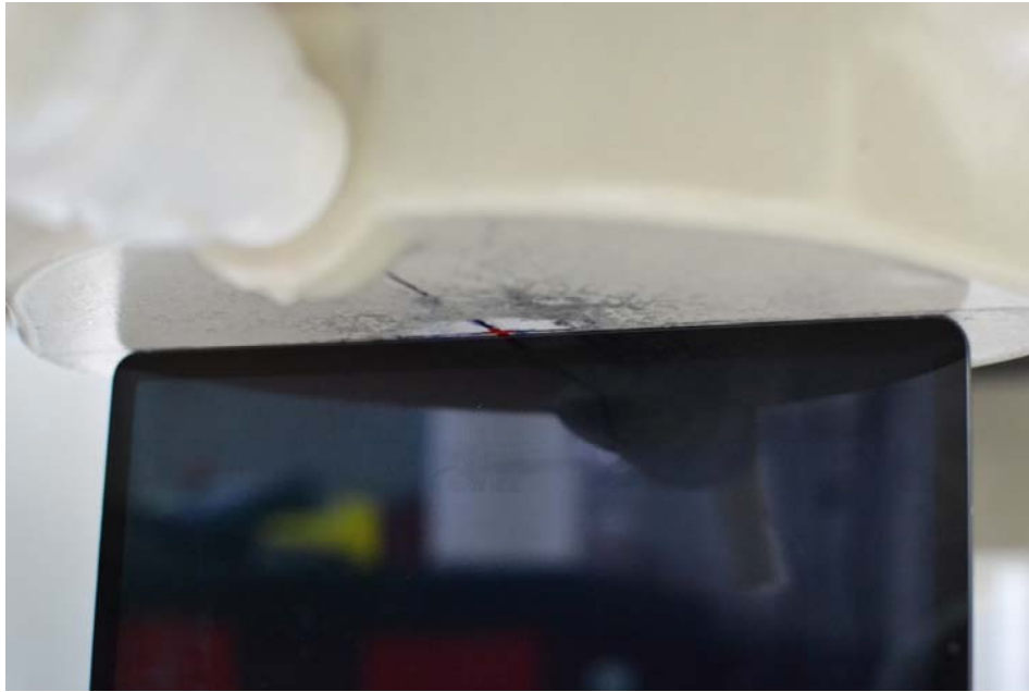
SAR Test Setup Photo 8: Left at 0.0 mm
