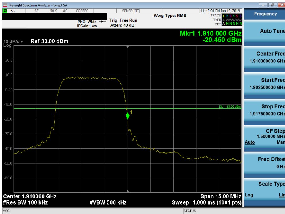
Plot 7-65. Band Edge Plot (PCS WCDMA Mode - High Channel)
