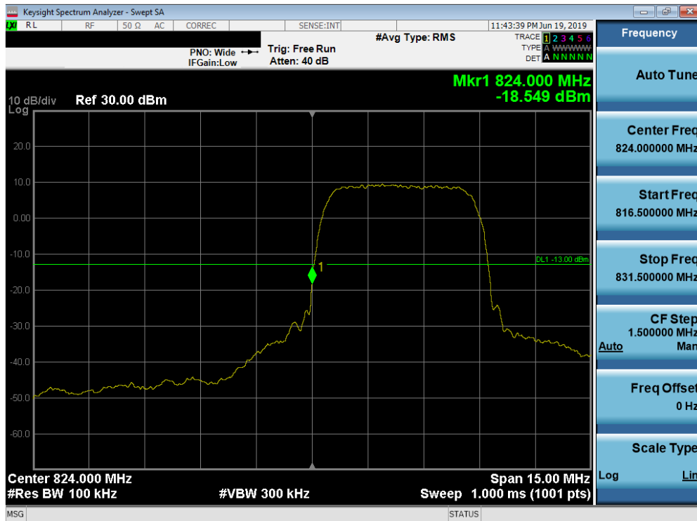
Plot 7-57. Band Edge Plot (Cellular WCDMA Mode - Low Channel)
