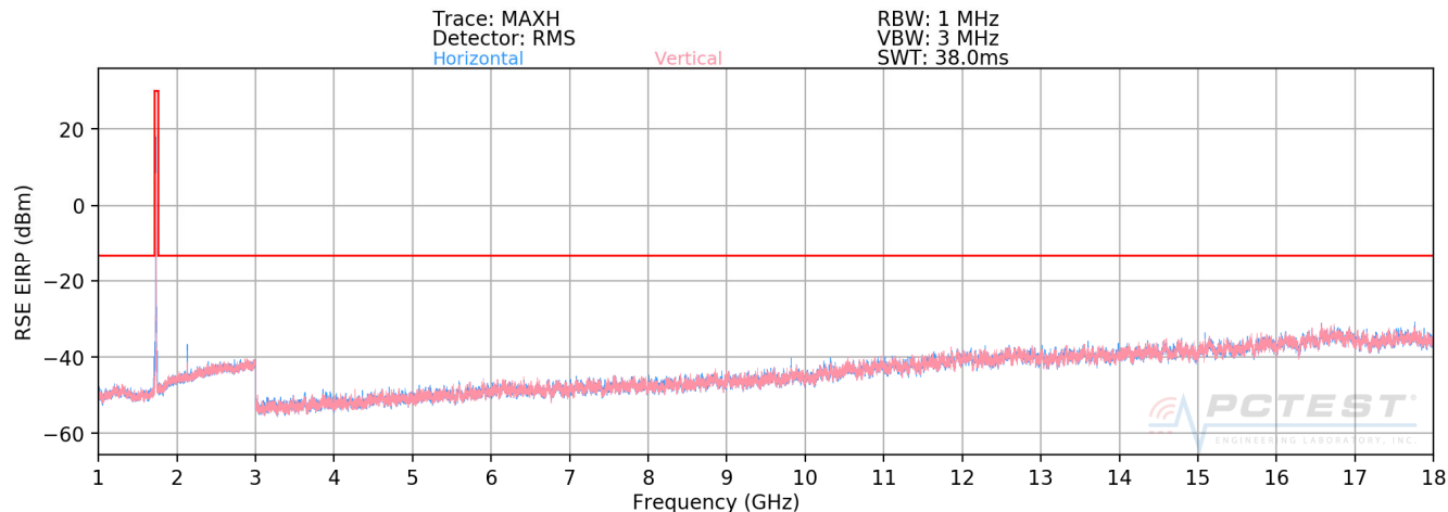
Plot 7-73. Radiated Spurious Plot above 1GHz (AWS WCDMA Mode)
