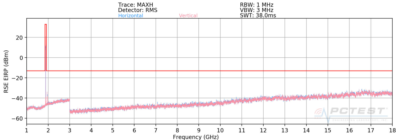
Plot 7-74. Radiated Spurious Plot above 1GHz (PCS GPRS Mode)
