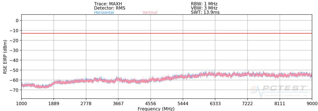
Plot 7-72. Radiated Spurious Plot above 1GHz (Cellular WCDMA Mode)
