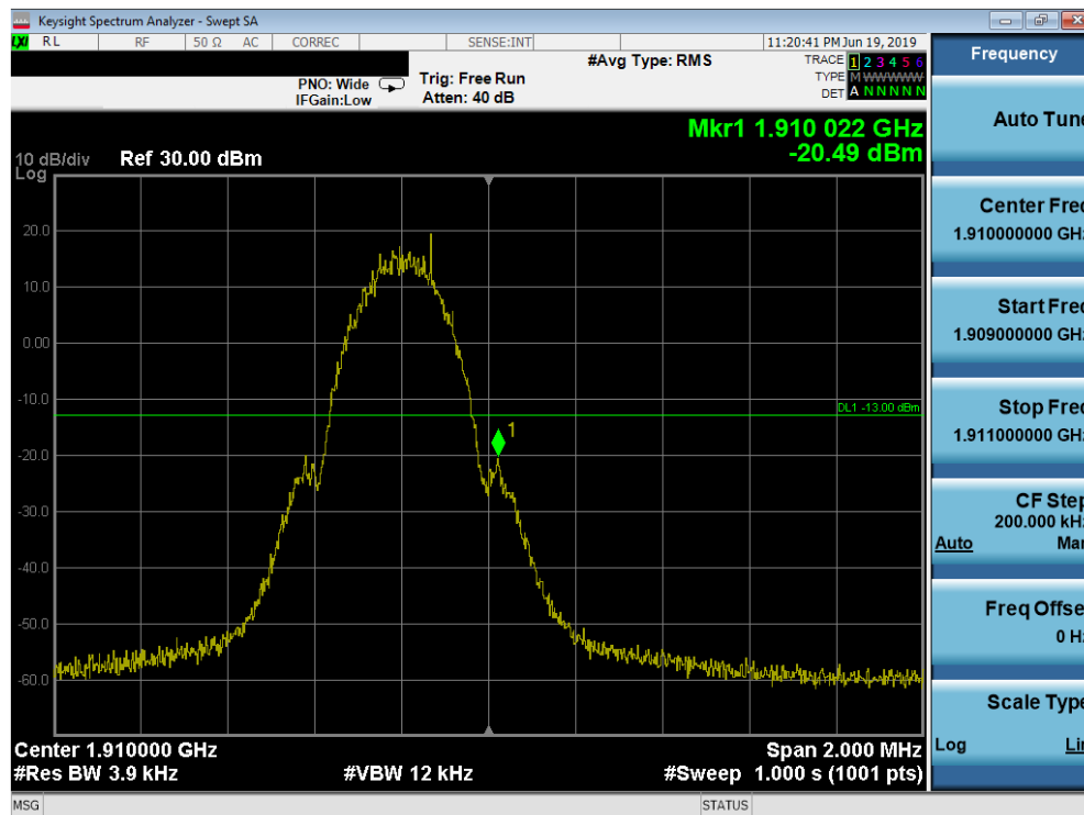
Plot 7-56. Band Edge Plot (PCS GPRS Mode - High Channel)
