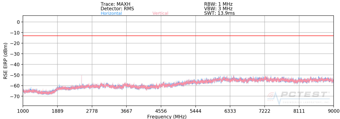
Plot 7-71. Radiated Spurious Plot above 1GHz (Cellular GPRS Mode)
