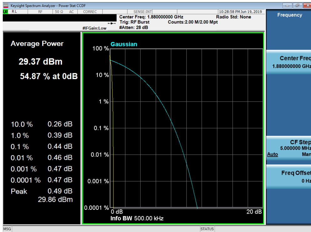
Plot 7-67. Peak-Average Ratio Plot (PCS GPRS Mode)
