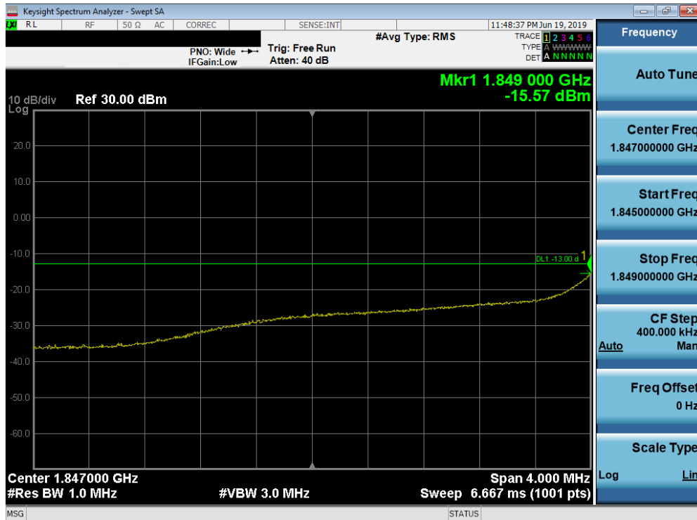
Plot 7-64. 4MHz Span Plot (PCS WCDMA Mode - Low Channel)
