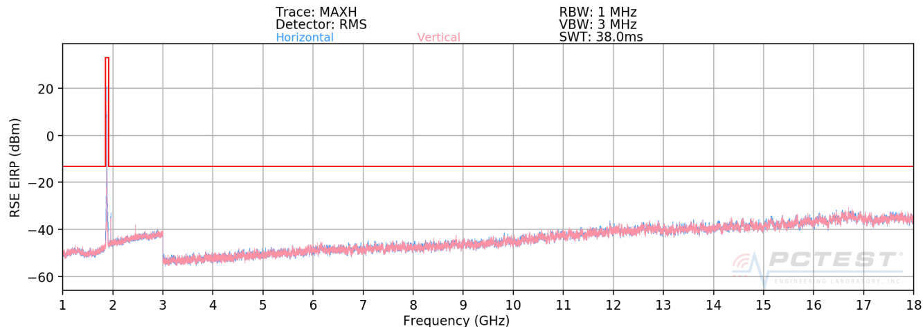
Plot 7-75. Radiated Spurious Plot above 1GHz (PCS WCDMA Mode)
