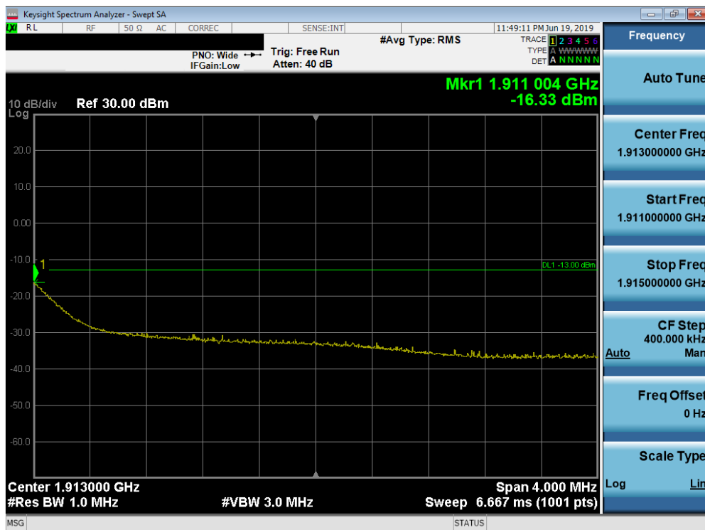
Plot 7-66. 4MHz Span Plot (PCS WCDMA Mode - High Channel)
