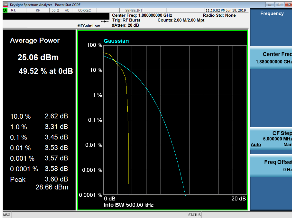
Plot 7-68. Peak-Average Ratio Plot (EDGE1900 Mode)
