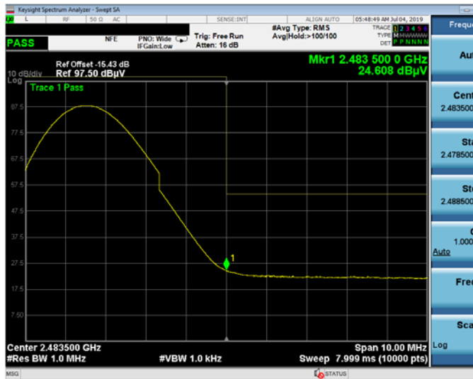
Plot 7-46. Radiated Restricted Upper Band Edge Measurement (Average)
