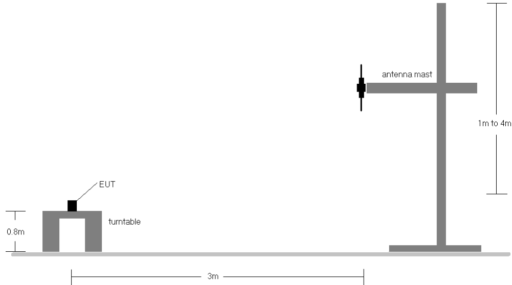
Figure 7-4. ERP/EIRP Measurement Setup
