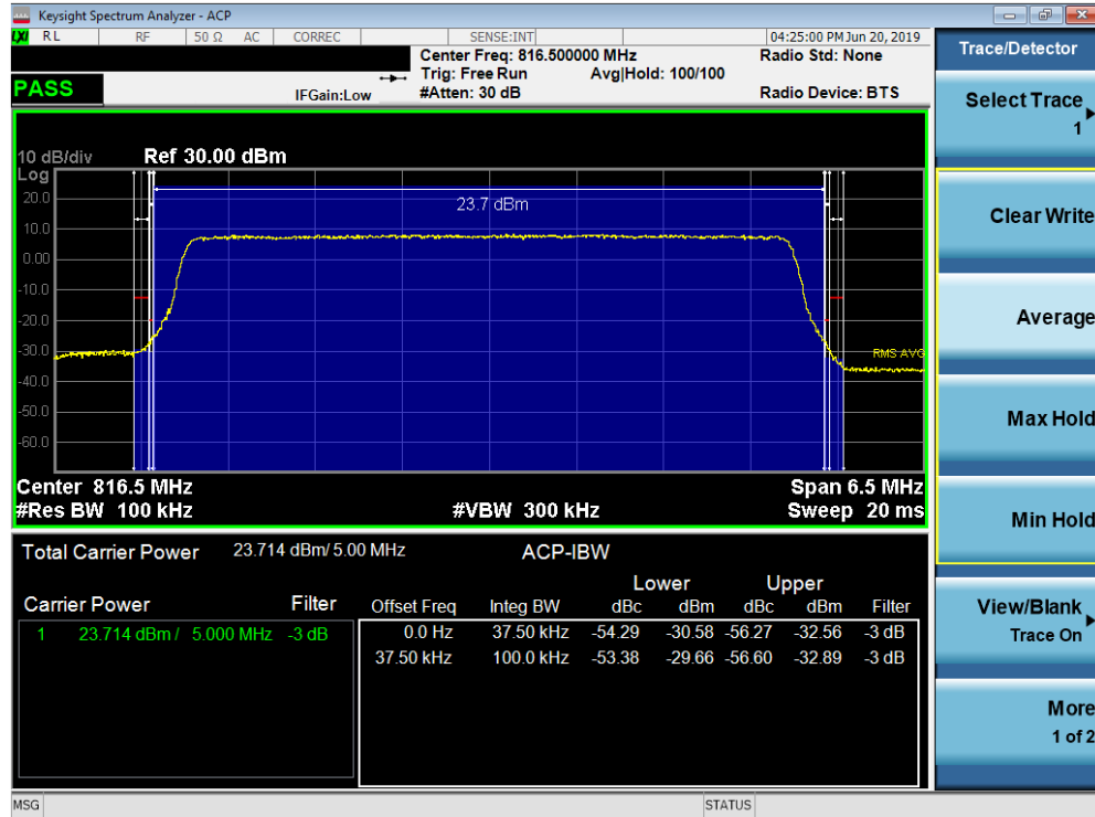
Plot 7-26. Channel Edge Plot (LTE Band 26, 5MHz QPSK – RB Size 25– Low Channel)
