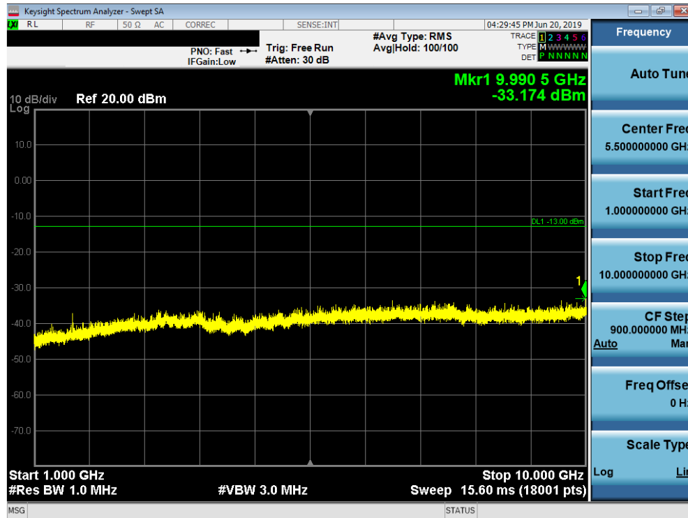
Plot 7-18. Conducted Spurious Plot (LTE Band 26, 5 MHz QPSK – RB Size 1, RB Offset 0 – Low Channel)
