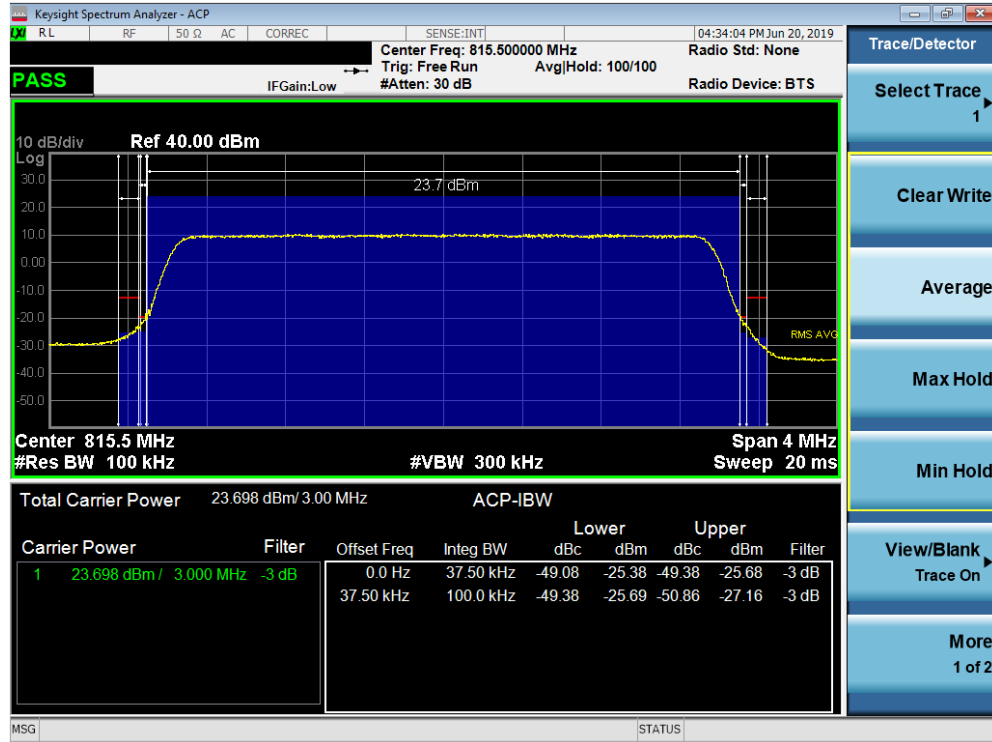
Plot 7-24. Channel Edge Plot (LTE Band 26, 3MHz QPSK – RB Size 15– Low Channel)
