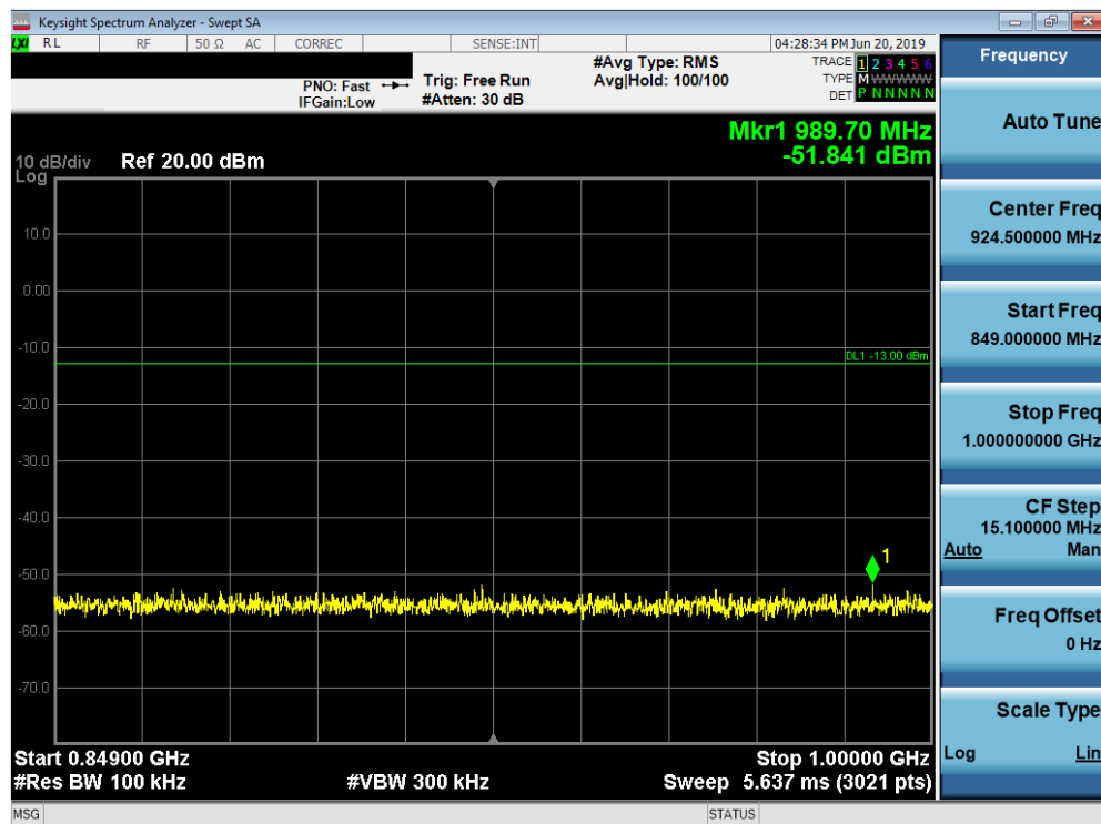
Plot 7-17. Conducted Spurious Plot (LTE Band 26, 5 MHz QPSK – RB Size 1, RB Offset 0 – Low Channel)
