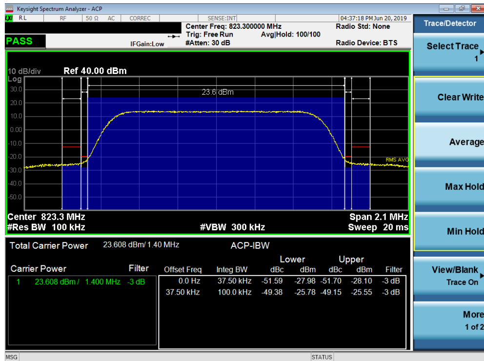
Plot 7-23. Channel Edge Plot (LTE Band 26, 1.4MHz QPSK – RB Size 6 – High Channel)
