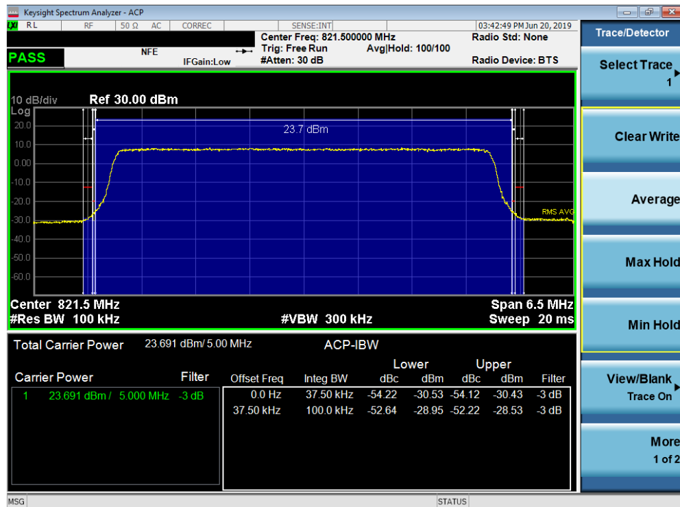
Plot 7-27. Channel Edge Plot (LTE Band 26, 5MHz QPSK – RB Size 25 – High Channel)
