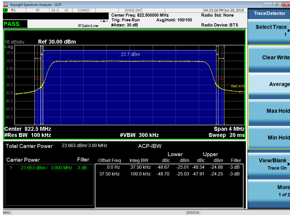
Plot 7-25. Channel Edge Plot (LTE Band 26, 3MHz QPSK – RB Size 15 – High Channel)
