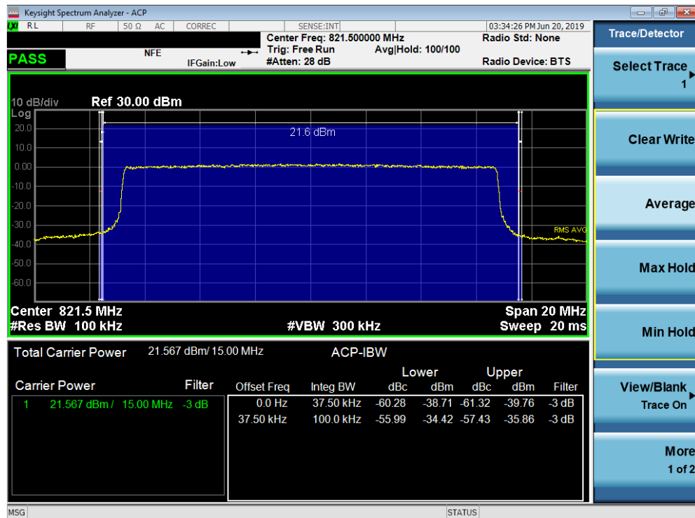
Plot 7-29. Channel Edge Plot (LTE Band 26, 15MHz QPSK – RB Size 75)
