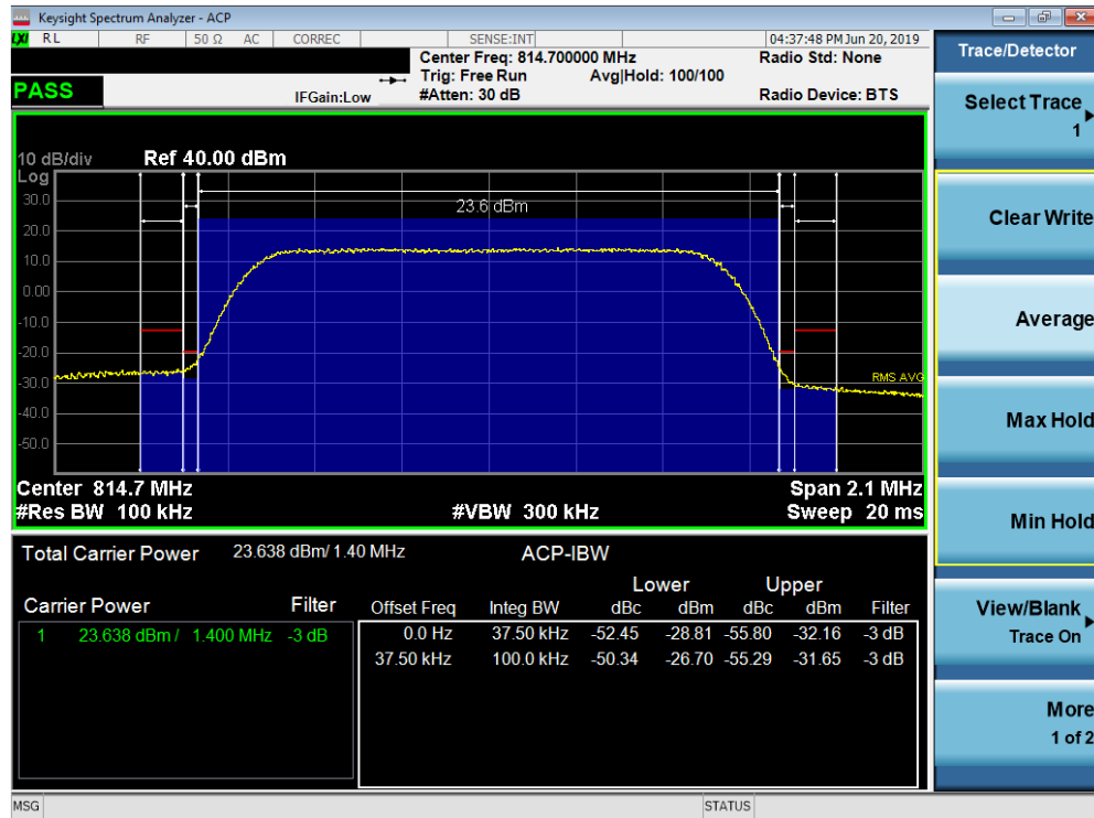
Plot 7-22. Channel Edge Plot (LTE Band 26, 1.4MHz QPSK – RB Size 6– Low Channel)
