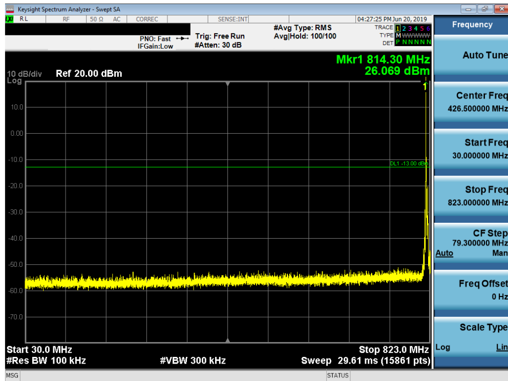
Plot 7-16. Conducted Spurious Plot (LTE Band 26, 5 MHz QPSK – RB Size 1, RB Offset 0 – Low Channel)
