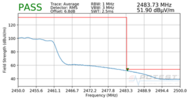
Plot 7-112. Radiated Restricted Upper Band Edge Measurement SISO ANT1 (Average)
