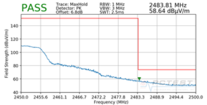
Plot 7-111. Radiated Restricted Upper Band Edge Measurement SISO ANT1 (Peak)
