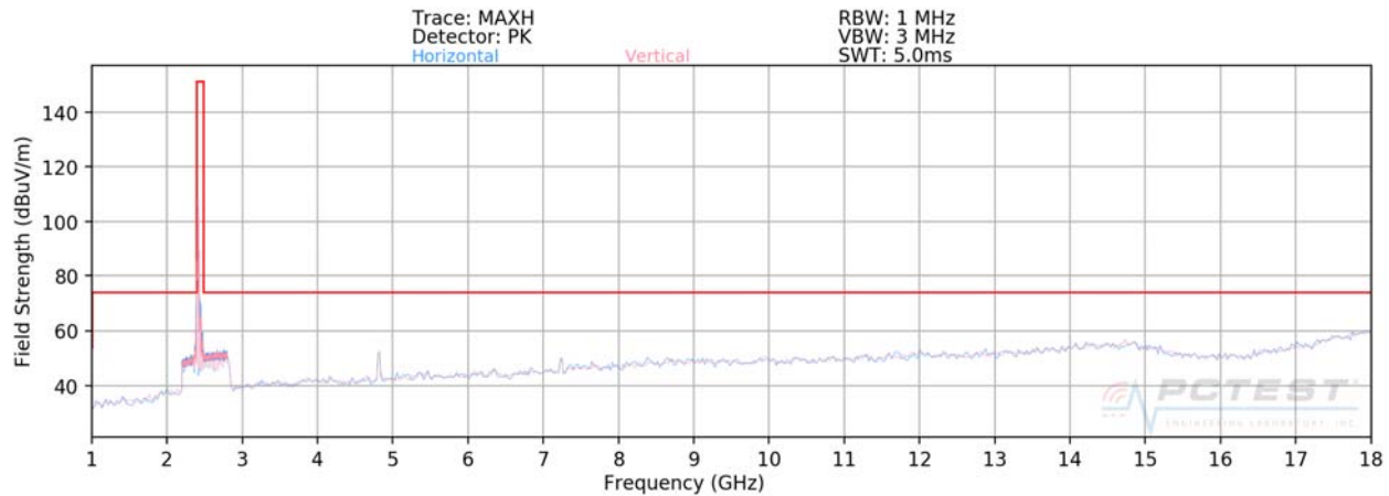
Plot 7-100. Radiated Spurious Plot above 1GHz MIMO/CDD (802.11g – Ch. 1)
