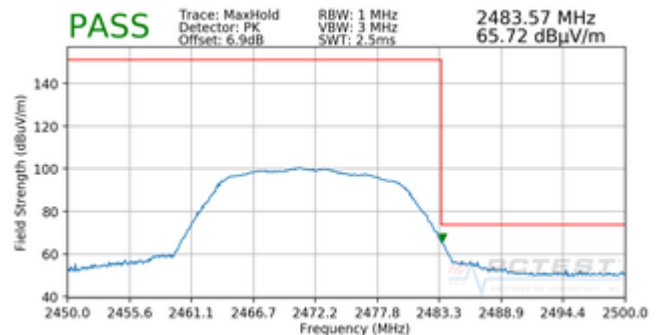
Plot 7-133. Radiated Restricted Upper Band Edge Measurement SISO ANT2 (Peak)
