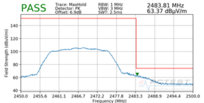
Plot 7-119. Radiated Restricted Upper Band Edge Measurement SISO ANT1 (Peak)
