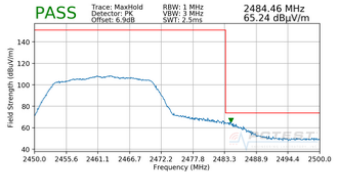
Plot 7-117. Radiated Restricted Upper Band Edge Measurement SISO ANT1 (Peak)
