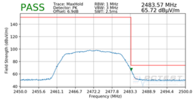
Plot 7-121. Radiated Restricted Upper Band Edge Measurement SISO ANT1 (Peak)
