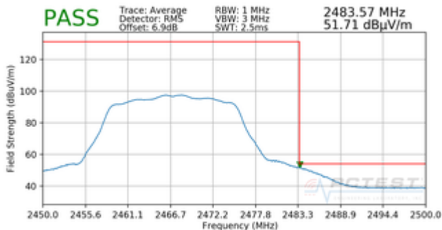
Plot 7-118. Radiated Restricted Upper Band Edge Measurement SISO ANT1 (Average)
