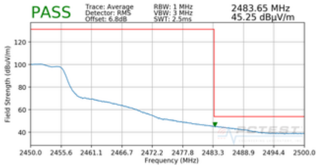
Plot 7-110. Radiated Restricted Upper Band Edge Measurement SISO ANT1 (Average)
