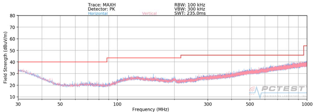
Plot 7-149. Radiated Spurious Plot below 1GHz SISO ANT2
