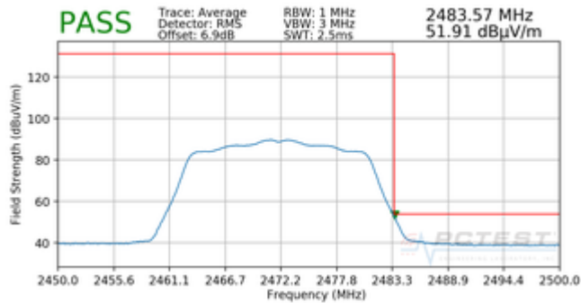
Plot 7-120. Radiated Restricted Upper Band Edge Measurement SISO ANT1 (Average)
