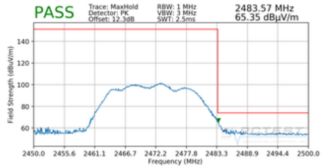
Plot 7-147. Radiated Restricted Upper Band Edge Measurement MIMO (Peak)
