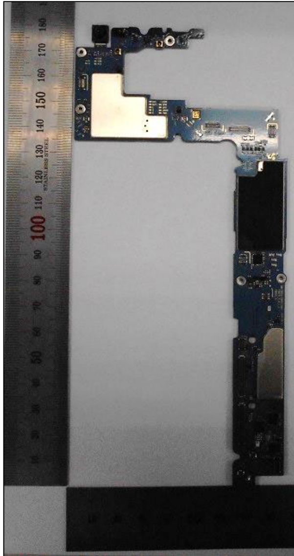
PBA TOP with Front CAM
