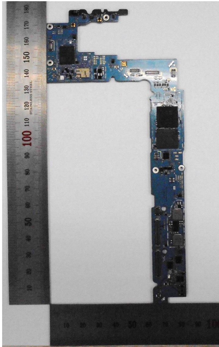
PBA TOP without Shield Can
