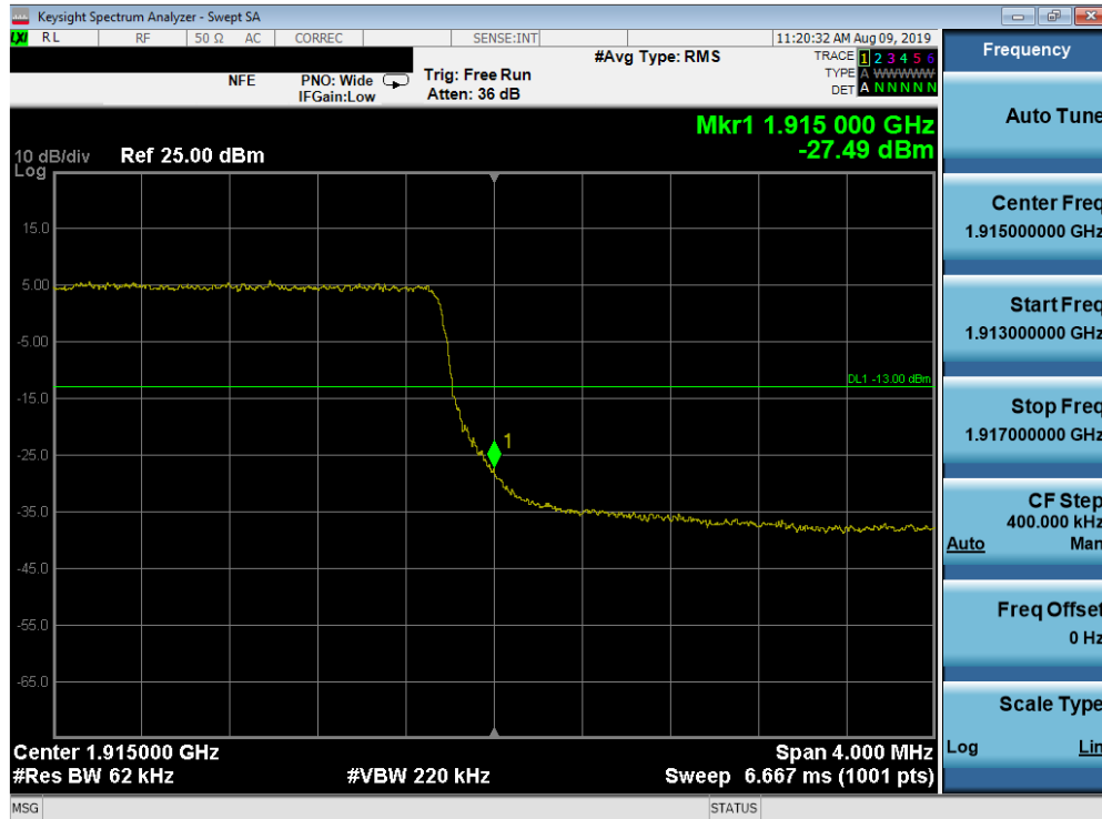
Plot 7-267. Upper Band Edge Plot (Band 25 - 5.0MHz QPSK - Full RB Configuration)
