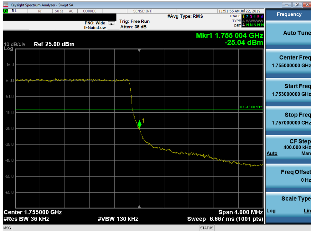
Plot 7-223. Upper Band Edge Plot (Band 4 - 3.0MHz QPSK - Full RB Configuration)
