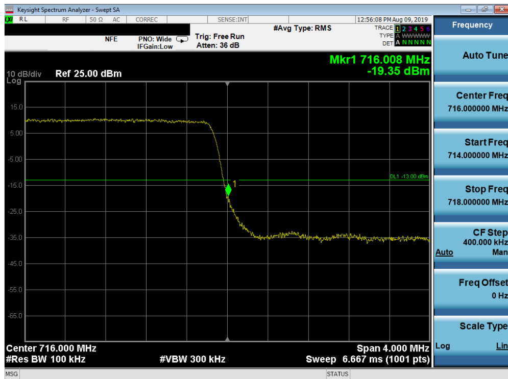
Plot 7-192. Upper Band Edge Plot (Band 12 - 3.0MHz QPSK - Full RB Configuration)
