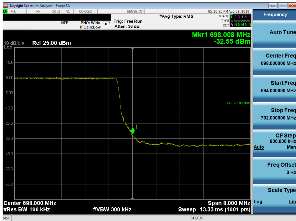
Plot 7-184. Upper Band Edge Plot (Band 71 - 10.0MHz QPSK - Full RB Configuration)
