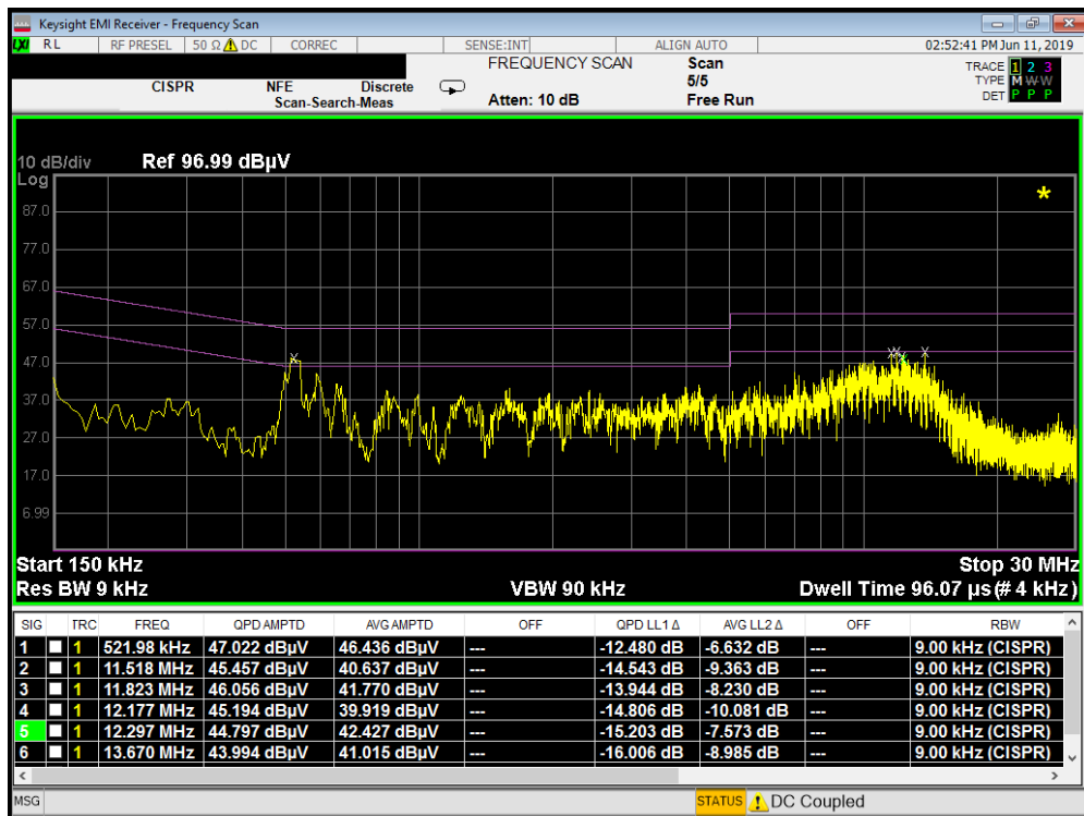
Plot 7-12. Line-Conducted Test Plot (L1) - Digitizer Mode 1
