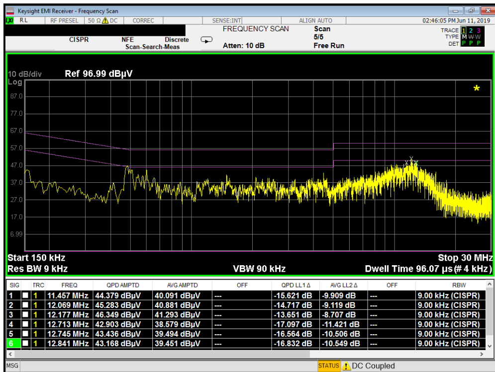
Plot 7-10. Line-Conducted Test Plot (L1) - Device to S-Pen WPT
