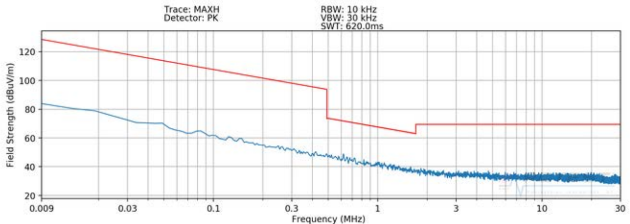
Plot 7-6. Radiated Spurious Plot 9kHz – 30MHz (Pol. Z – Digitizer Mode 1)
