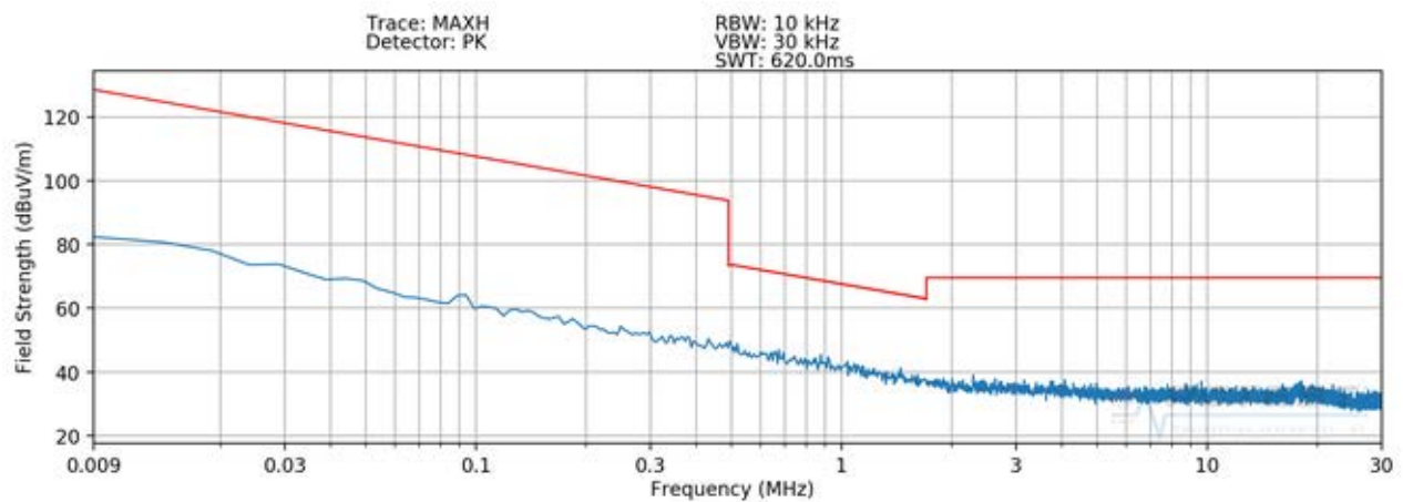
Plot 7-8 Radiated Spurious Plot 9kHz – 30MHz (Pol. Y – Digitizer Mode 2)
