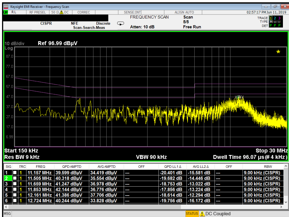
Plot 7-15. Line-Conducted Test Plot (N) - Digitizer Mode 2
