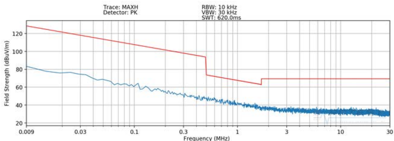
Plot 7-2 Radiated Spurious Plot 9kHz – 30MHz (Pol. Y – Device to S-Pen WPT)
