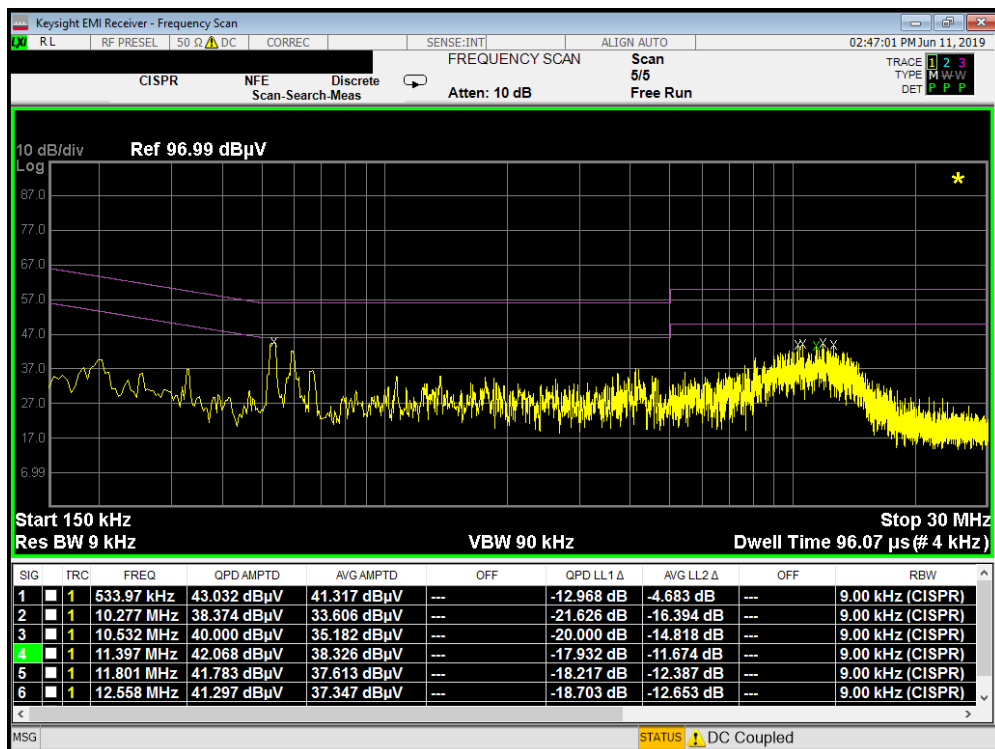
Plot 7-11. Line-Conducted Test Plot (N) - Device to S-pen WPT
