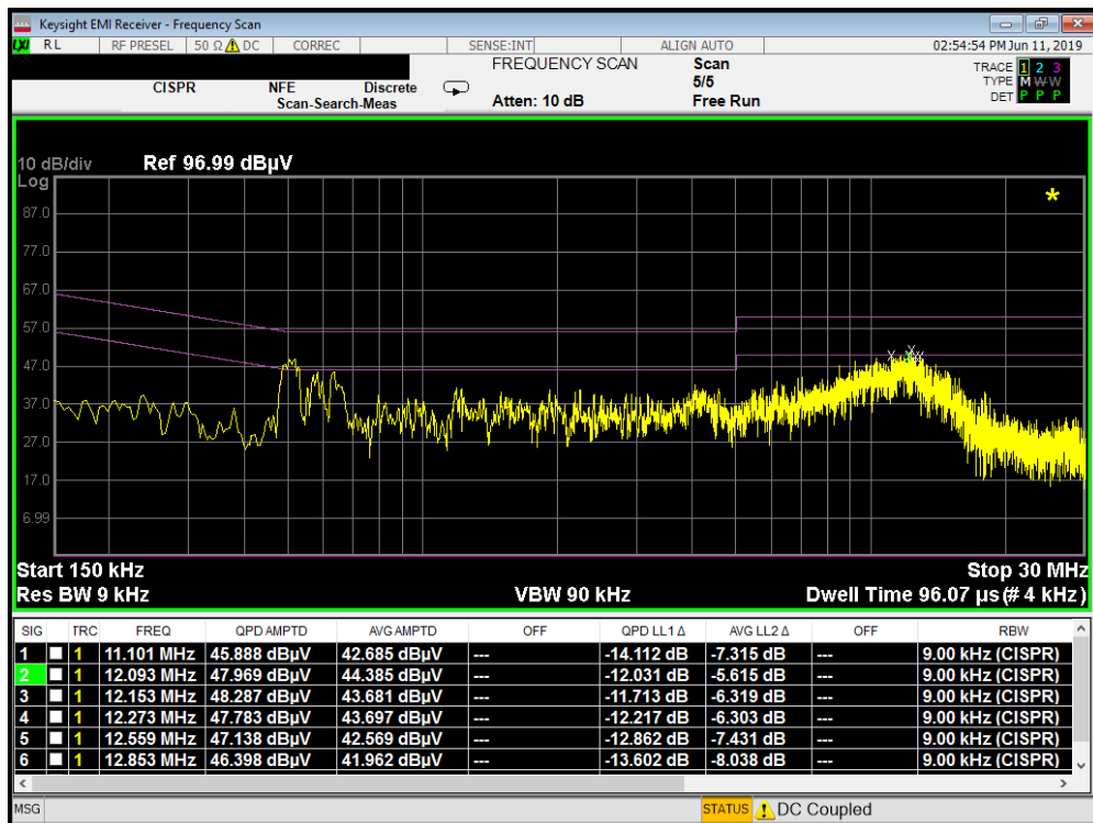
Plot 7-14. Line-Conducted Test Plot (L1) - Digitizer Mode 2
