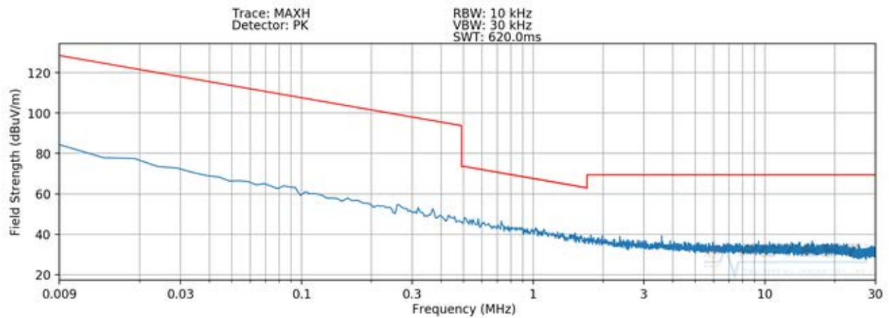
Plot 7-9. Radiated Spurious Plot 9kHz – 30MHz (Pol. Z – Digitizer Mode 2)
