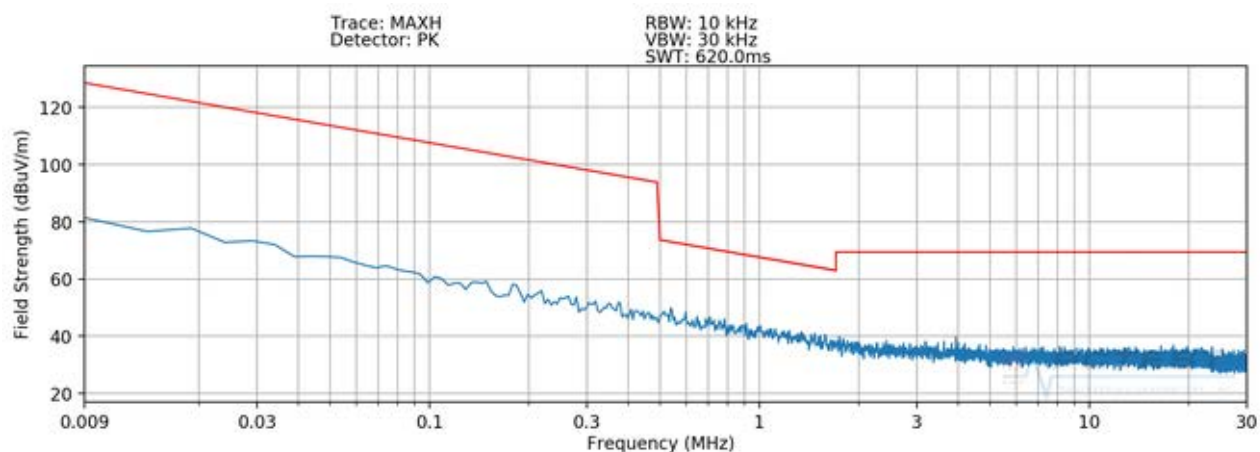
Plot 7-3. Radiated Spurious Plot 9kHz – 30MHz (Pol. Z – Device to S-Pen WPT)
