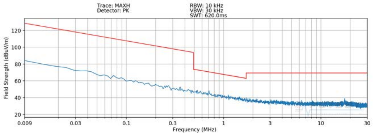
Plot 7-5 Radiated Spurious Plot 9kHz – 30MHz (Pol. Y – Digitizer Mode 1)
