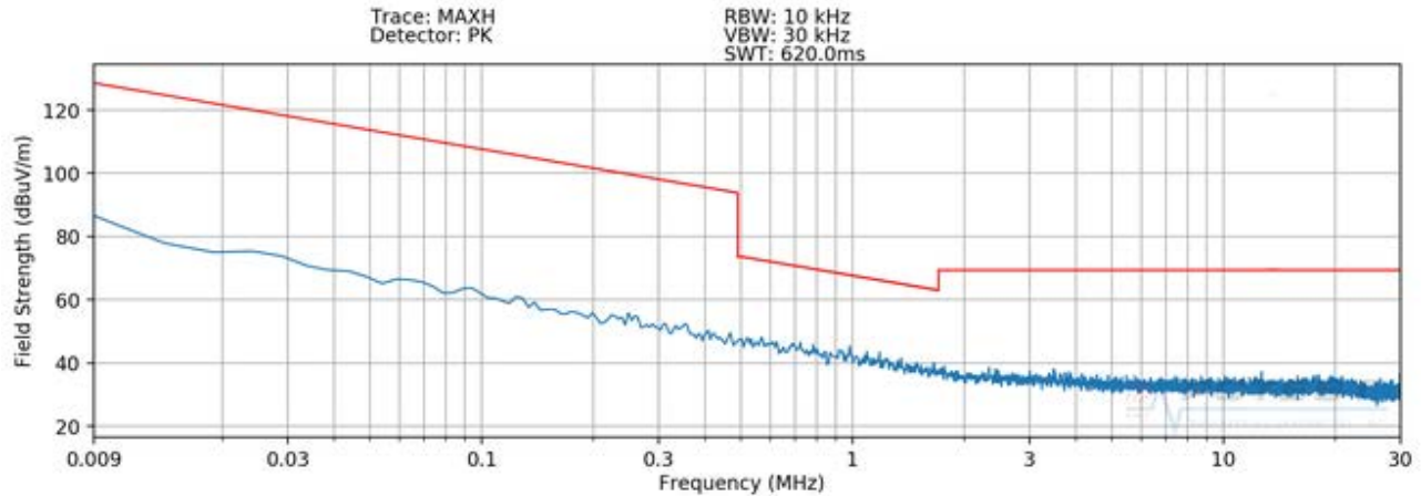
Plot 7-4. Radiated Spurious Plot 9kHz – 30MHz (Pol. X – Digitizer Mode 1)
