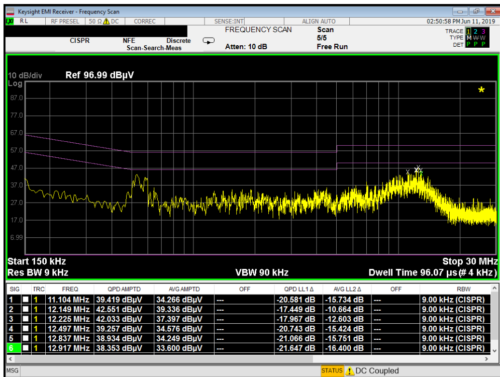
Plot 7-13. Line-Conducted Test Plot (N) - Digitizer Mode 1
