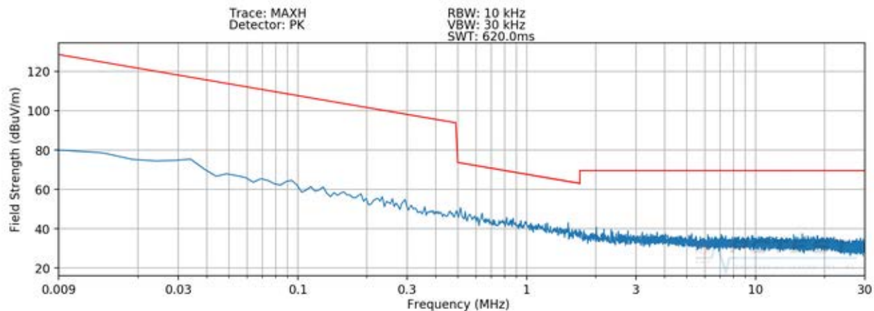
Plot 7-1. Radiated Spurious Plot 9kHz – 30MHz (Pol. X – Device to S-Pen WPT)
