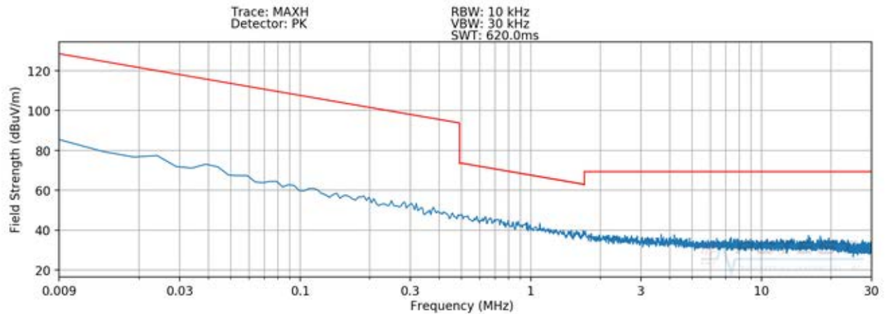
Plot 7-7. Radiated Spurious Plot 9kHz – 30MHz (Pol. X – Digitizer Mode 2)
