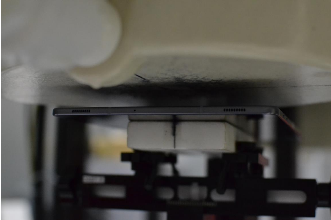
SAR Test Setup Photo 1 – Back Side at 1.6 cm
