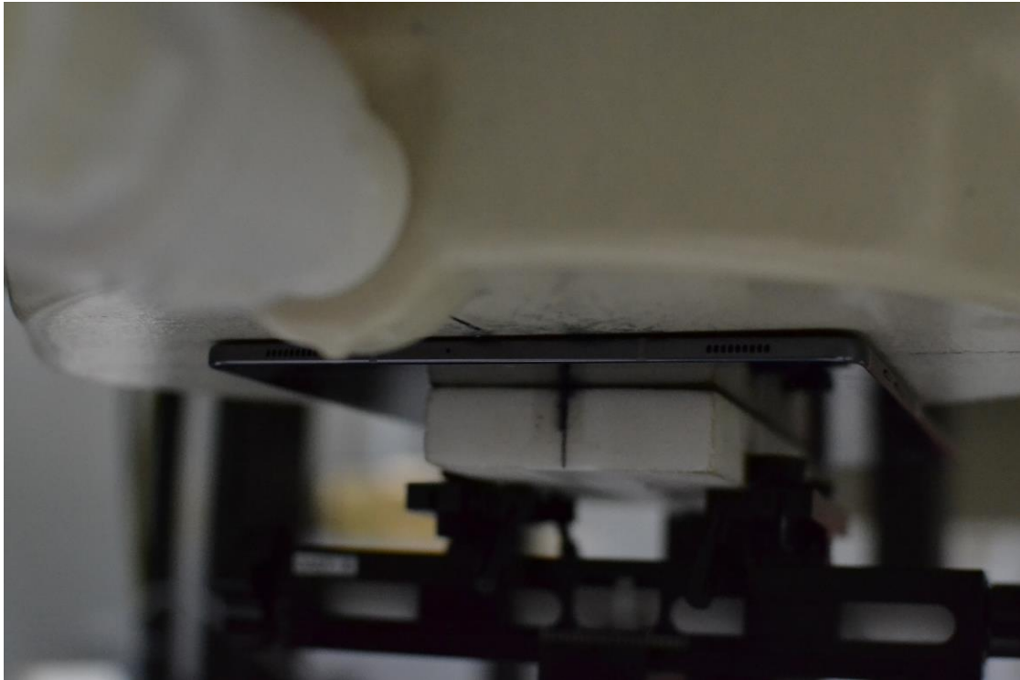
SAR Test Setup Photo 3 – Back Side at 0.0 cm
