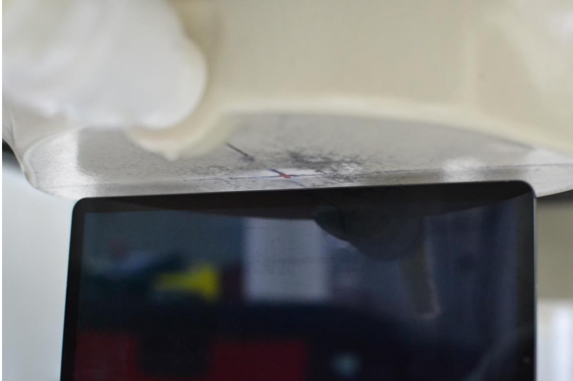
SAR Test Setup Photo 9 – Left Edge at 0.8 cm
