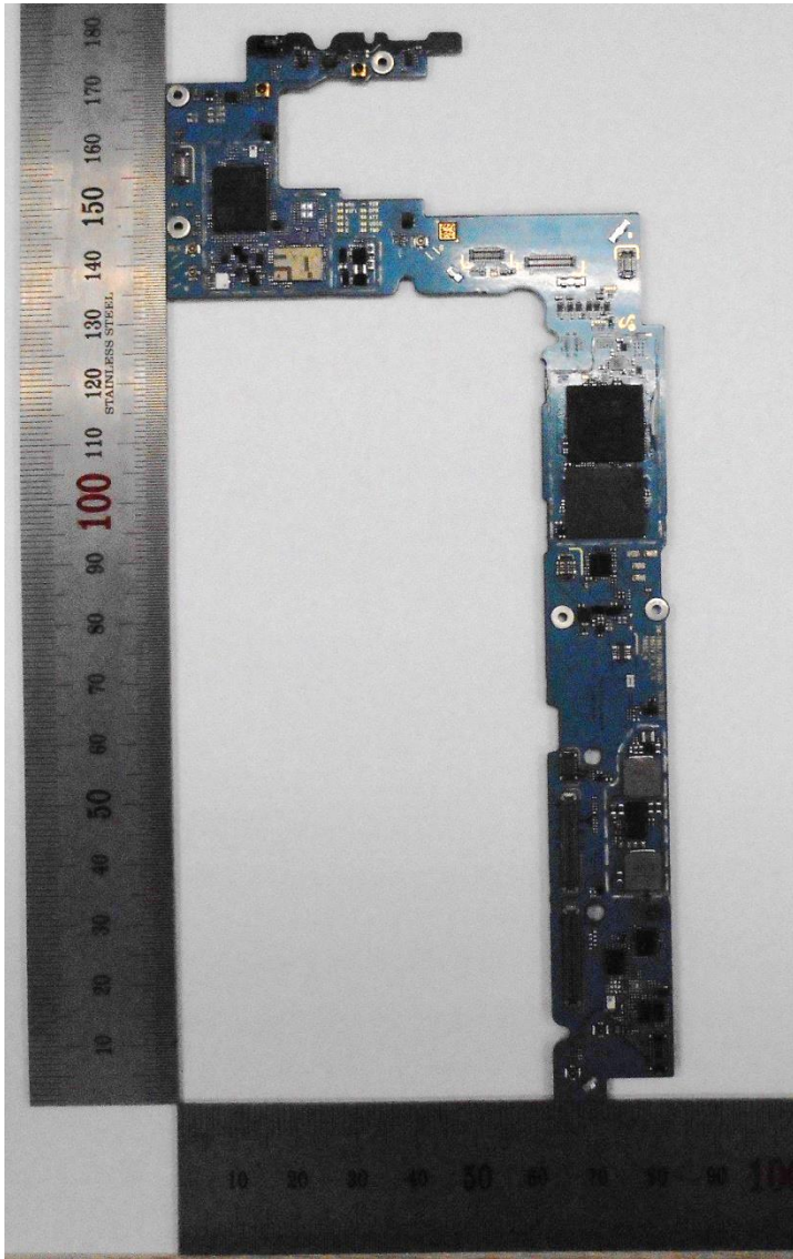
PBA TOP without Shield Can
