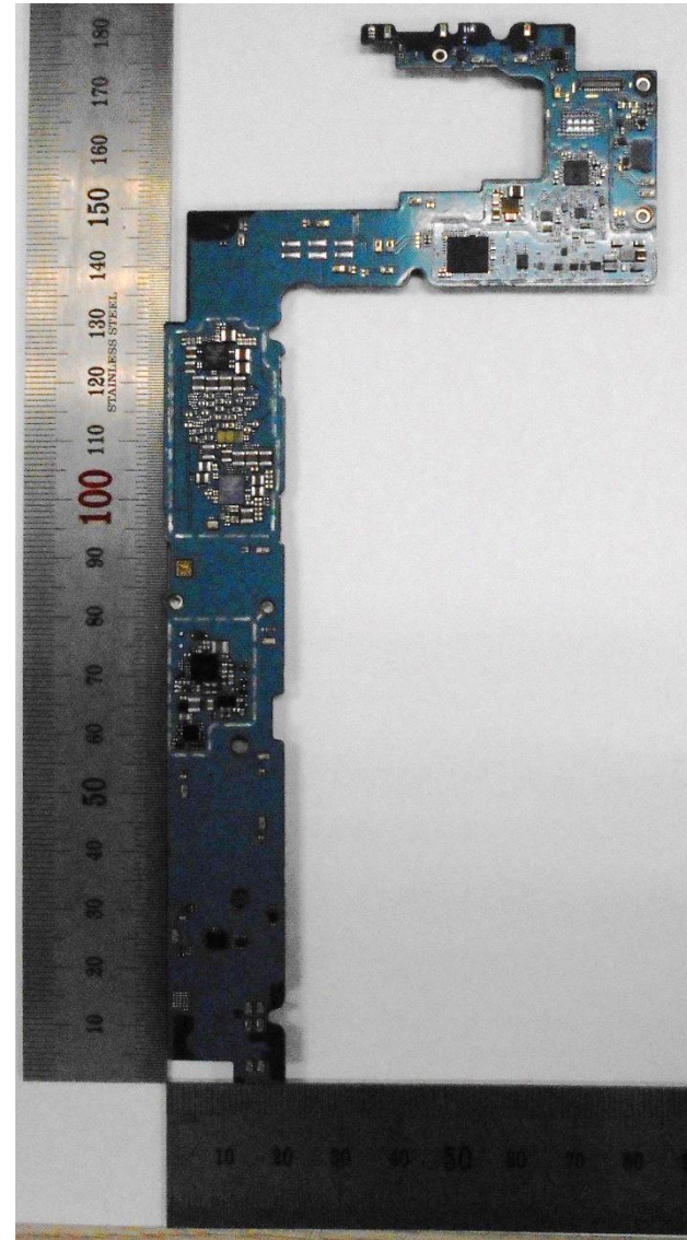
PBA BOT without Shield Can
