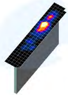
Figure 4-1 Sample SAR Area Scan
