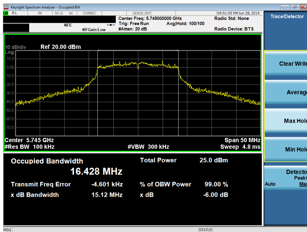
Plot 7-68. 6dB Bandwidth Plot SISO ANT2 (802.11a (UNII Band 3) – Ch. 149)
