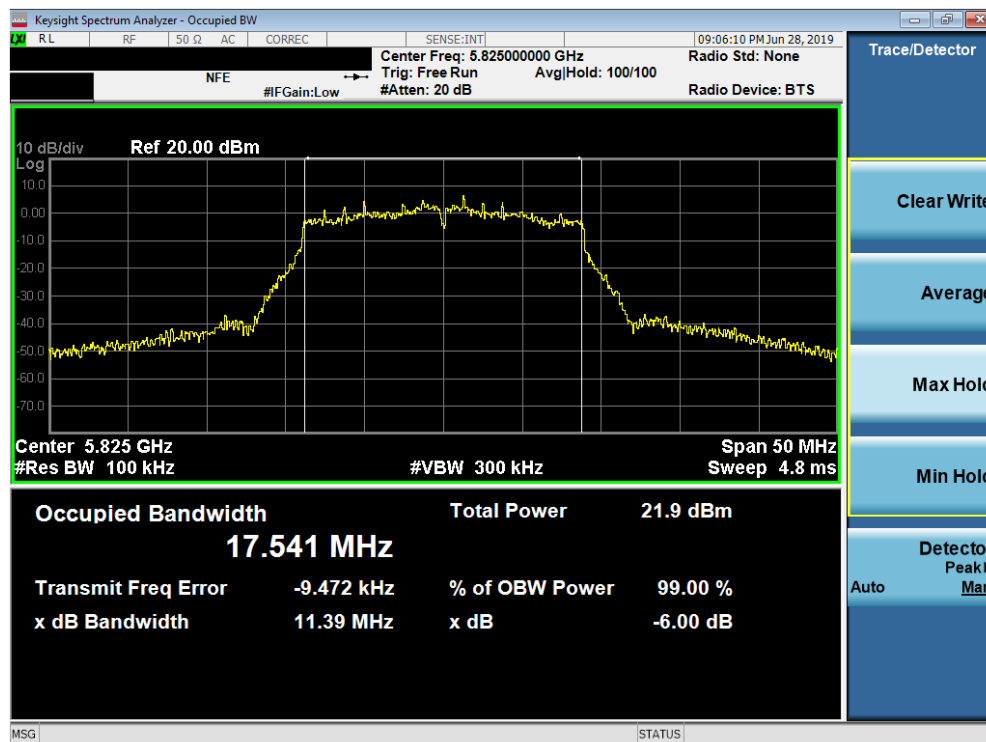
Plot 7-64. 6dB Bandwidth Plot SISO ANT1 (20MHz BW 802.11n (UNII Band 3) – Ch. 165)
