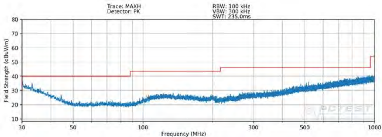
Plot 7-234. Radiated Spurious Plot below 1GHz MIMO (802.11a – U3 Ch. 157)
