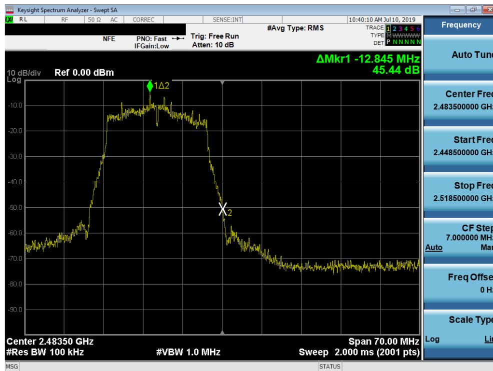
Plot 7-79. Band Edge Plot SISO ANT2 (802.11n (2.4GHz) – Ch. 13)
