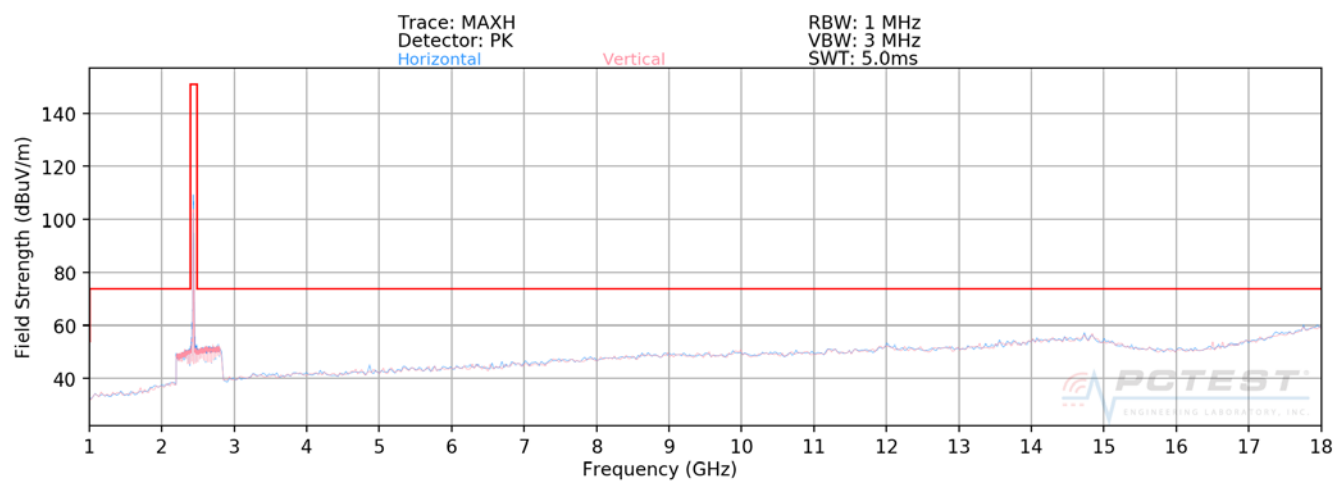
Plot 7-93. Radiated Spurious Plot above 1GHz SISO ANT1 (802.11b – Ch. 6)
