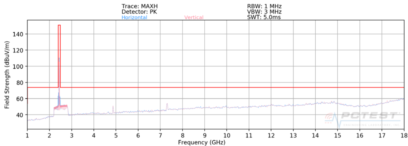
Plot 7-97. Radiated Spurious Plot above 1GHz SISO ANT2 (802.11b – Ch. 6)
