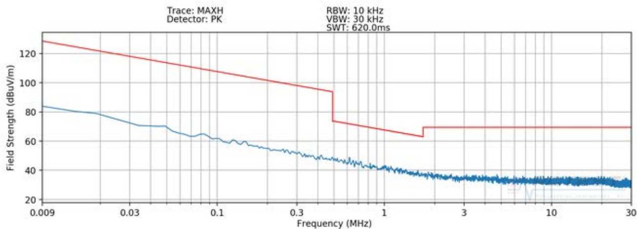
Plot 7-6. Radiated Spurious Plot 9kHz – 30MHz (Pol. Z – Digitizer Mode 1)
