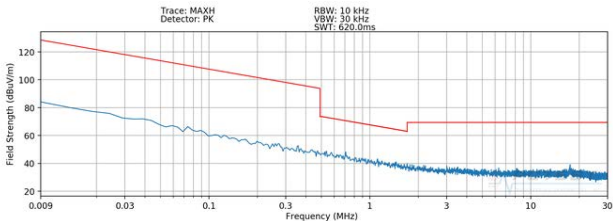
Plot 7-5 Radiated Spurious Plot 9kHz – 30MHz (Pol. Y – Digitizer Mode 1)
