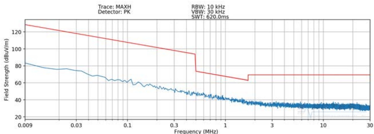
Plot 7-2 Radiated Spurious Plot 9kHz – 30MHz (Pol. Y – Device to S-Pen WPT)
