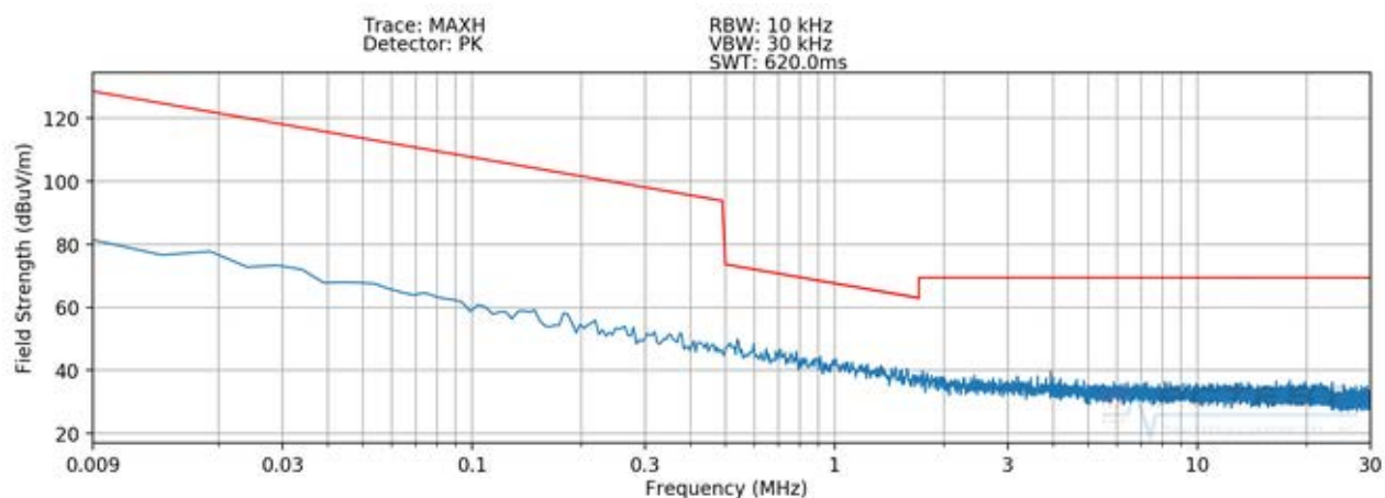
Plot 7-3. Radiated Spurious Plot 9kHz – 30MHz (Pol. Z – Device to S-Pen WPT)
