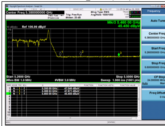
Middle channel_36 RU (Peak)
