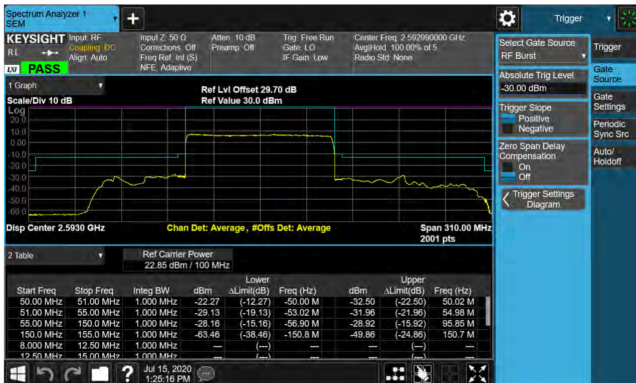
Sub6 n41. Mid Channel Edge Plot (100 MHz Ch.518598 BPSK RB 25)
