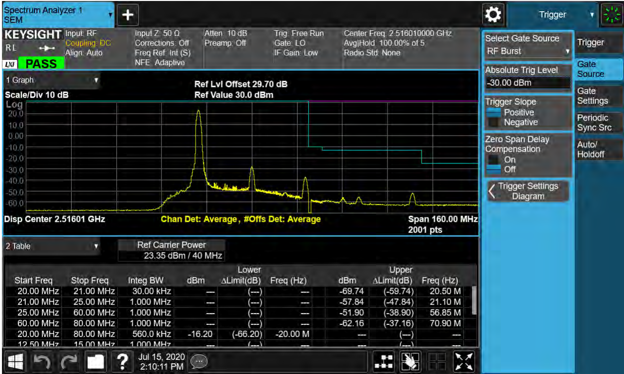
Sub6 n41. Low Channel Edge Plot (40 MHz Ch.503202 BPSK_RB1_Offset 0)-2
