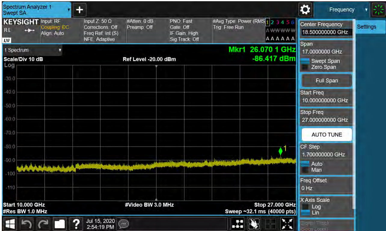
Sub6 n41. Conducted Spurious Plot 2 (50 MHz Ch.504204 BPSK RB 1, Offset 0)
