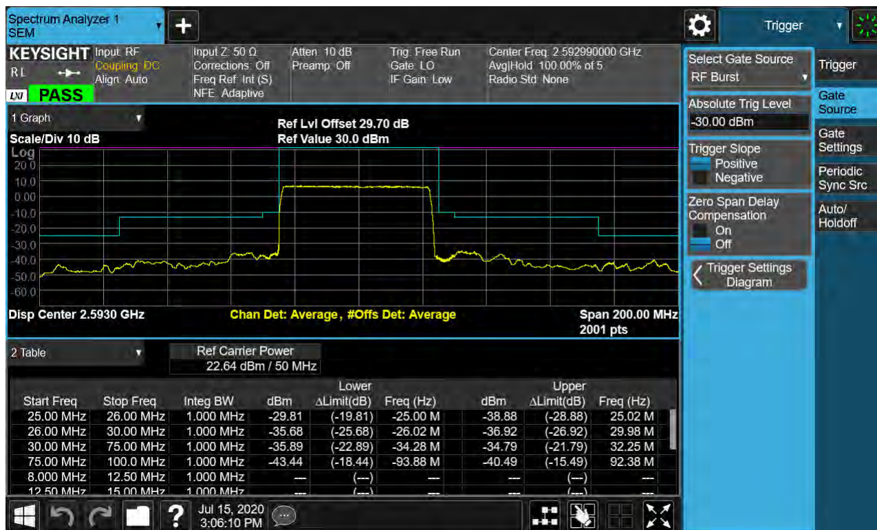
Sub6 n41. Mid Channel Edge Plot (50 MHz Ch.518598 BPSK RB 25)
