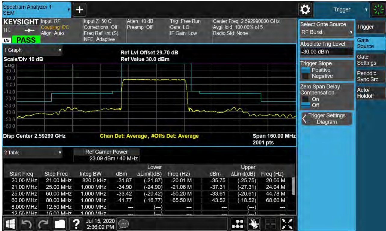
Sub6 n41. Mid Channel Edge Plot (40 MHz Ch.518598 BPSK RB 25)
