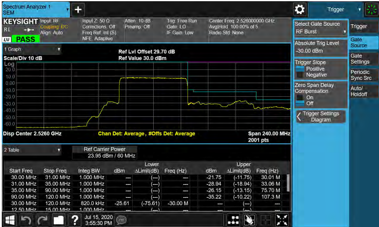
Sub6 n41. Low Channel Edge Plot (60 MHz Ch.505200 BPSK_RB25_Offset 0)-2
