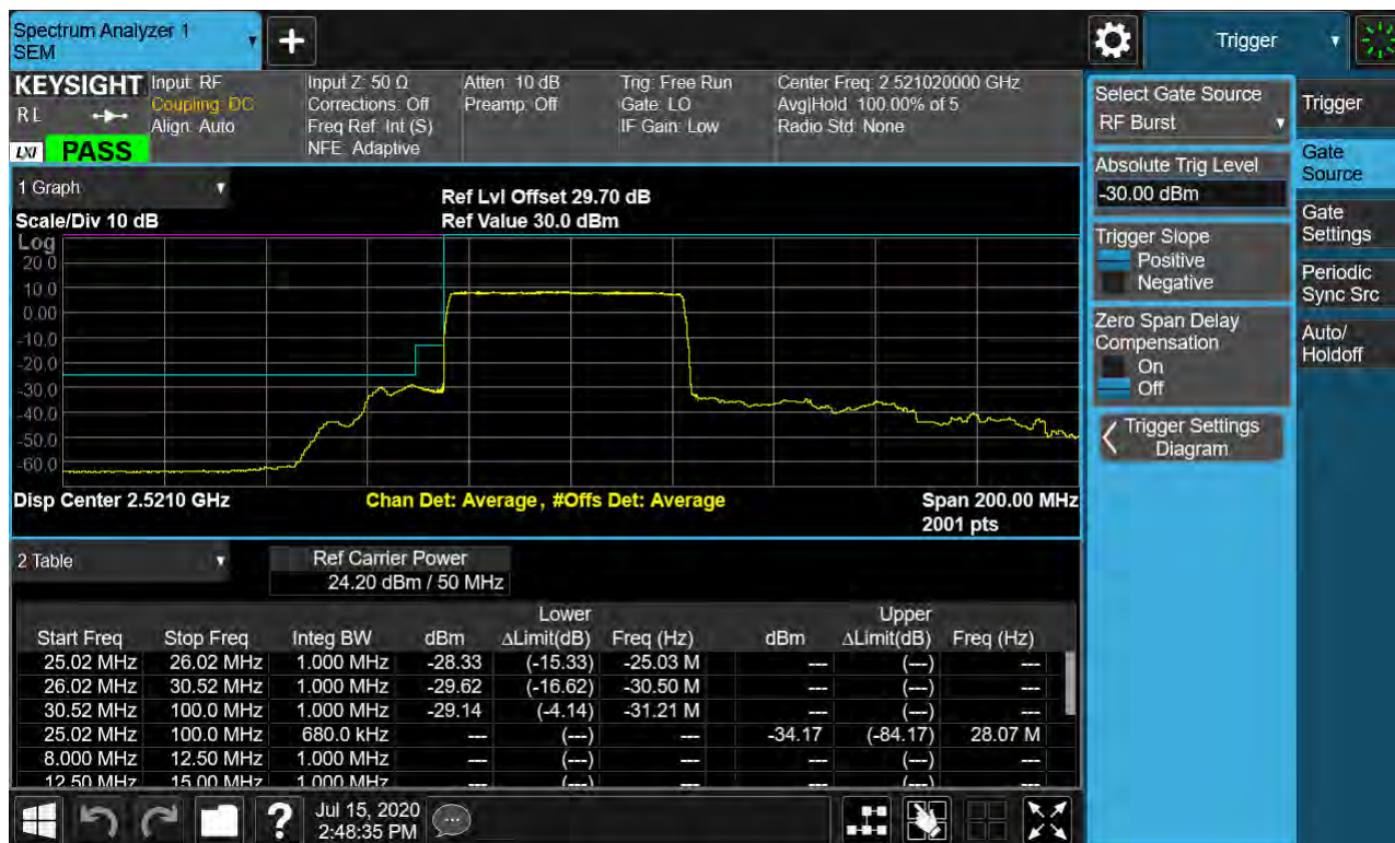
Sub6 n41. Low Channel Edge Plot (50 MHz Ch.504204 BPSK RB 25, Offset 0)-1
