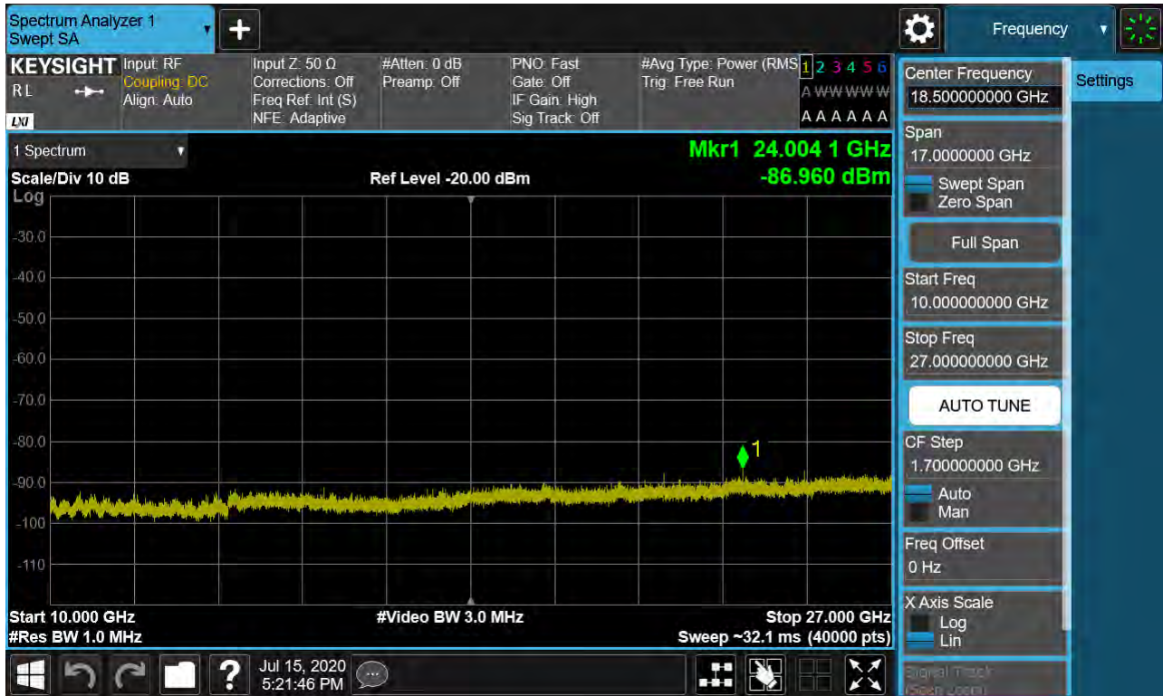
Sub6 n41. Conducted Spurious Plot 2 (80 MHz Ch.529998 BPSK RB 1, Offset 0)
