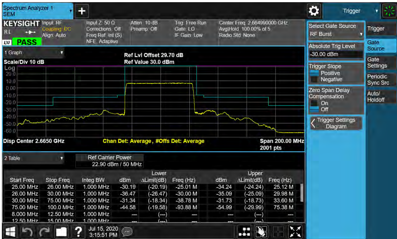
Sub6 n41. High Channel Edge Plot (50 MHz Ch.532998 BPSK_RB25_Offset 0)
