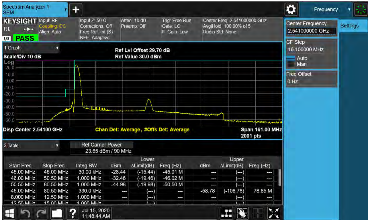
Sub6 n41. Low Channel Edge Plot (90 MHz Ch.508200 BPSK RB 1, Offset 0)-1
