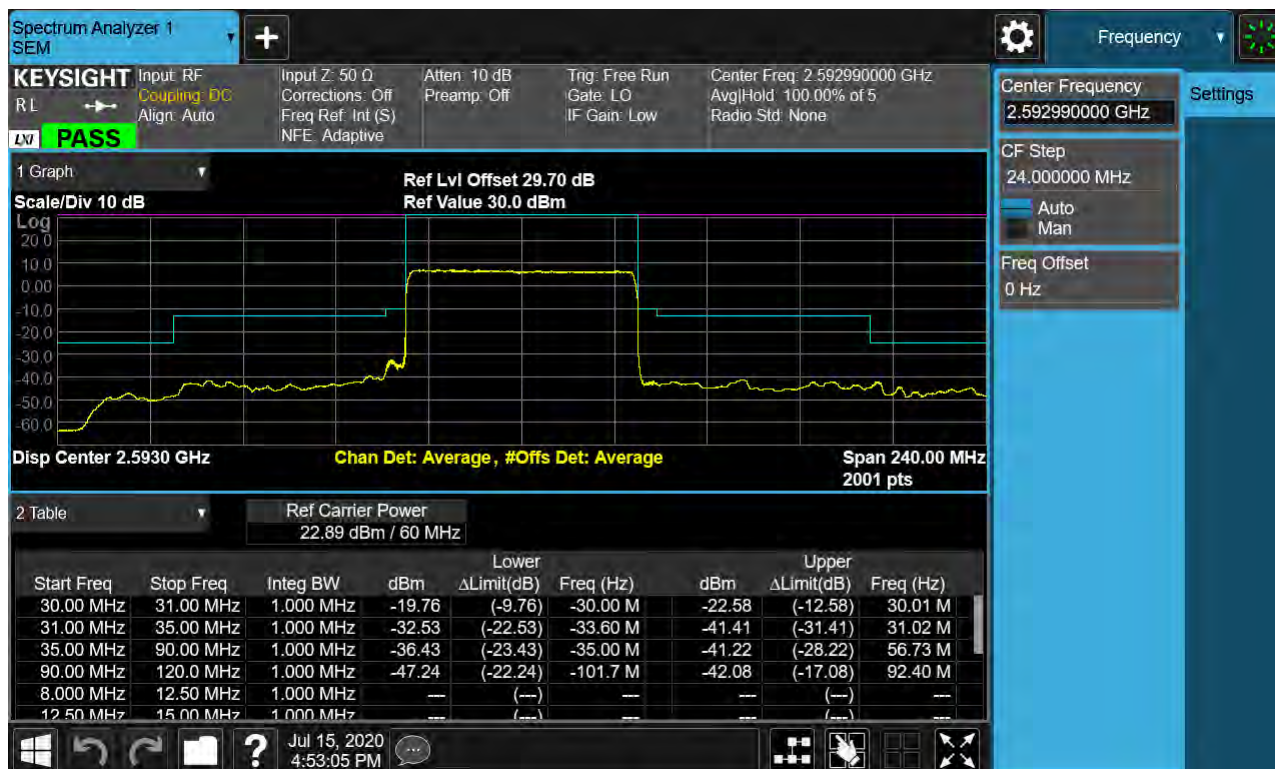
Sub6 n41. Mid Channel Edge Plot (60 MHz Ch.518598 BPSK RB 25)
