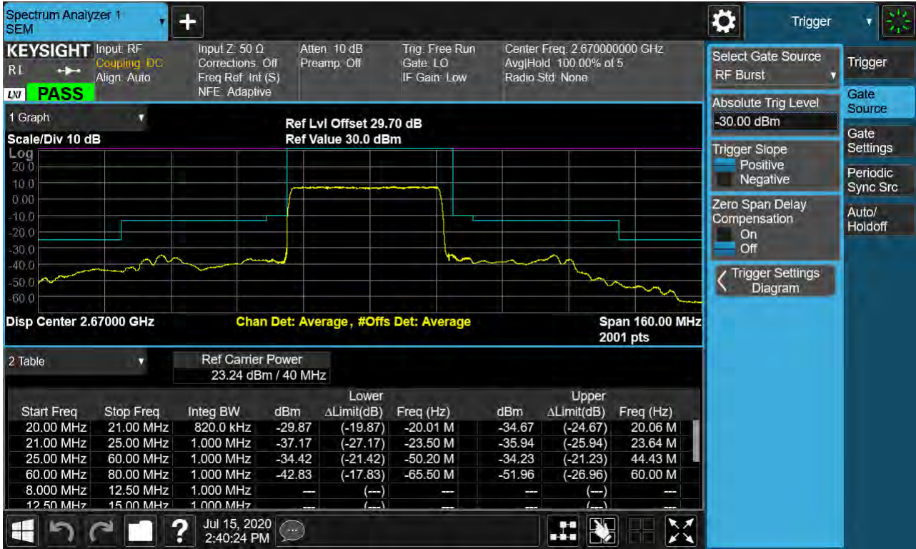
Sub6 n41. High Channel Edge Plot (40 MHz Ch.534000 BPSK_RB25_Offset 0)
