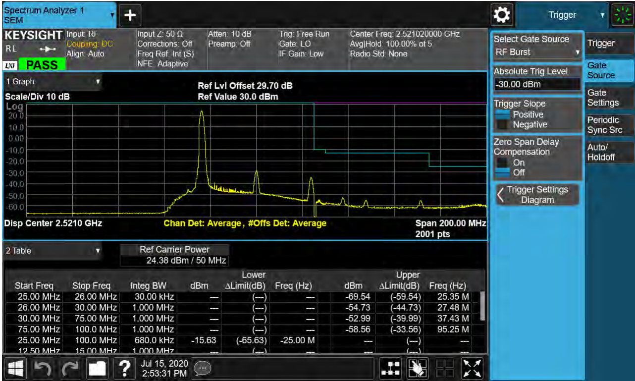
Sub6 n41. Low Channel Edge Plot (50 MHz Ch.504204 BPSK_RB1_Offset 0)-2
