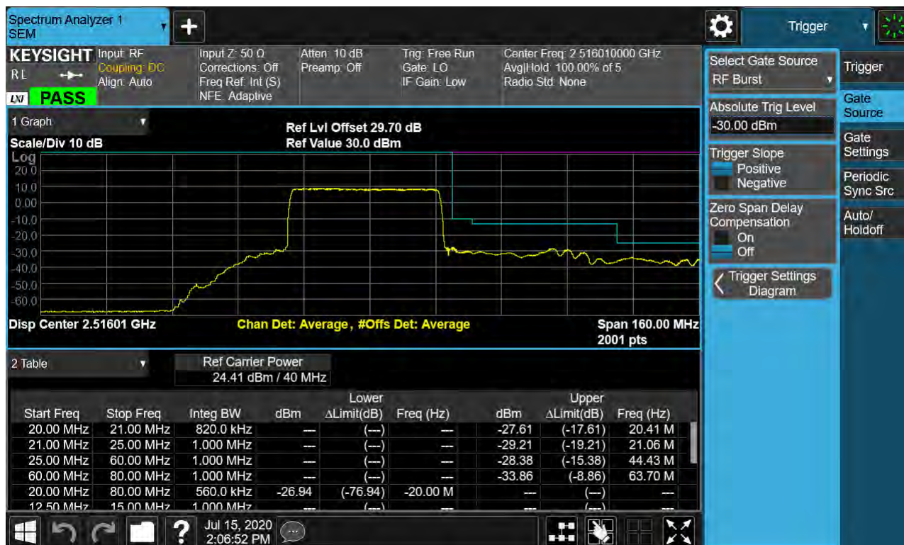
Sub6 n41. Low Channel Edge Plot (40 MHz Ch.503202 BPSK_RB25_Offset 0)-2
