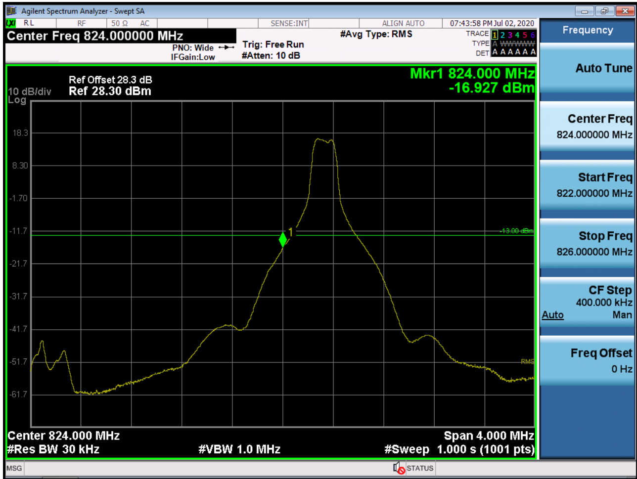
Sub6 n5. Lower Band Edge Plot (5M BW Ch.165300 BPSK_RB1_Offset 0)
