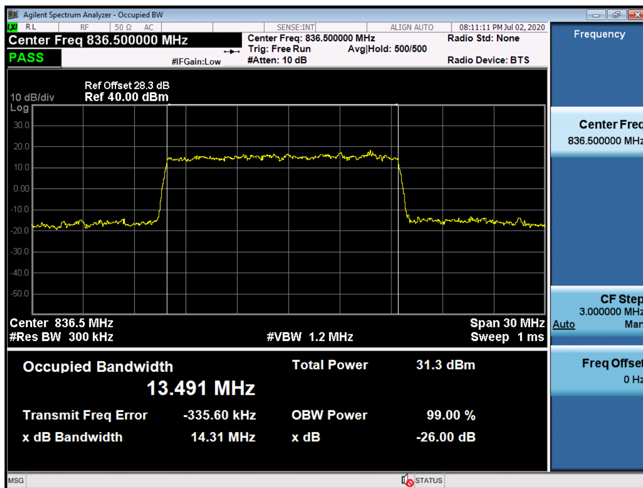
Sub6 n5. Occupied Bandwidth Plot (15M BW Ch.167300 QPSK_RB25_0)
