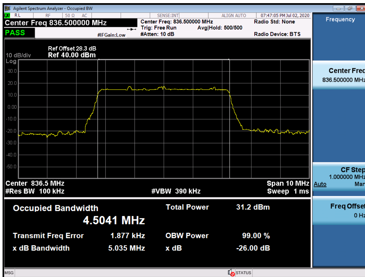
Sub6 n5. Occupied Bandwidth Plot (5M BW Ch.167300 16QAM_RB6_0)
