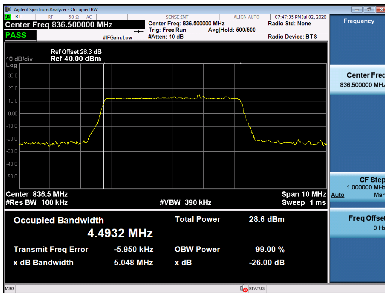
Sub6 n5. Occupied Bandwidth Plot (5M BW Ch.167300 256QAM_RB6_0)
