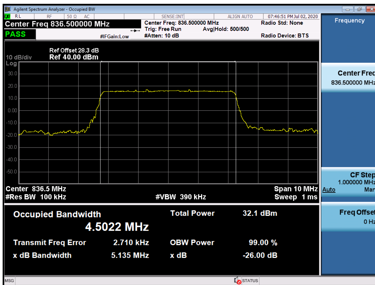
Sub6 n5. Occupied Bandwidth Plot (5M BW Ch.167300 QPSK_RB6_0)
