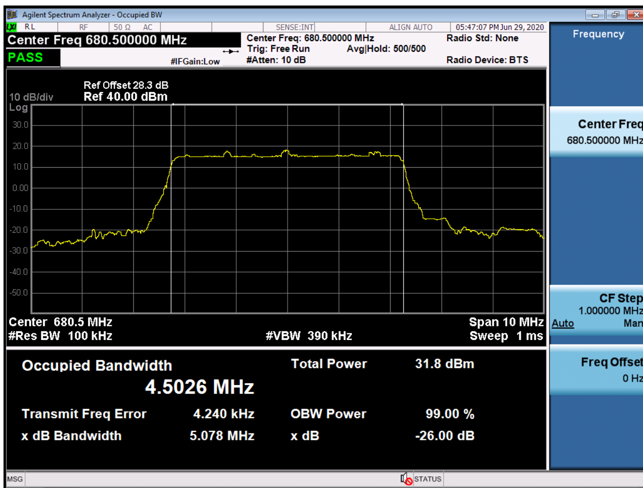
Sub6 n71. Occupied Bandwidth Plot (5M BW Ch.136100 16QAM_RB6_0)
