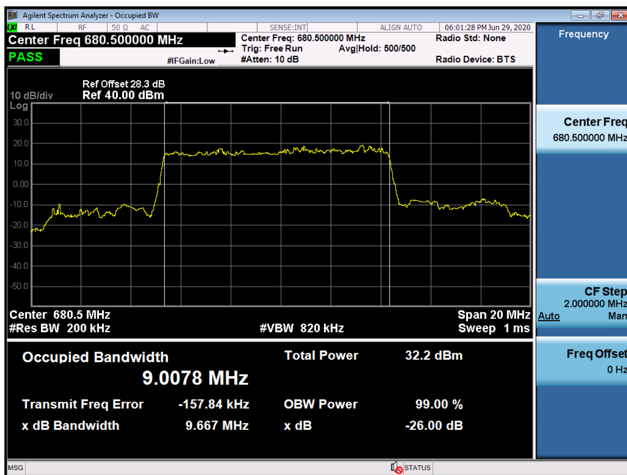
Sub6 n71. Occupied Bandwidth Plot (10M BW Ch.136100 BPSK_RB15_0)
