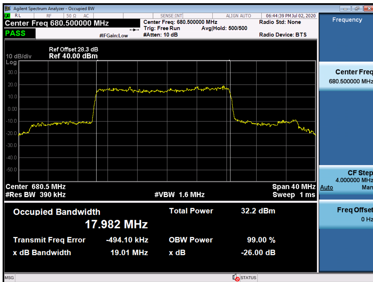
Sub6 n71. Occupied Bandwidth Plot (20M BW Ch.136100 BPSK_RB50_0)
