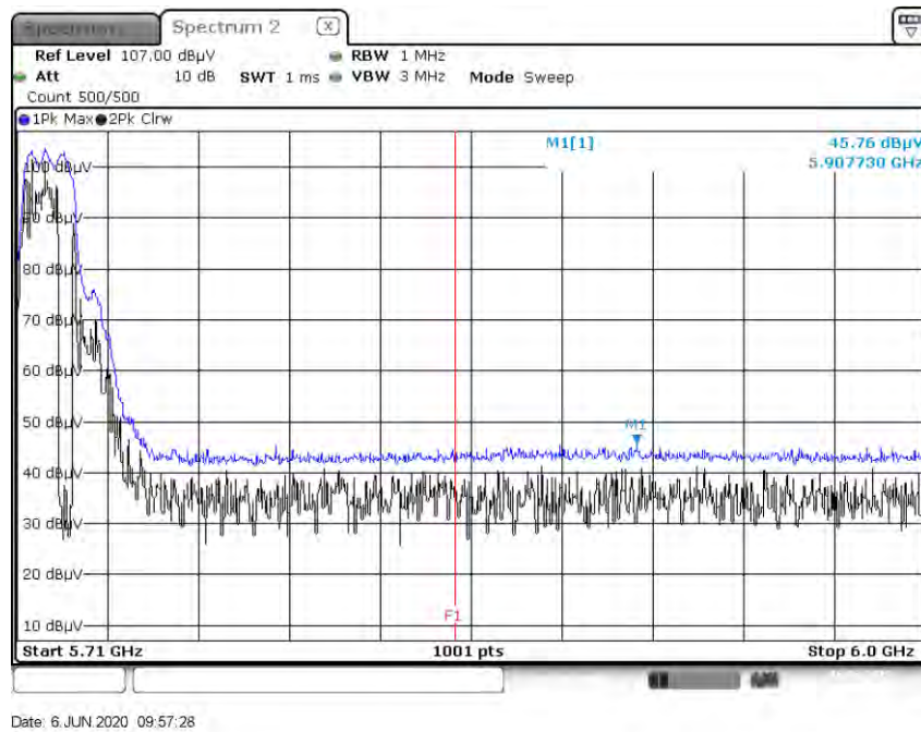
Peak Reading (802.11n_HT20, Ch.144, Z-H)
