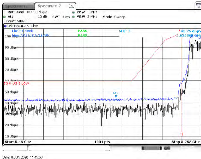
Peak Reading (802.11n_HT20, Ch.149, Z-H)
