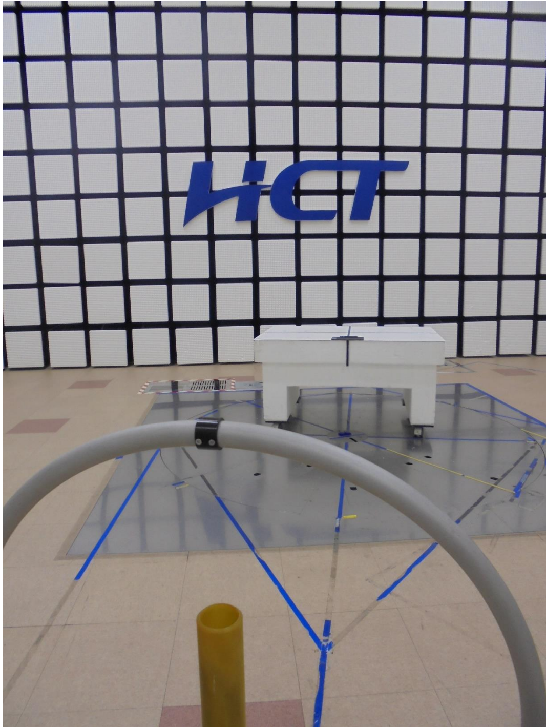
S-Pen Radiated Test Setup Photo for below 30 MHz:
