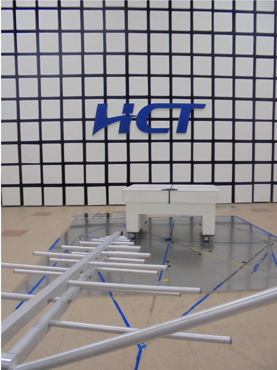
S-Pen Radiated Test Setup Photo for 30 MHz ~ 1 GHz :
