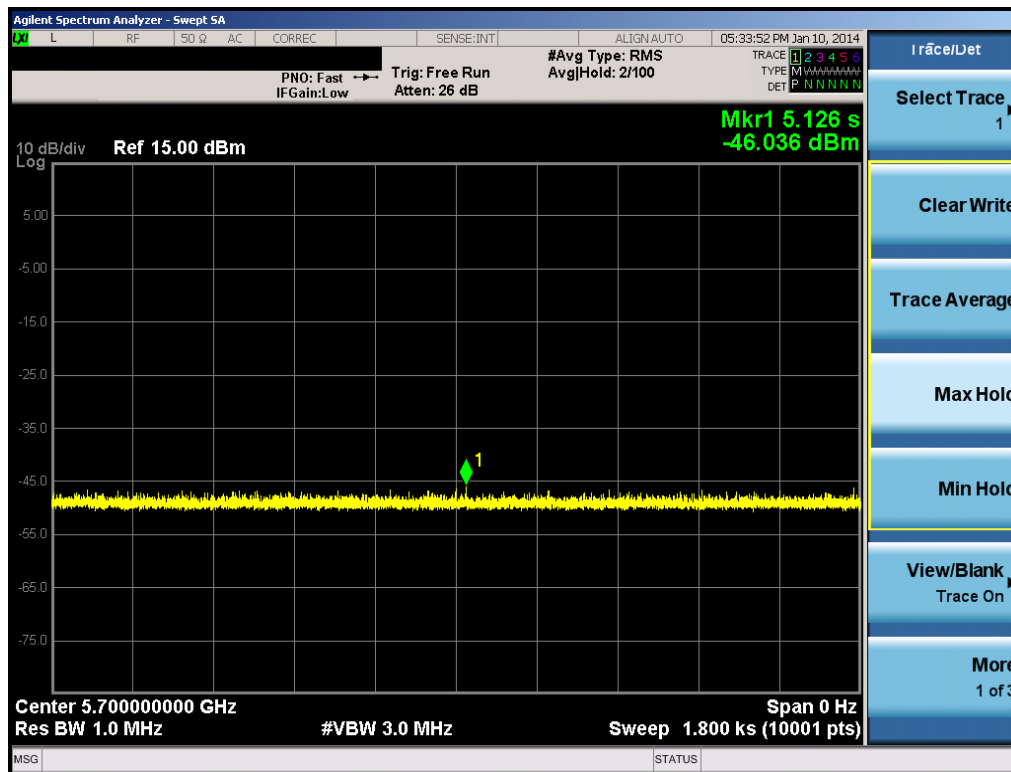
Figure 6-6. Non-occupancy Period - Monitoring live spectrum - Elapse time 30 minutes
