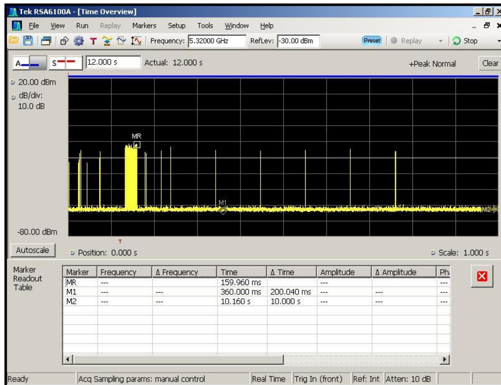
Figure 5-5. Channel Move Time (< 1sec)
