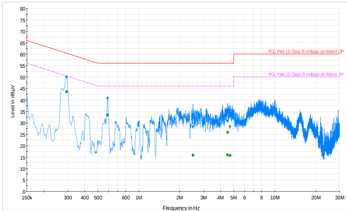
Plot 6-7. Line Conducted Plot with ANT+ (N)
