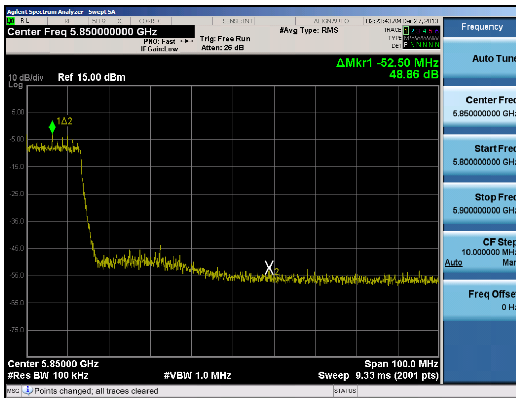
Plot 6-84. Band Edge Plot (40MHz BW 802.11n (5.8GHz) – Ch. 159)
