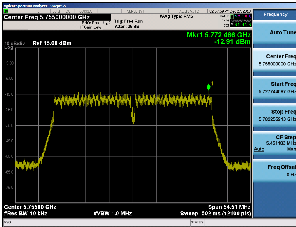
Plot 6-70. Power Spectral Density Plot (40MHz BW 802.11n (5.8GHz) – Ch. 151)
