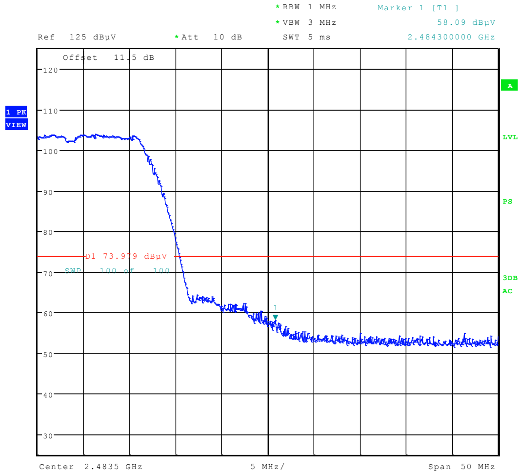
Plot 6-128. Radiated Restricted Upper Band Edge Measurement (Peak)
