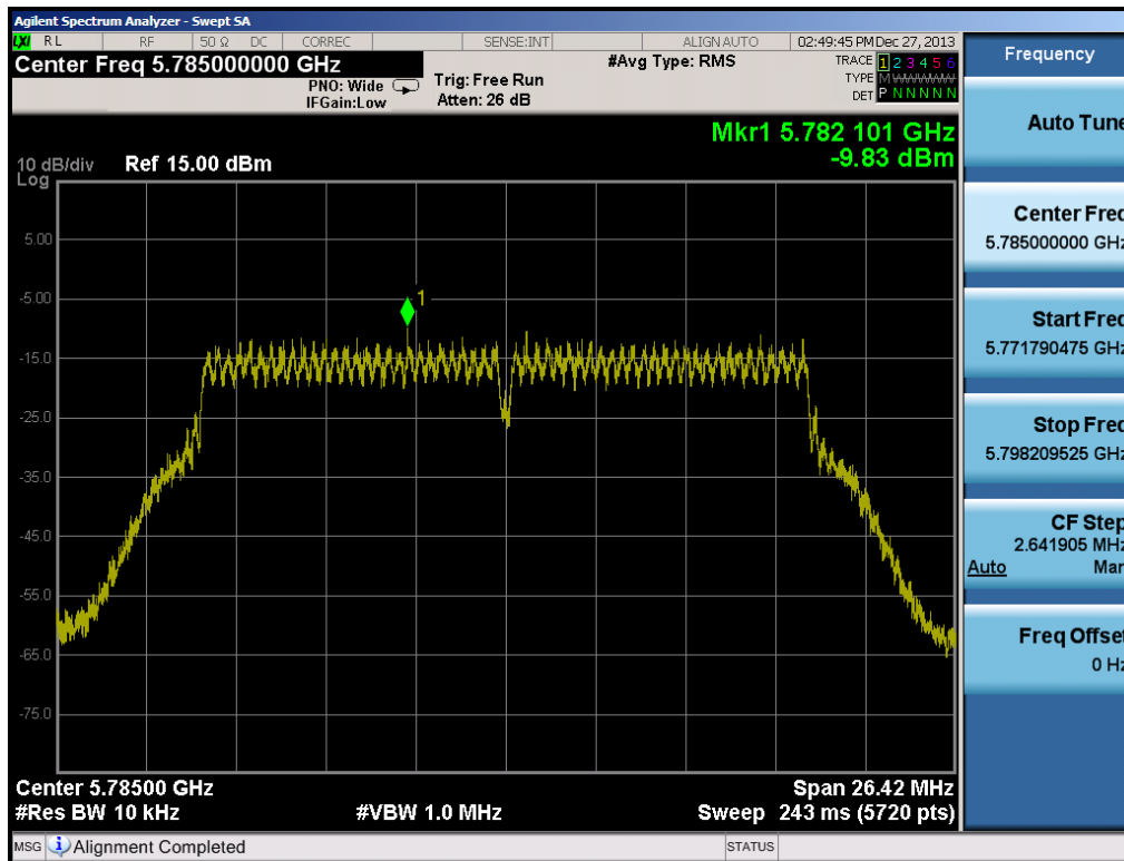
Plot 6-68. Power Spectral Density Plot (20MHz BW 802.11n (5.8GHz) – Ch. 157)
