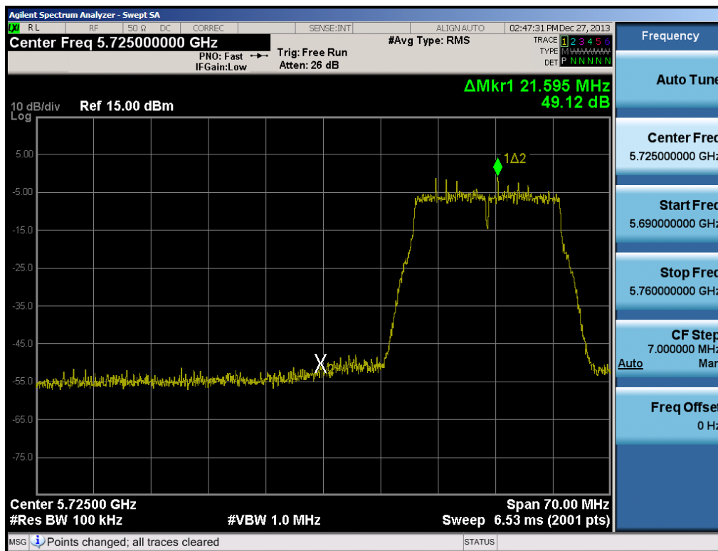
Plot 6-95. Band Edge Plot (20MHz BW 802.11n (5.8GHz) – Ch. 149)
