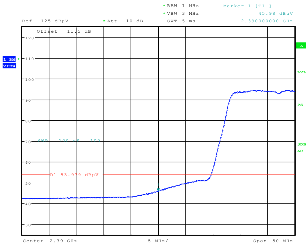
Plot 6-133. Radiated Restricted Lower Band Edge Measurement (Average)
