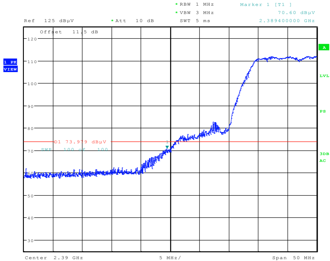
Plot 6-130. Radiated Restricted Lower Band Edge Measurement (Peak)
