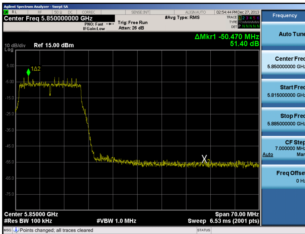
Plot 6-96. Band Edge Plot (20MHz BW 802.11n (5.8GHz) – Ch. 165)
