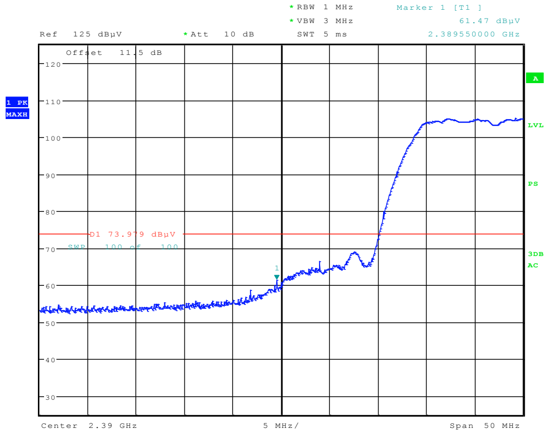
Plot 6-126. Radiated Restricted Lower Band Edge Measurement (Peak)
