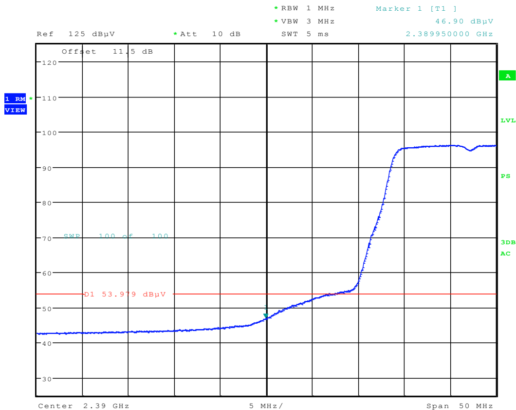
Plot 6-125. Radiated Restricted Lower Band Edge Measurement (Average)
