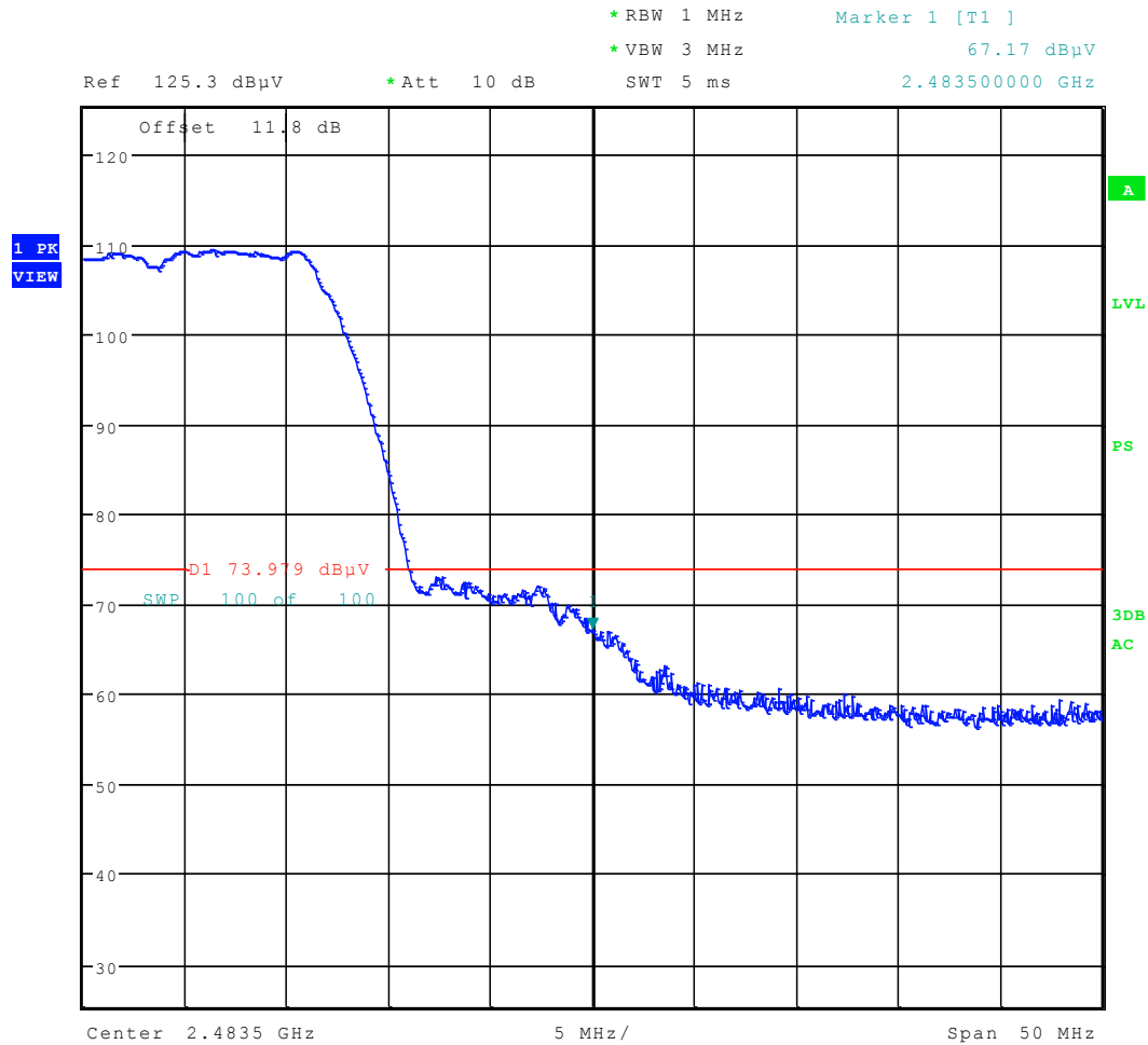
Plot 6-132. Radiated Restricted Upper Band Edge Measurement (Peak)
