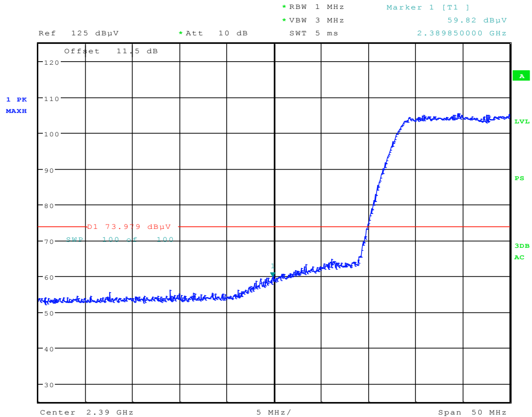
Plot 6-134. Radiated Restricted Lower Band Edge Measurement (Peak)
