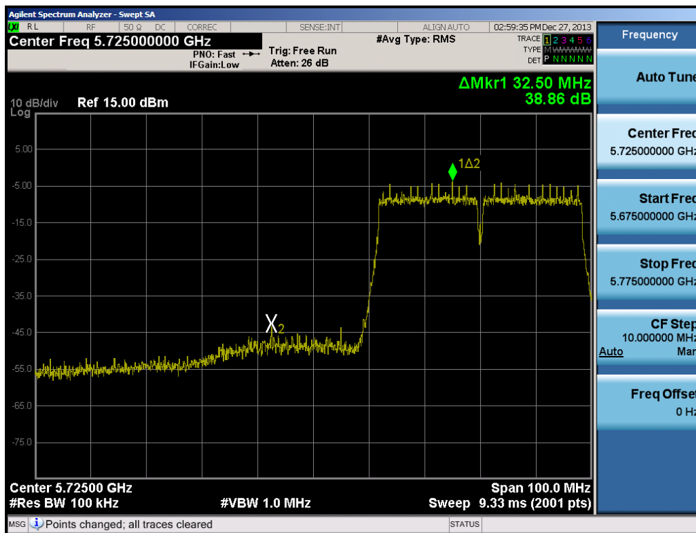
Plot 6-97. Band Edge Plot (40MHz BW 802.11n (5.8GHz) – Ch. 151)
