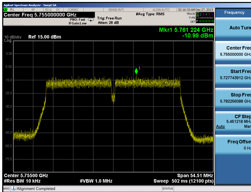
Plot 6-52. Power Spectral Density Plot (40MHz BW 802.11n (5.8GHz) – Ch. 151)
