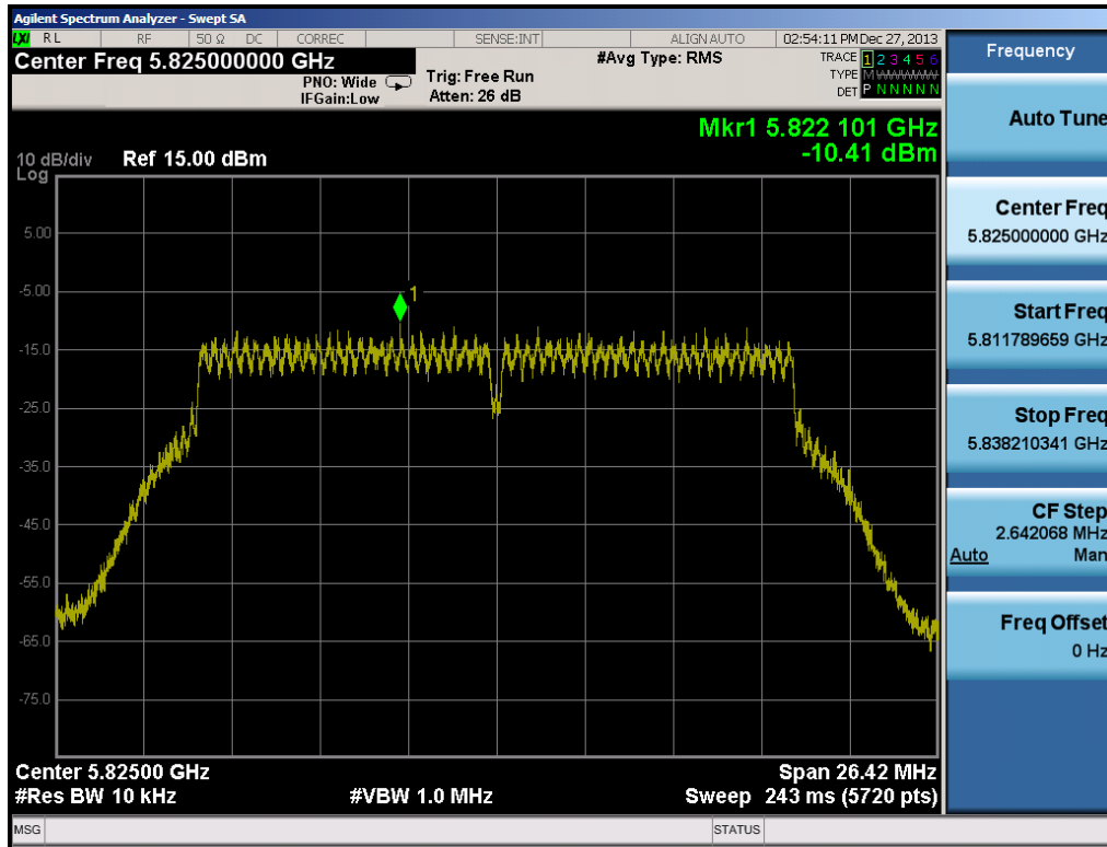
Plot 6-69. Power Spectral Density Plot (20MHz BW 802.11n (5.8GHz) – Ch. 165)
