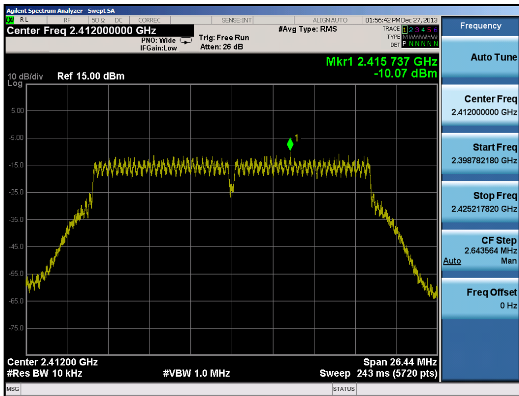
Plot 6-61. Power Spectral Density Plot (802.11n (2.4GHz) – Ch. 1)
