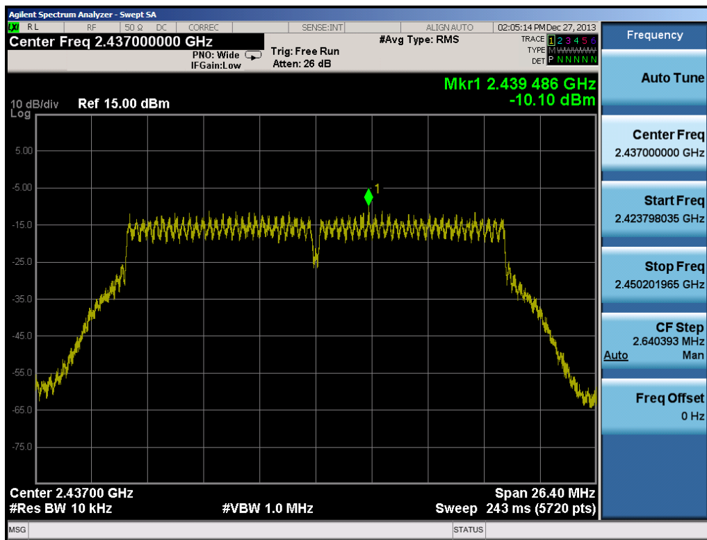
Plot 6-62. Power Spectral Density Plot (802.11n (2.4GHz) – Ch. 6)
