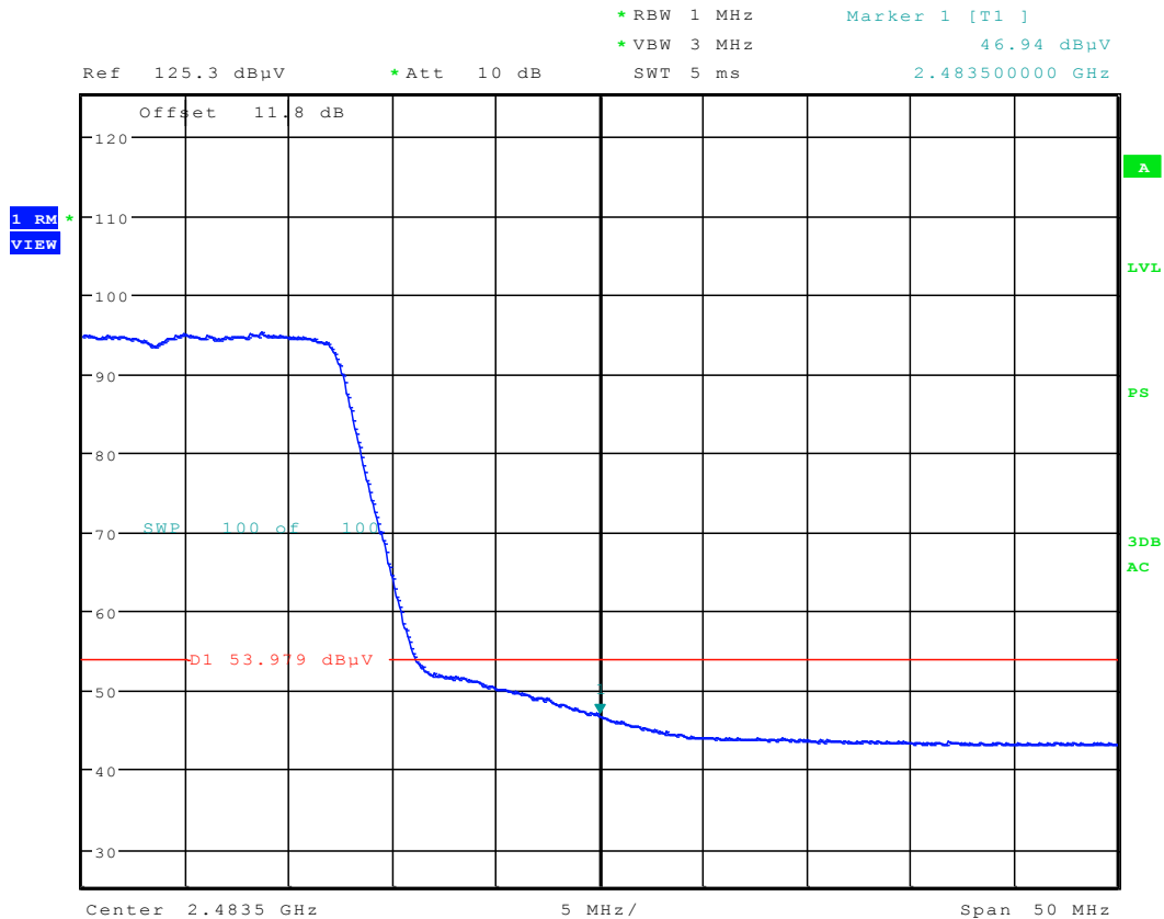
Plot 6-135. Radiated Restricted Upper Band Edge Measurement (Average)
