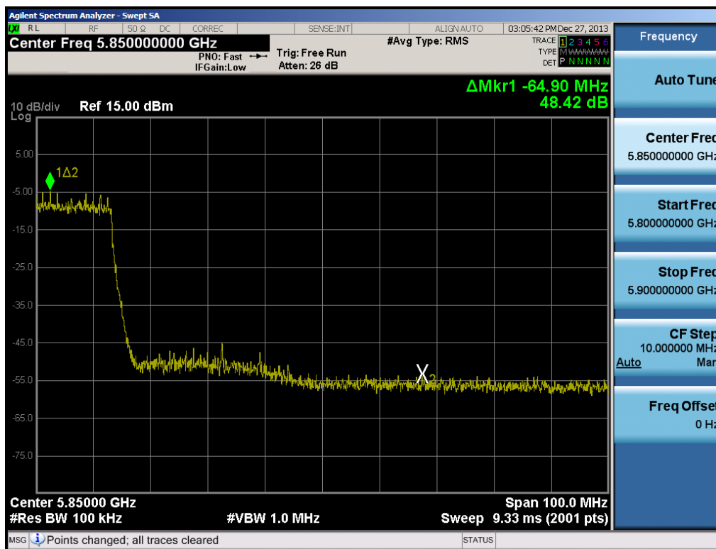
Plot 6-98. Band Edge Plot (40MHz BW 802.11n (5.8GHz) – Ch. 159)
