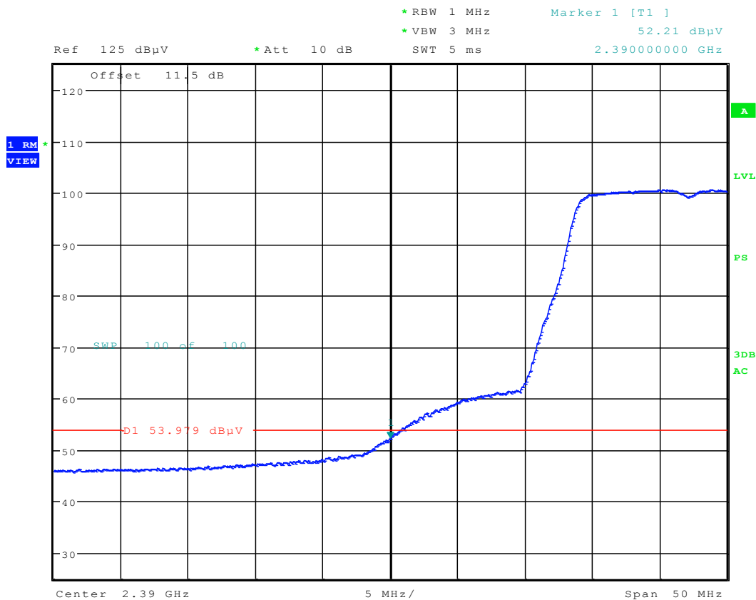
Plot 6-129. Radiated Restricted Lower Band Edge Measurement (Average)
