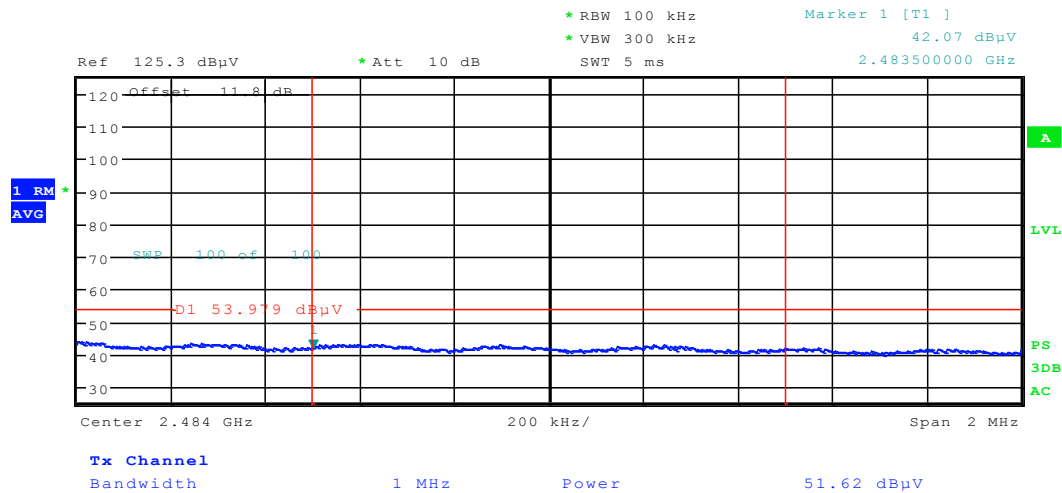
Plot 6-131. Radiated Restricted Upper Band Edge Measurement (Average)
