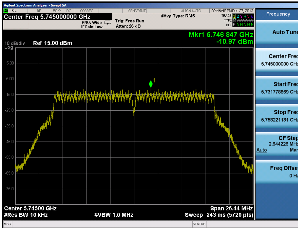
Plot 6-67. Power Spectral Density Plot (20MHz BW 802.11n (5.8GHz) – Ch. 149)
