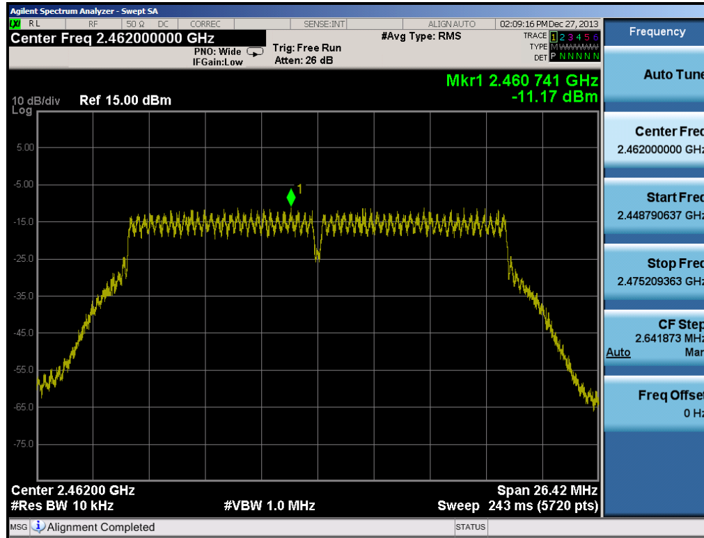
Plot 6-63. Power Spectral Density Plot (802.11n (2.4GHz) – Ch. 11)
