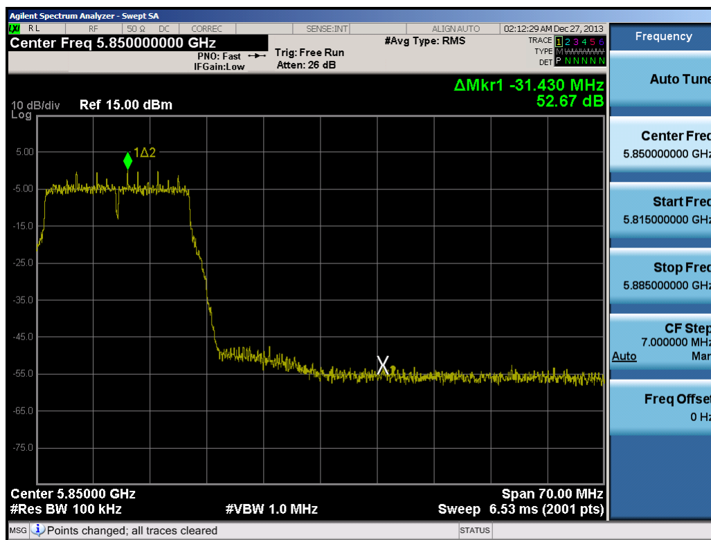
Plot 6-82. Band Edge Plot (20MHz BW 802.11n (5.8GHz) – Ch. 165)
