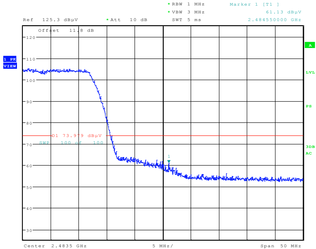
Plot 6-136. Radiated Restricted Upper Band Edge Measurement (Peak)
