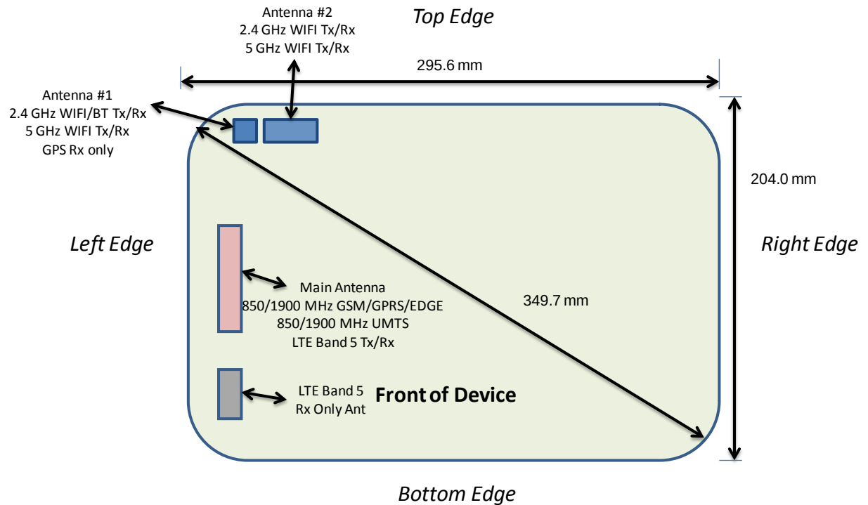
Figure 1-1 DUT Antenna Locations
