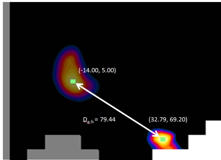
Figure 11-1 Peak SAR Locations of 2.4 GHz WLAN Antenna 1 and GPRS 850 MHz
