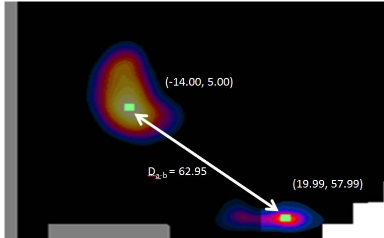
Figure 11-5 Peak SAR Location of 5 GHz WLAN Antenna 1 and GPRS 850 MHz
