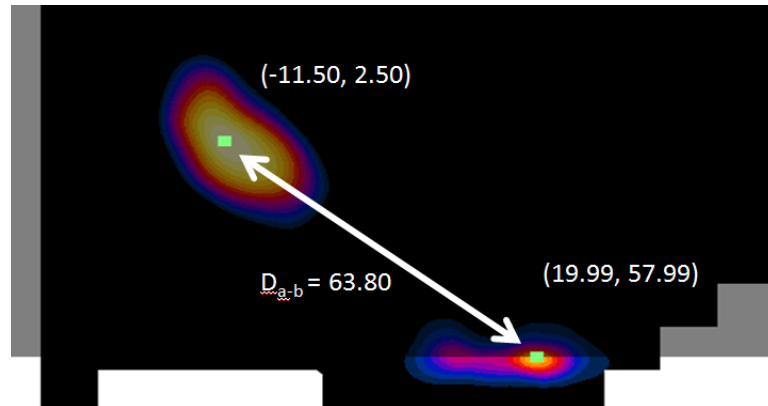
Figure 11-6 Peak SAR Location of 5 GHz WLAN Antenna 1 and GPRS 850 MHz
