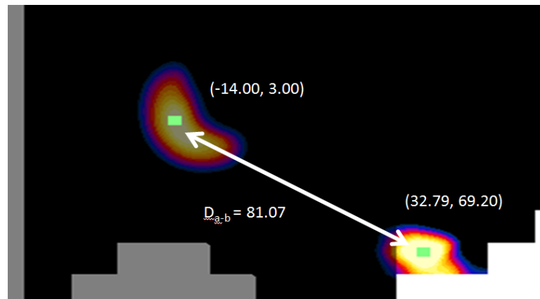
Figure 11-2 Peak SAR Locations of 2.4 GHz WLAN Antenna 1 and UMTS 850 MHz
