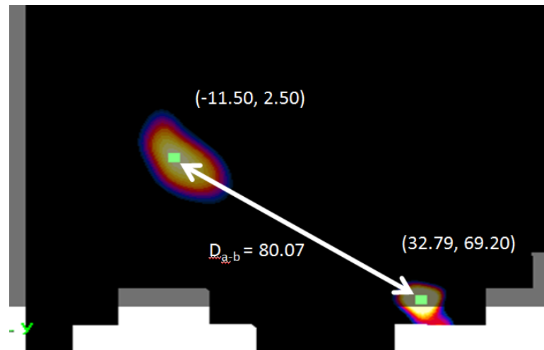
Figure 11-3 Peak SAR Locations of 2.4 GHz WLAN Antenna 1 and GPRS 850 MHz
