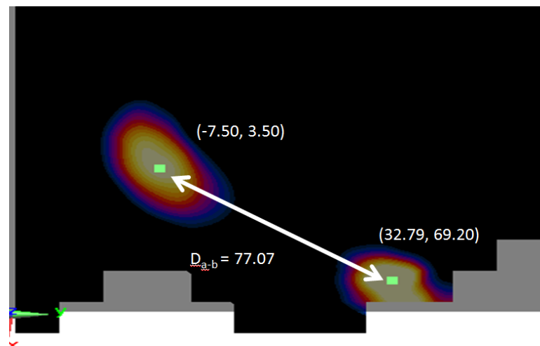
Figure 11-4 Peak SAR Locations of 2.4 GHz WLAN Antenna 1 and UMTS 850 MHz
