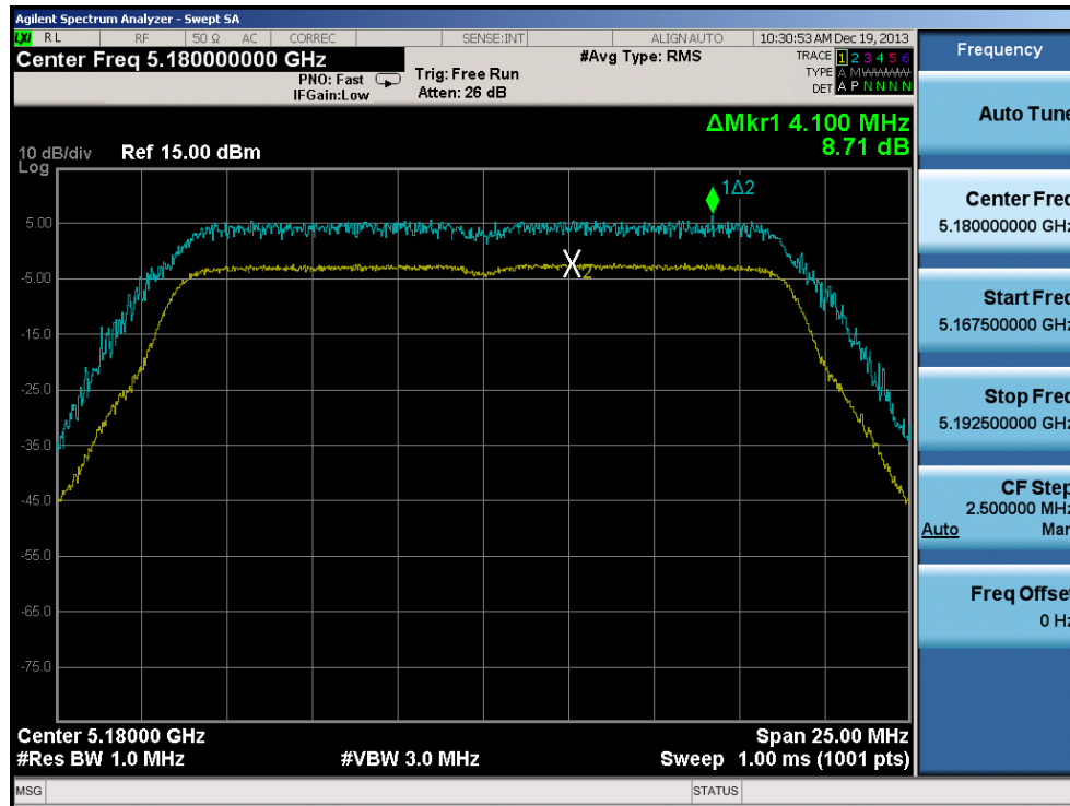
Plot 6-120. Peak Excursion Ratio Plot (20MHz BW 802.11n)
