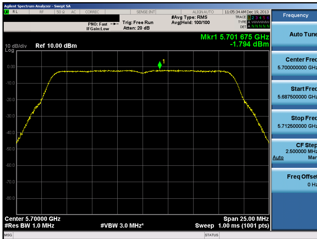
Plot 6-114. Peak Power Spectral Density Plot (20MHz BW 802.11n (UNII Band 2C) – Ch. 140)
