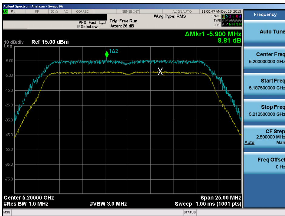
Plot 6-124. Peak Excursion Ratio Plot (20MHz BW 802.11n)
