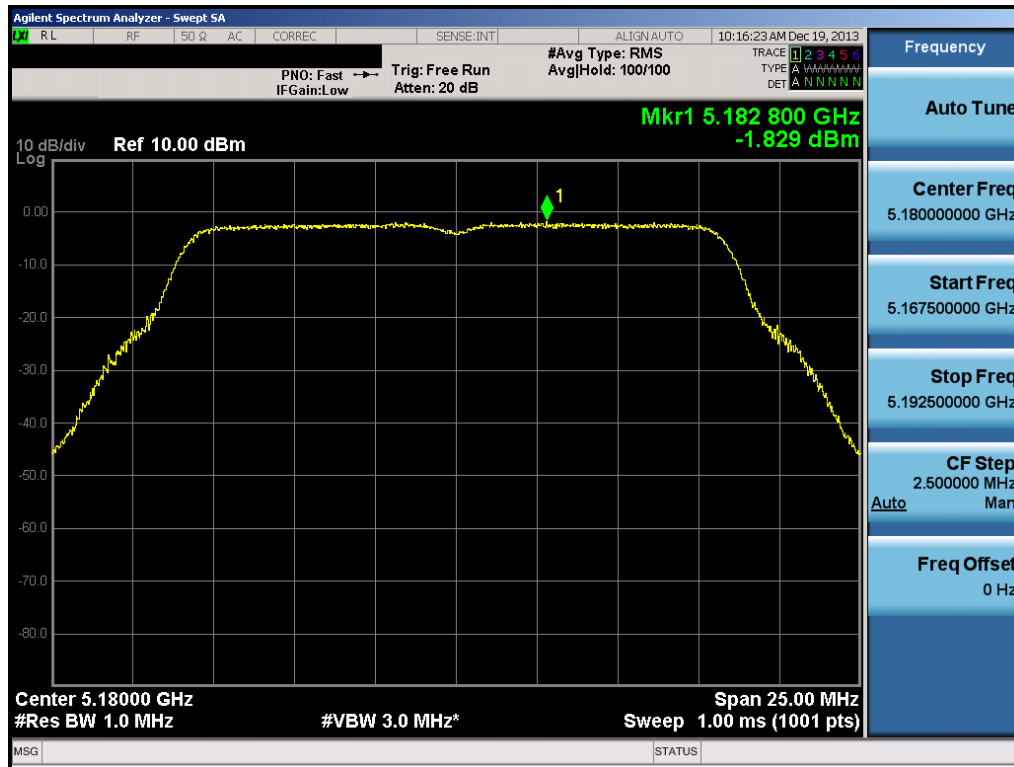
Plot 6-63. Peak Power Spectral Density Plot (802.11a (UNII Band 1) – Ch. 36)
