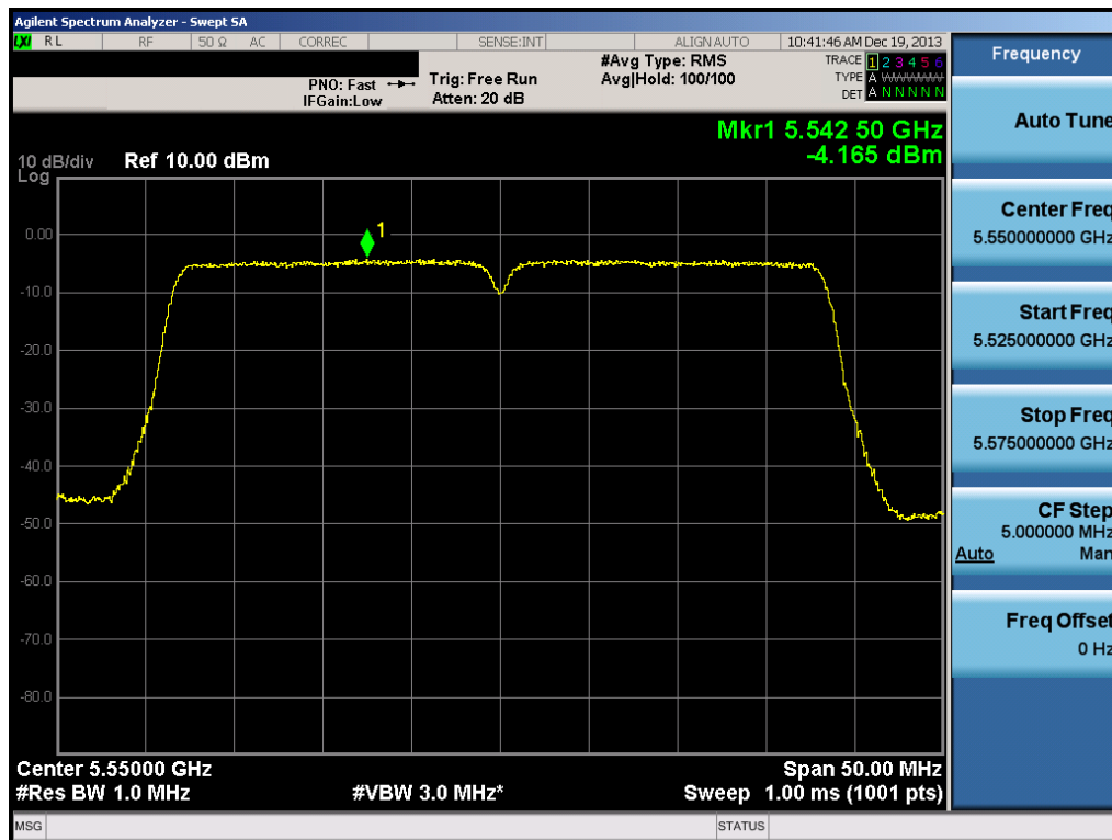
Plot 6-88. Peak Power Spectral Density Plot (40MHz BW 802.11n (UNII Band 2C) – Ch. 110)
