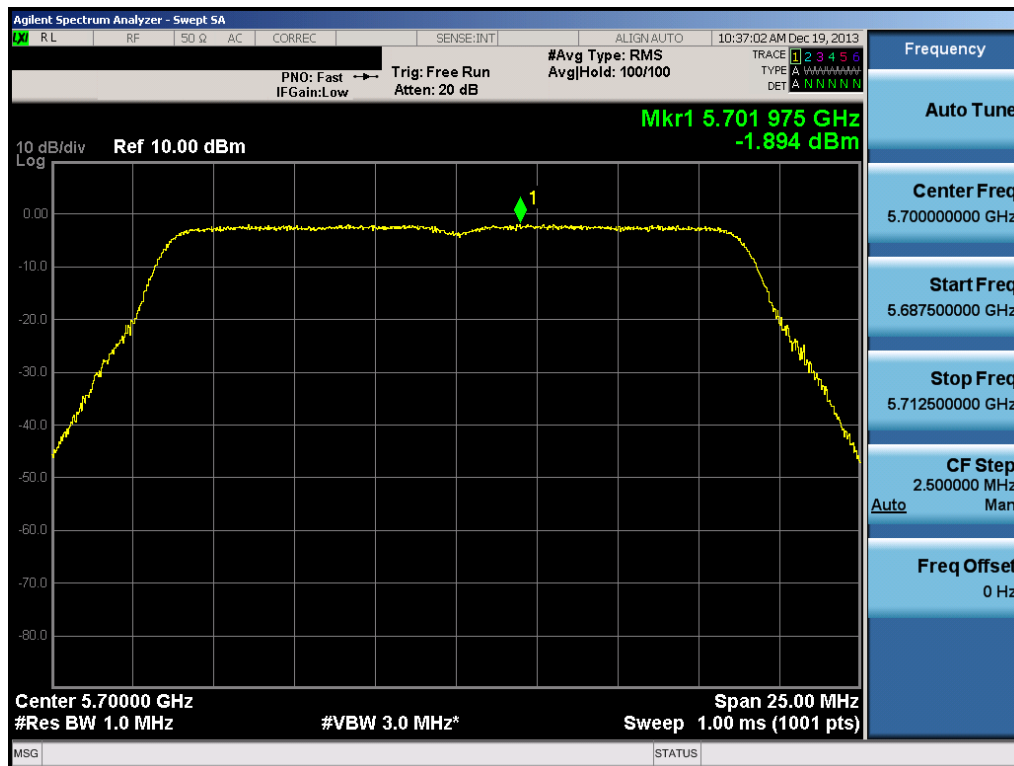
Plot 6-86. Peak Power Spectral Density Plot (20MHz BW 802.11n (UNII Band 2C) – Ch. 140)
