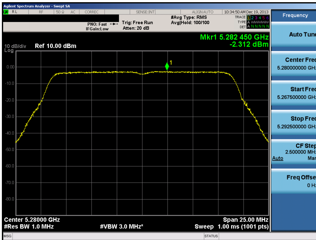
Plot 6-76. Peak Power Spectral Density Plot (20MHz BW 802.11n (UNII Band 2A) – Ch. 56)
