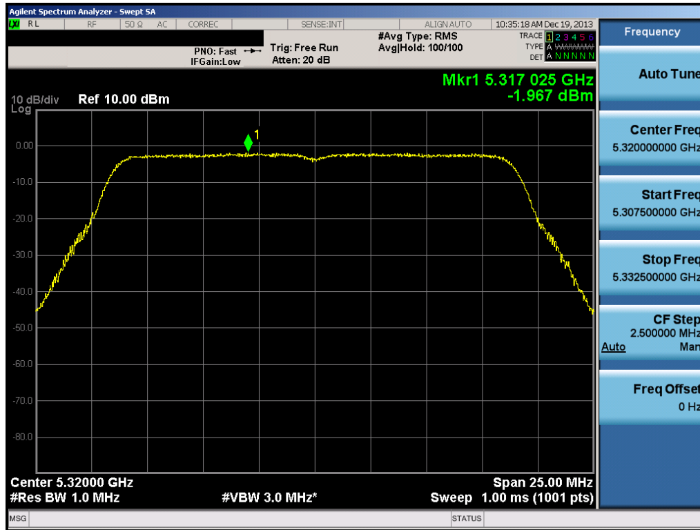
Plot 6-77. Peak Power Spectral Density Plot (20MHz BW 802.11n (UNII Band 2A) – Ch. 64)
