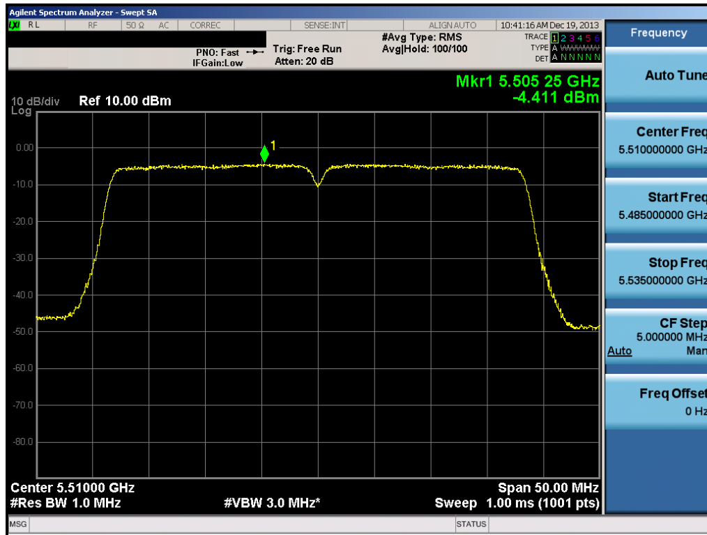
Plot 6-87. Peak Power Spectral Density Plot (40MHz BW 802.11n (UNII Band 2C) – Ch. 102)
