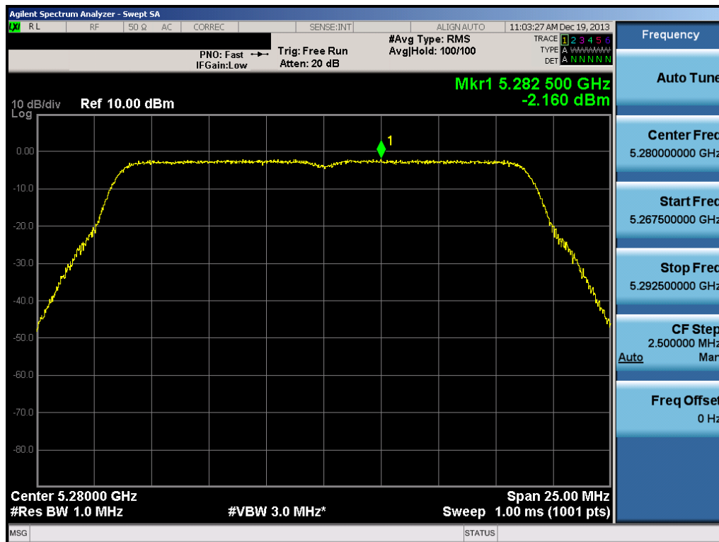
Plot 6-104. Peak Power Spectral Density Plot (20MHz BW 802.11n (UNII Band 2A) – Ch. 56)
