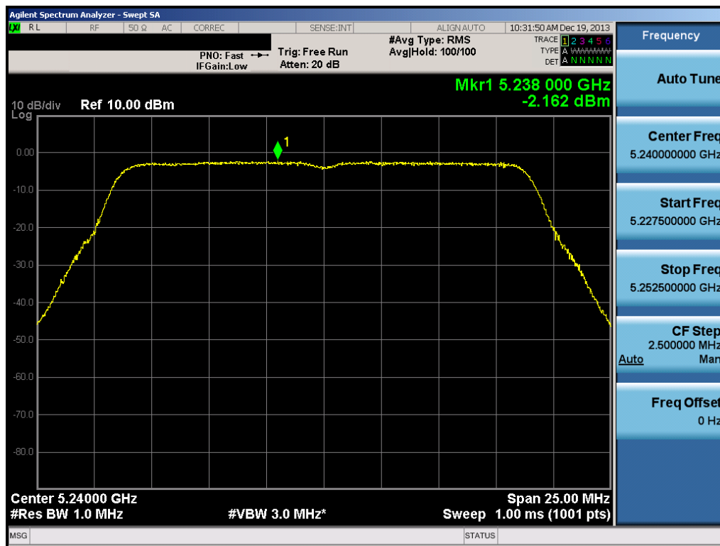
Plot 6-68. Peak Power Spectral Density Plot (20MHz BW 802.11n (UNII Band 1) – Ch. 48)
