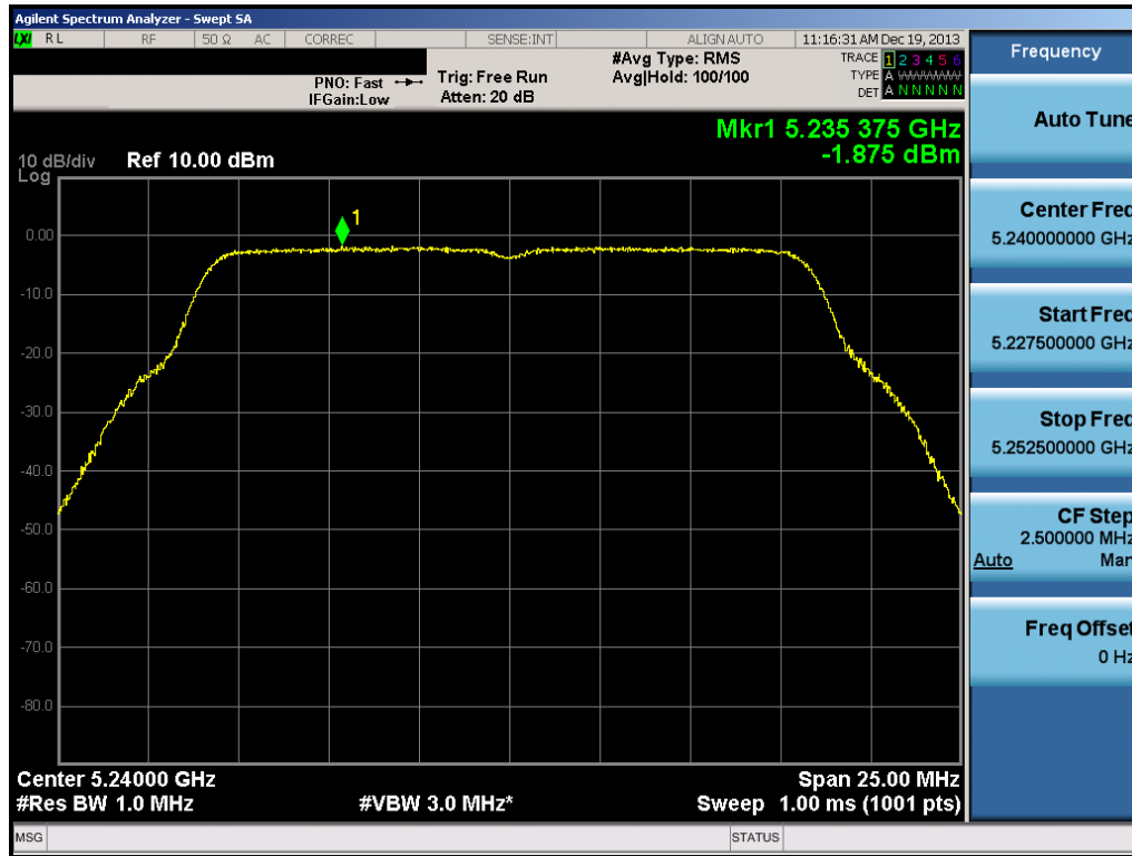
Plot 6-93. Peak Power Spectral Density Plot (802.11a (UNII Band 1) – Ch. 48)
