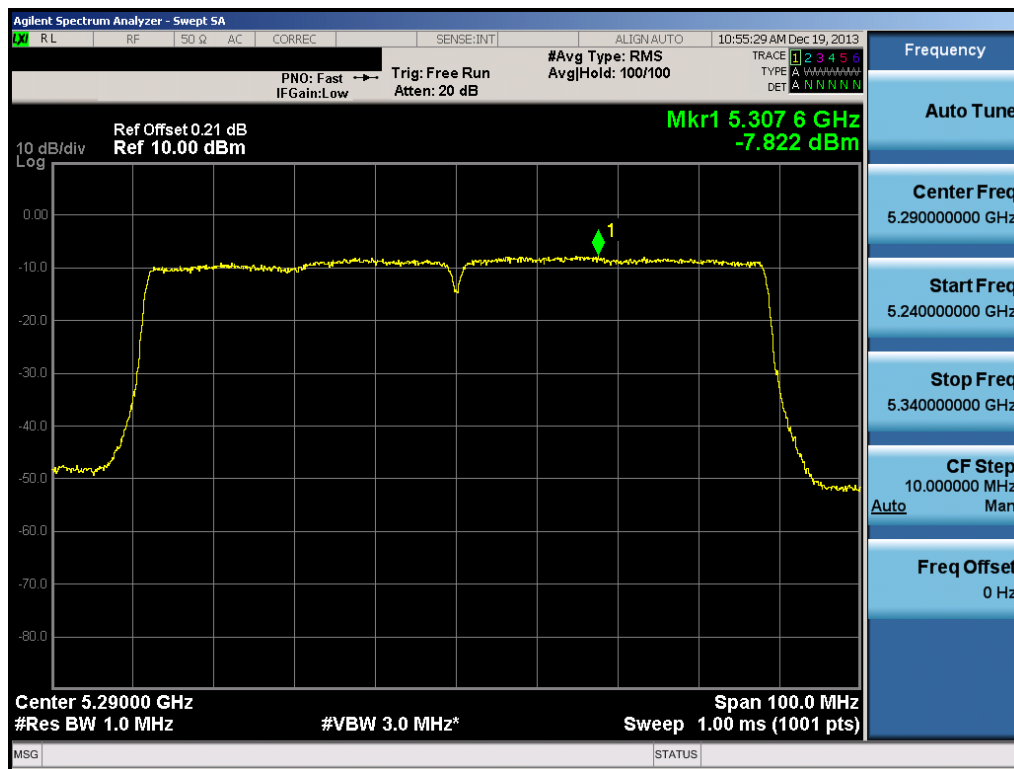
Plot 6-80. Peak Power Spectral Density Plot (80MHz BW 802.11ac (UNII Band 2A) – Ch. 58)
