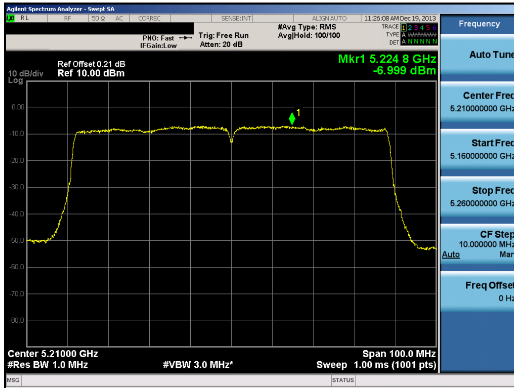
Plot 6-99. Peak Power Spectral Density Plot (80MHz BW 802.11ac (UNII Band 1) – Ch. 42)
