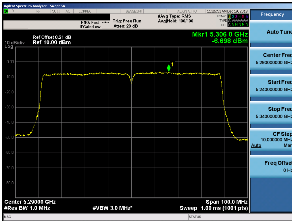
Plot 6-108. Peak Power Spectral Density Plot (80MHz BW 802.11ac (UNII Band 2A) – Ch. 58)
