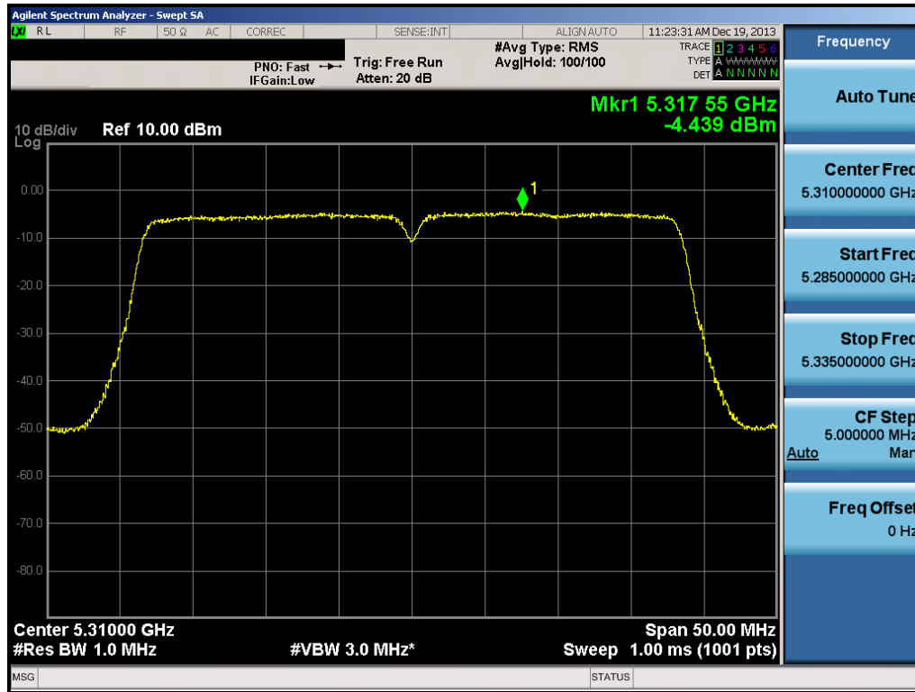
Plot 6-107. Peak Power Spectral Density Plot (40MHz BW 802.11n (UNII Band 2A) – Ch. 62)
