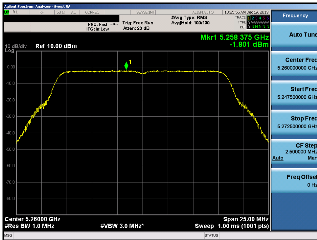
Plot 6-72. Peak Power Spectral Density Plot (802.11a (UNII Band 2A) – Ch. 52)
