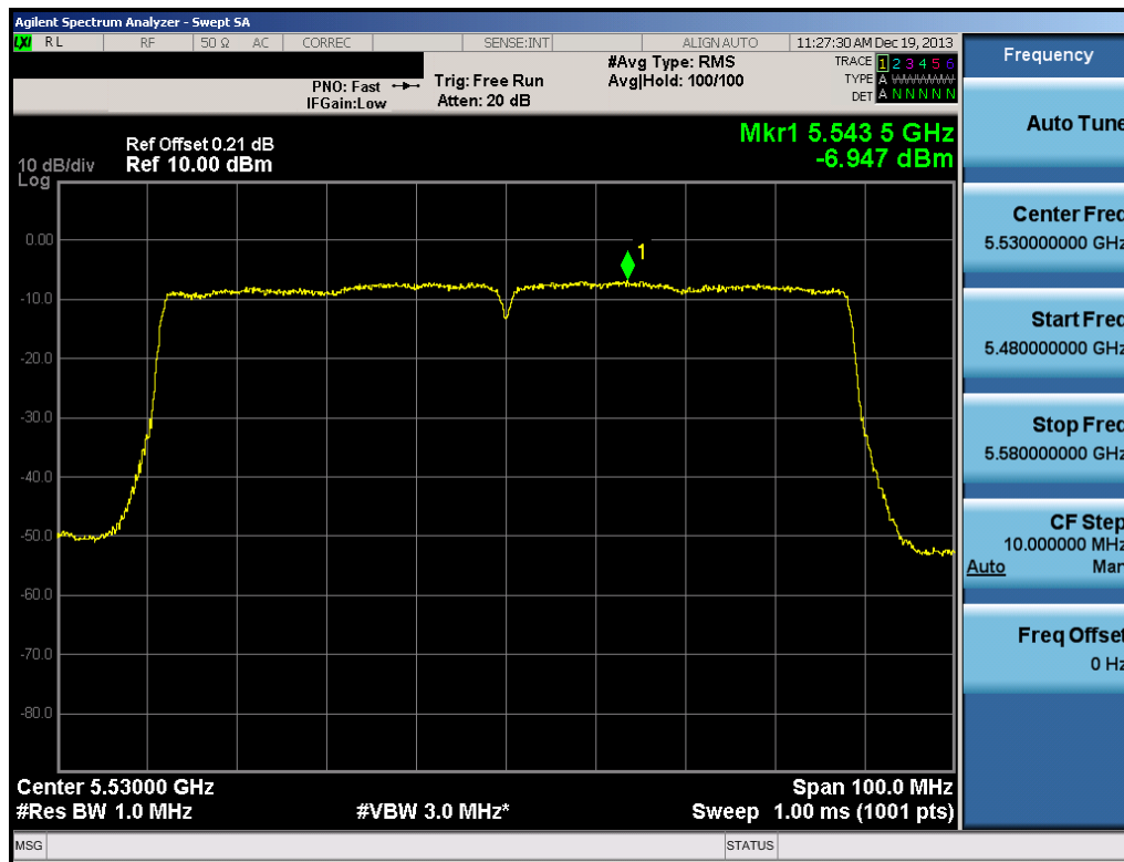
Plot 6-118. Peak Power Spectral Density Plot (80MHz BW 802.11ac (UNII Band 2C) – Ch. 106)
