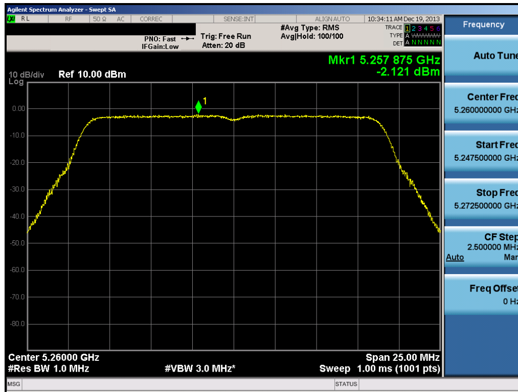
Plot 6-75. Peak Power Spectral Density Plot (20MHz BW 802.11n (UNII Band 2A) – Ch. 52)
