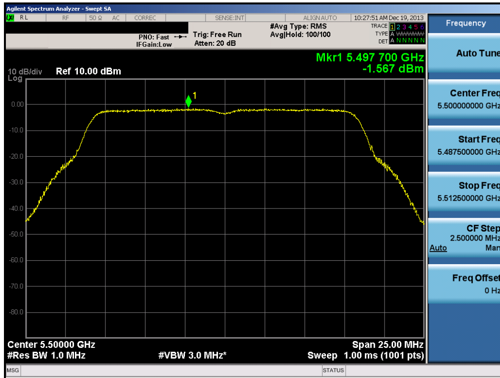
Plot 6-81. Peak Power Spectral Density Plot (802.11a (UNII Band 2C) – Ch. 100)
