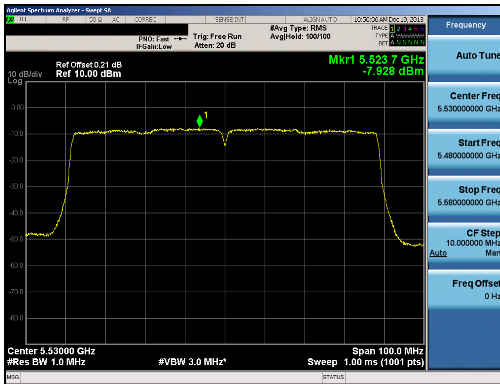
Plot 6-90. Peak Power Spectral Density Plot (80MHz BW 802.11ac (UNII Band 2C) – Ch. 106)
