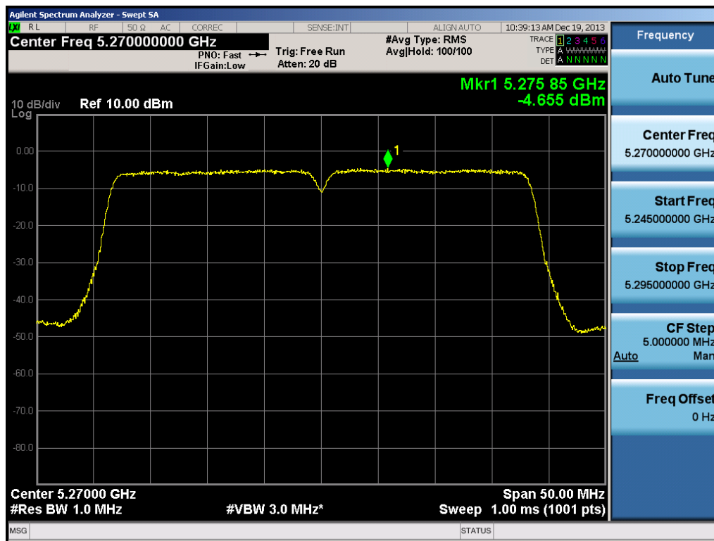
Plot 6-78. Peak Power Spectral Density Plot (40MHz BW 802.11n (UNII Band 2A) – Ch. 54)
