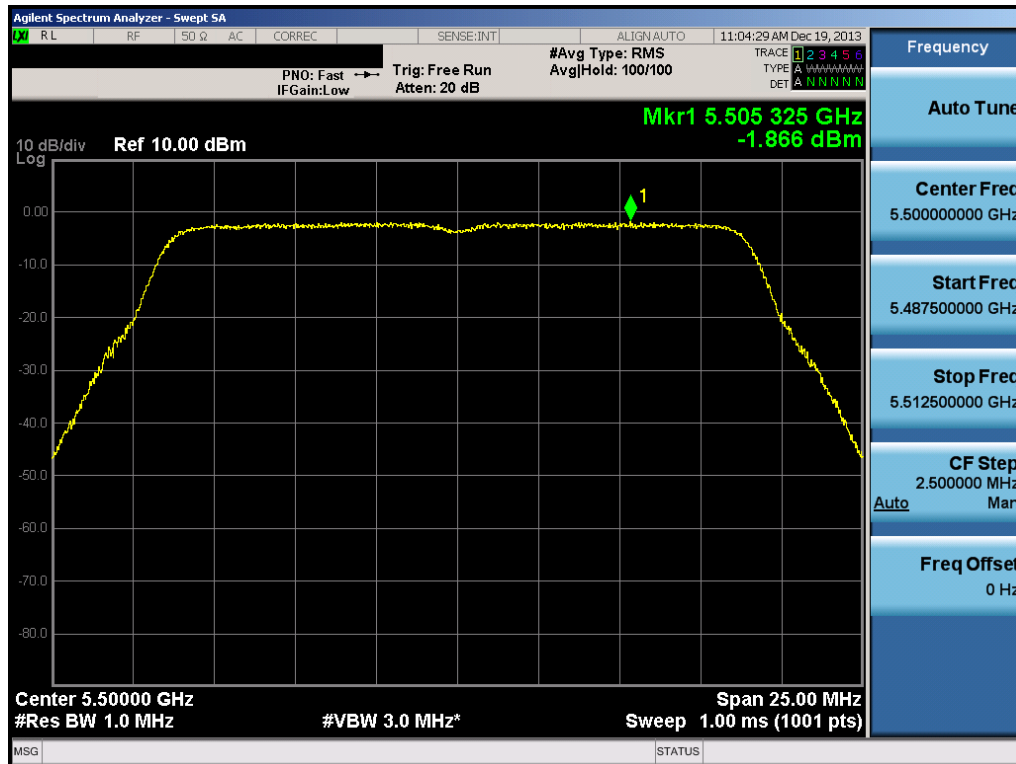
Plot 6-112. Peak Power Spectral Density Plot (20MHz BW 802.11n (UNII Band 2C) – Ch. 100)
