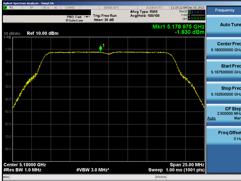
Plot 6-91. Peak Power Spectral Density Plot (802.11a (UNII Band 1) – Ch. 36)
