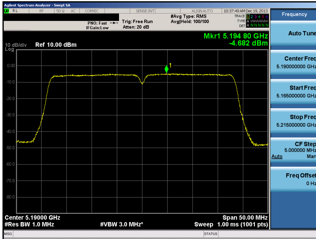
Plot 6-69. Peak Power Spectral Density Plot (40MHz BW 802.11n (UNII Band 1) – Ch. 38)
