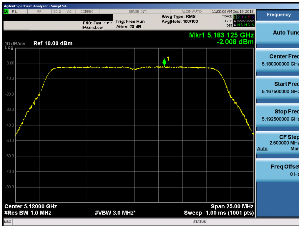
Plot 6-94. Peak Power Spectral Density Plot (20MHz BW 802.11n (UNII Band 1) – Ch. 36)
