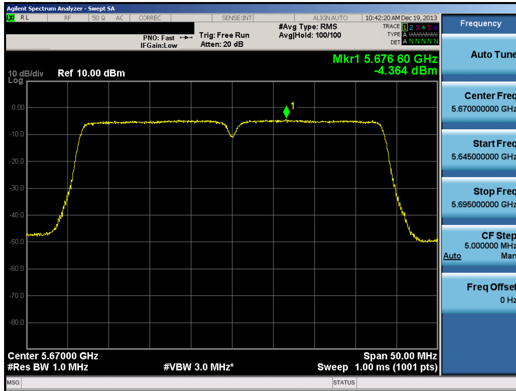
Plot 6-89. Peak Power Spectral Density Plot (40MHz BW 802.11n (UNII Band 2C) – Ch. 134)
