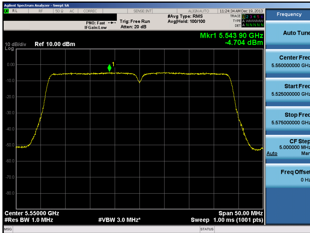
Plot 6-116. Peak Power Spectral Density Plot (40MHz BW 802.11n (UNII Band 2C) – Ch. 110)
