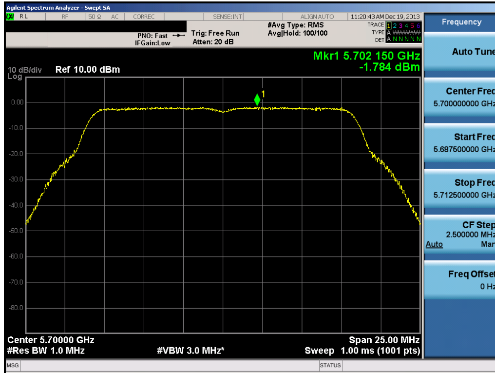
Plot 6-111. Peak Power Spectral Density Plot (802.11a (UNII Band 2C) – Ch. 140)
