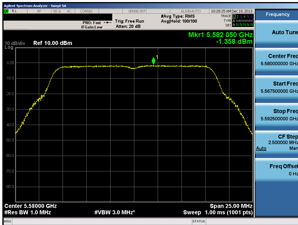
Plot 6-82. Peak Power Spectral Density Plot (802.11a (UNII Band 2C) – Ch. 116)
