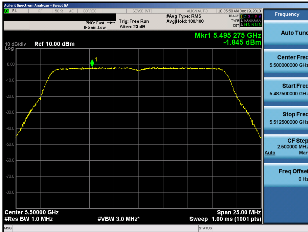
Plot 6-84. Peak Power Spectral Density Plot (20MHz BW 802.11n (UNII Band 2C) – Ch. 100)
