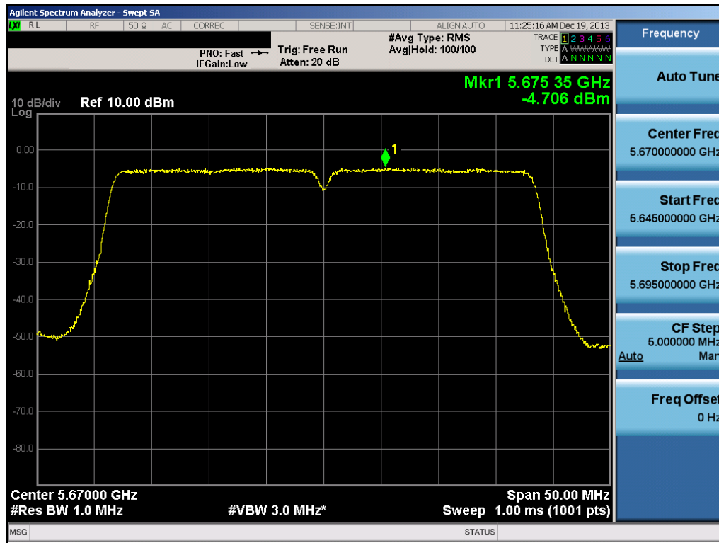
Plot 6-117. Peak Power Spectral Density Plot (40MHz BW 802.11n (UNII Band 2C) – Ch. 134)
