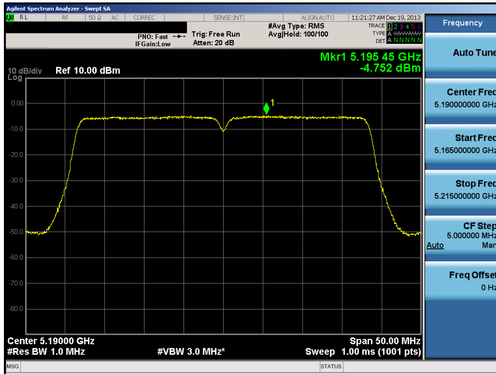
Plot 6-97. Peak Power Spectral Density Plot (40MHz BW 802.11n (UNII Band 1) – Ch. 38)
