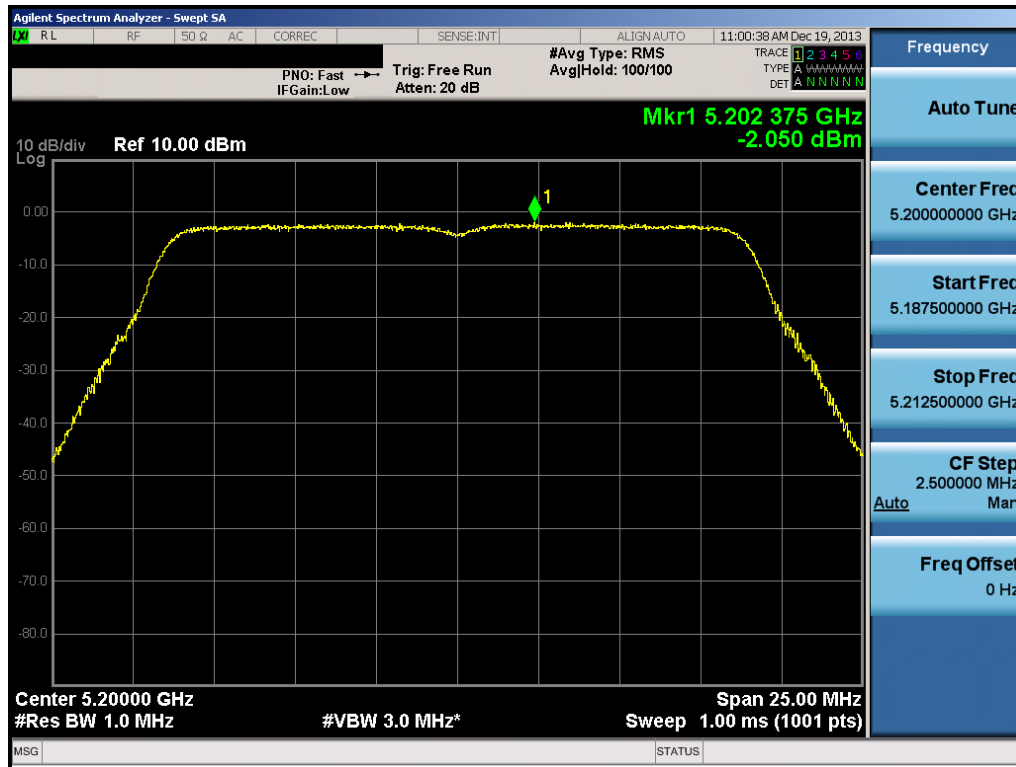
Plot 6-95. Peak Power Spectral Density Plot (20MHz BW 802.11n (UNII Band 1) – Ch. 40)
