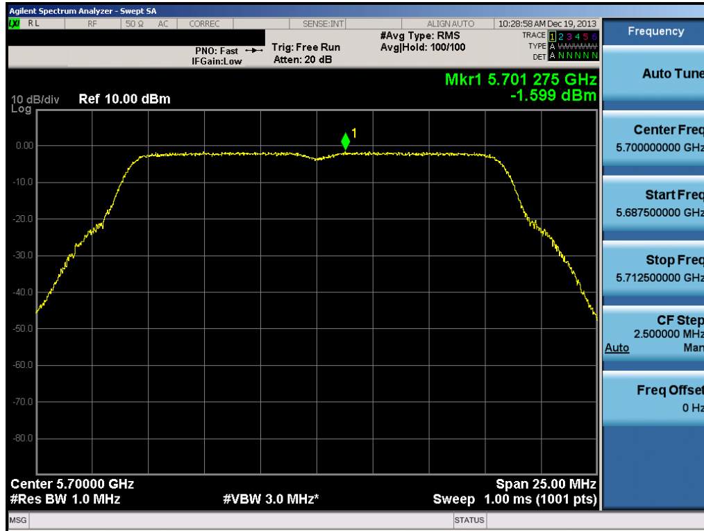
Plot 6-83. Peak Power Spectral Density Plot (802.11a (UNII Band 2C) – Ch. 140)
