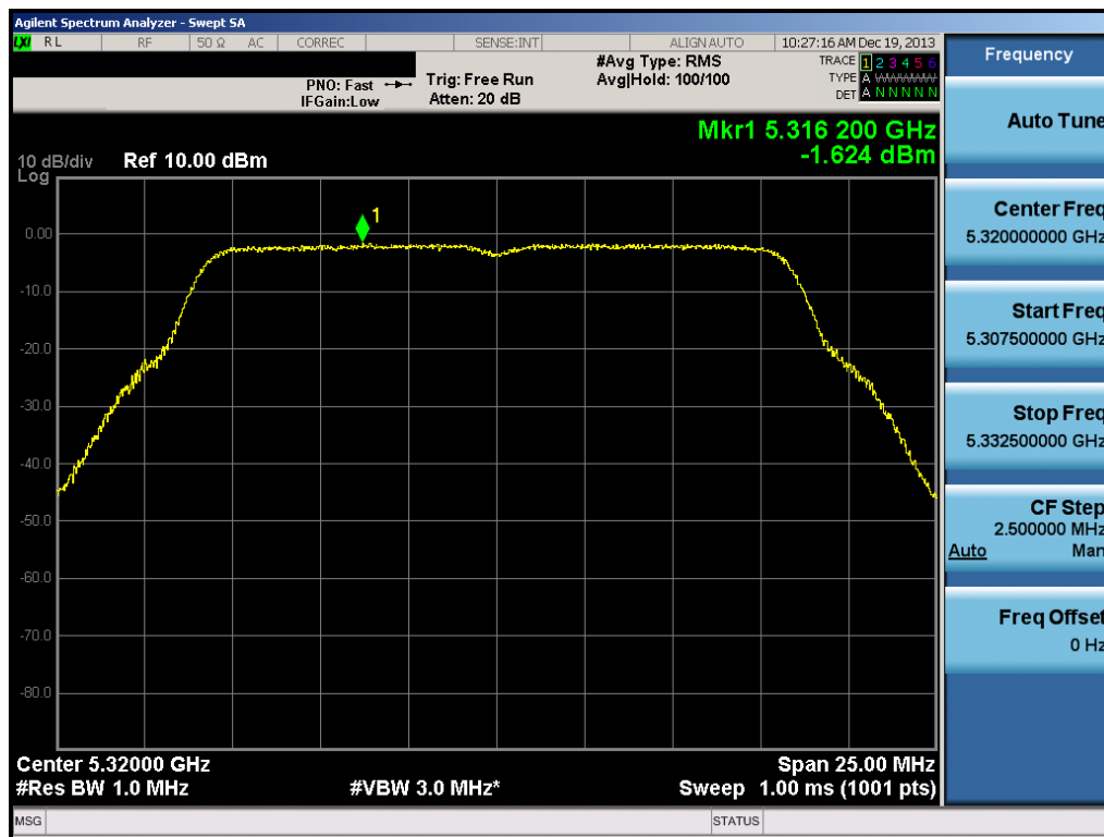
Plot 6-74. Peak Power Spectral Density Plot (802.11a (UNII Band 2A) – Ch. 64)
