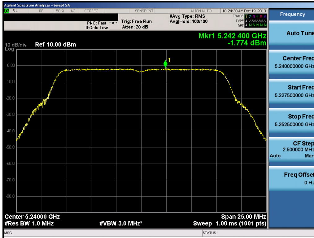
Plot 6-65. Peak Power Spectral Density Plot (802.11a (UNII Band 1) – Ch. 48)
