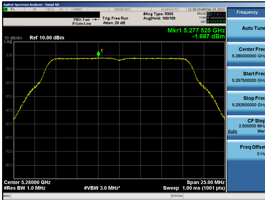
Plot 6-101. Peak Power Spectral Density Plot (802.11a (UNII Band 2A) – Ch. 56)
