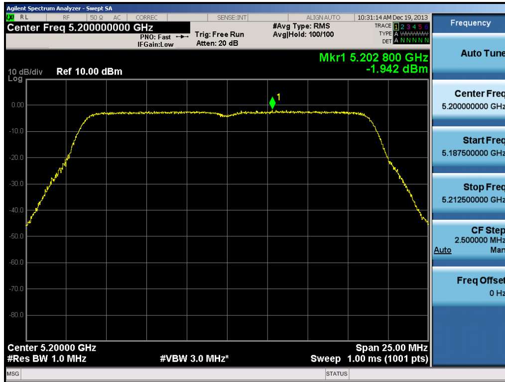
Plot 6-67. Peak Power Spectral Density Plot (20MHz BW 802.11n (UNII Band 1) – Ch. 40)
