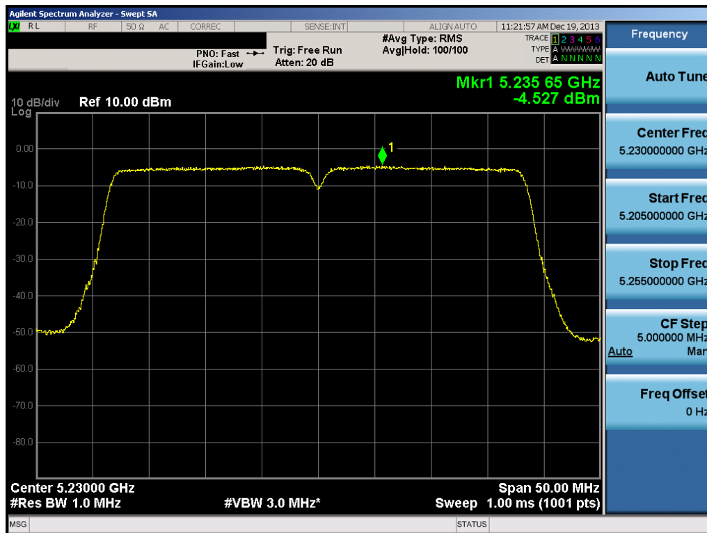
Plot 6-98. Peak Power Spectral Density Plot (40MHz BW 802.11n (UNII Band 1) – Ch. 46)
