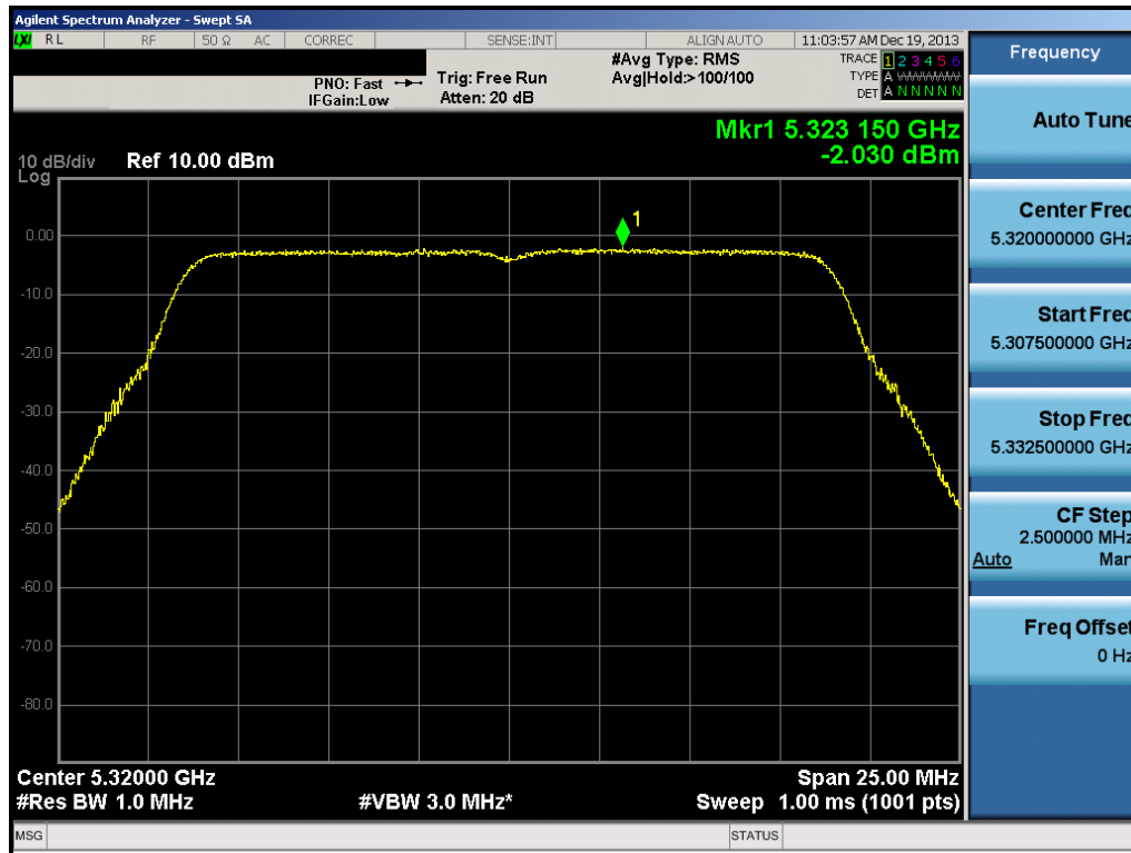
Plot 6-105. Peak Power Spectral Density Plot (20MHz BW 802.11n (UNII Band 2A) – Ch. 64)
