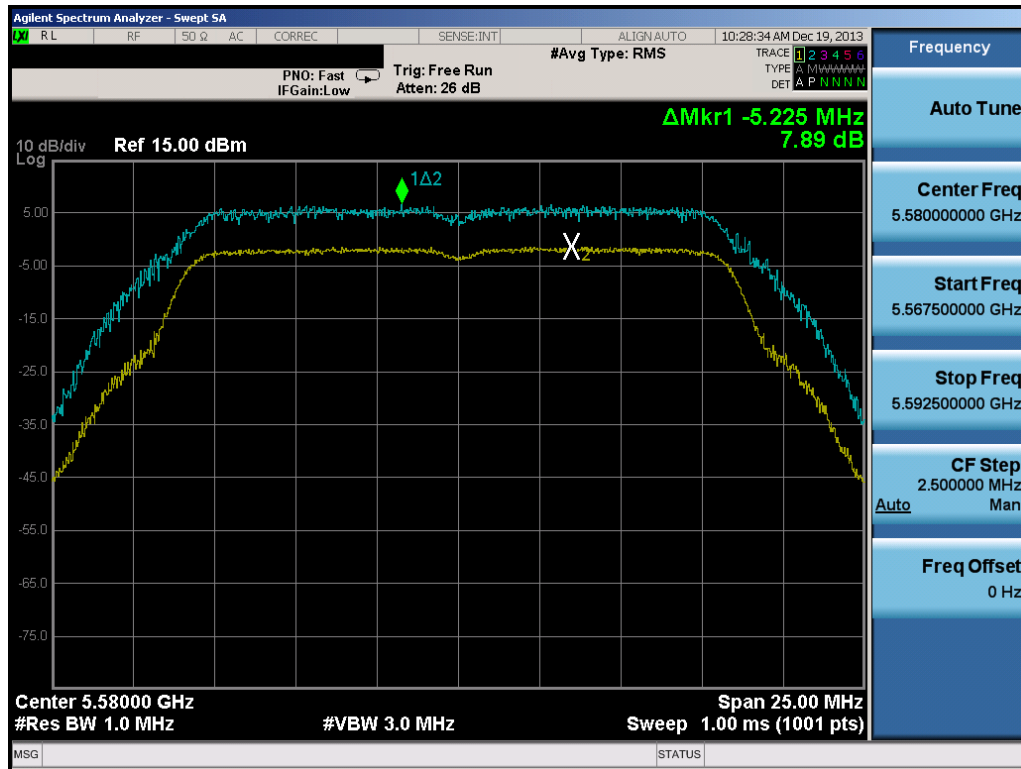
Plot 6-119. Peak Excursion Ratio Plot (802.11a)
