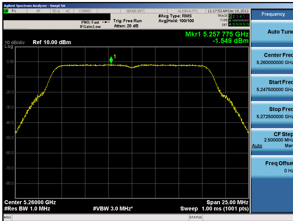
Plot 6-100. Peak Power Spectral Density Plot (802.11a (UNII Band 2A) – Ch. 52)
