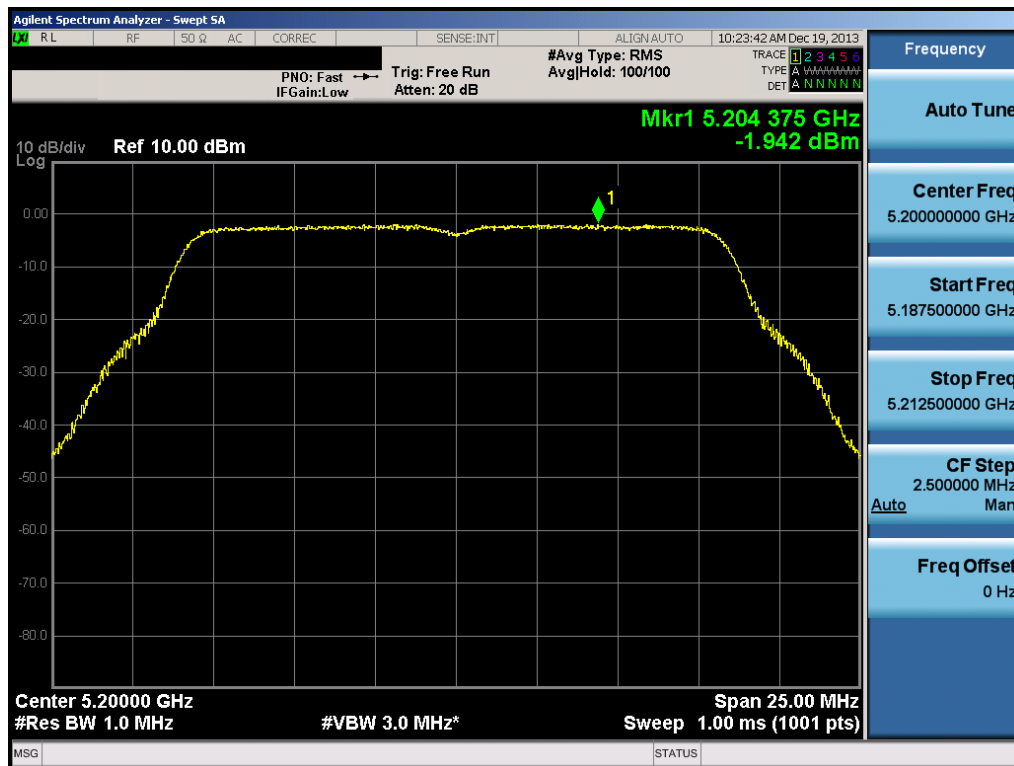
Plot 6-64. Peak Power Spectral Density Plot (802.11a (UNII Band 1) – Ch. 40)
