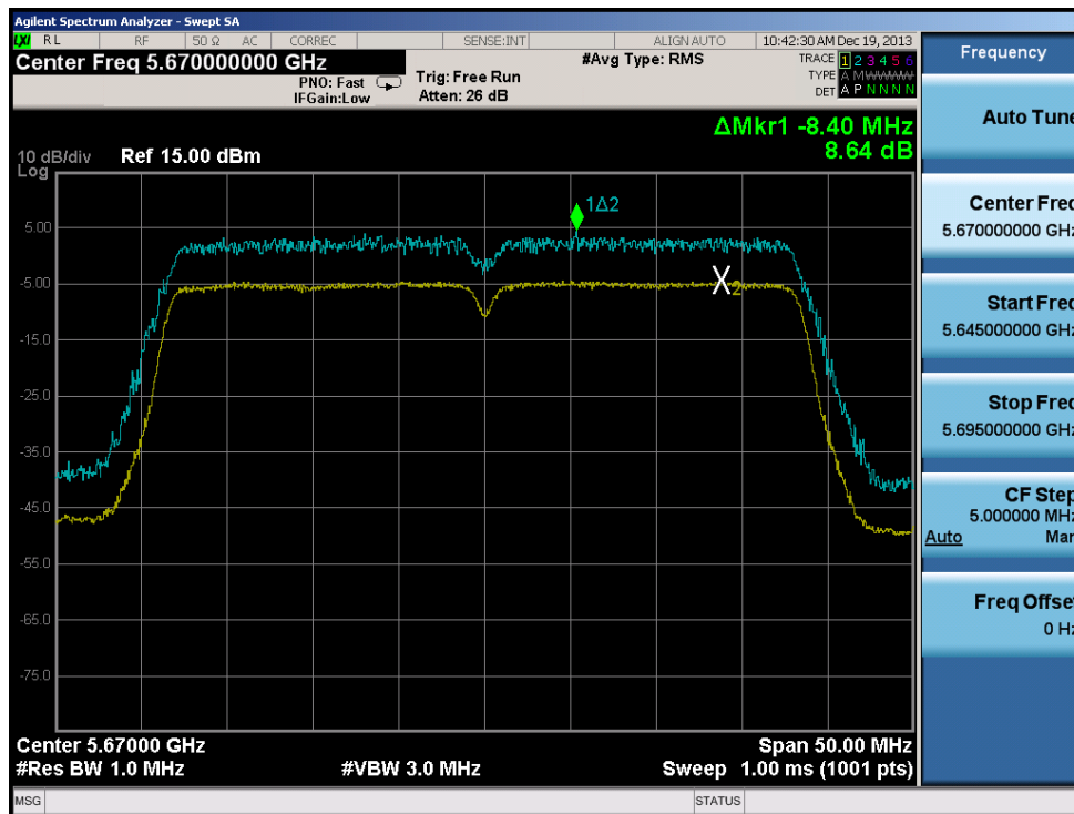
Plot 6-121. Peak Excursion Ratio Plot (40MHz BW 802.11n)
