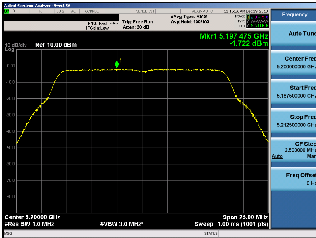
Plot 6-92. Peak Power Spectral Density Plot (802.11a (UNII Band 1) – Ch. 40)
