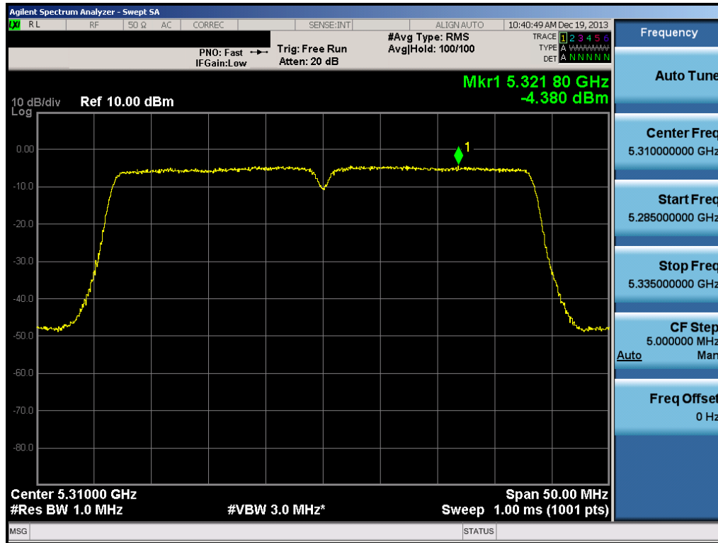
Plot 6-79. Peak Power Spectral Density Plot (40MHz BW 802.11n (UNII Band 2A) – Ch. 62)
