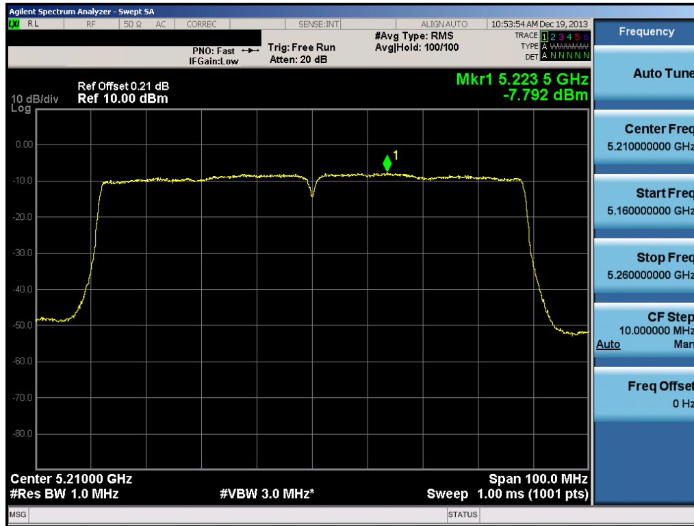
Plot 6-71. Peak Power Spectral Density Plot (80MHz BW 802.11ac (UNII Band 1) – Ch. 42)
