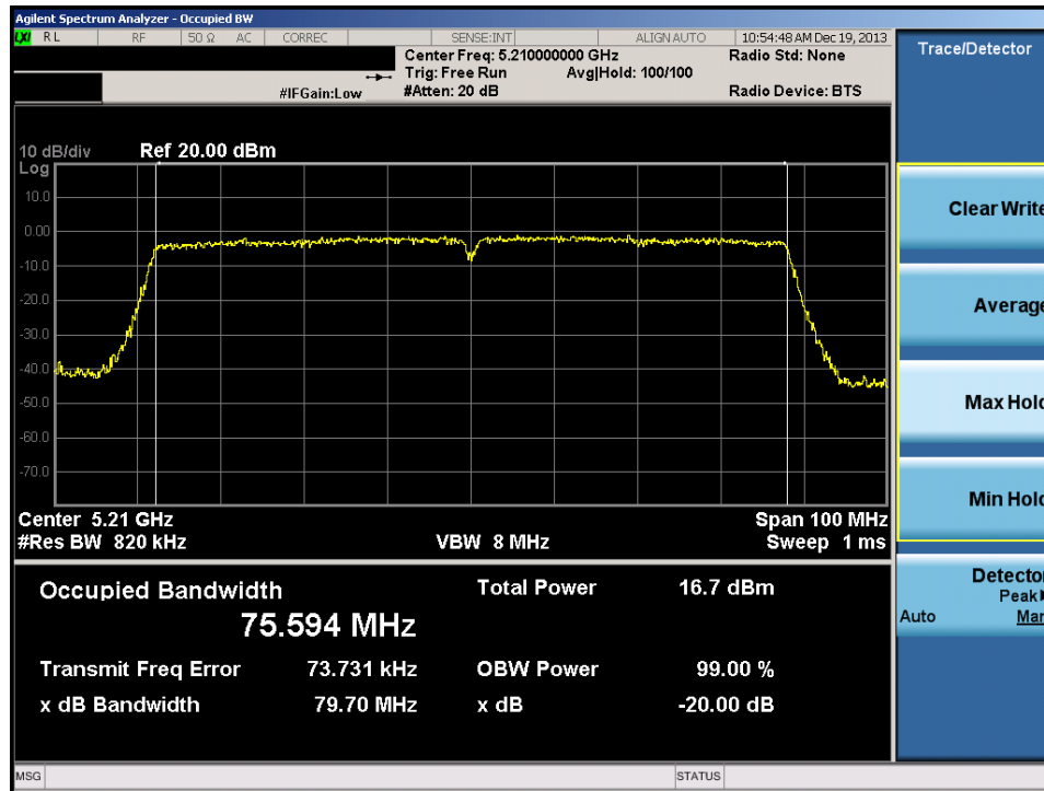
Plot 6-62. 20dB Bandwidth Plot (80MHz BW 802.11ac (UNII Band 1) – Ch. 42)
