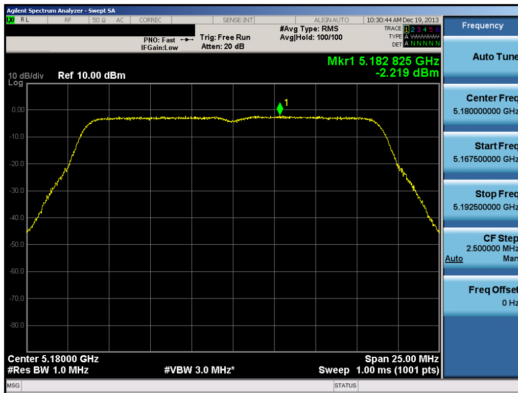
Plot 6-66. Peak Power Spectral Density Plot (20MHz BW 802.11n (UNII Band 1) – Ch. 36)
