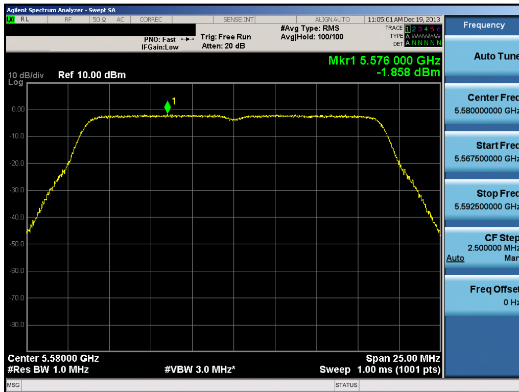
Plot 6-113. Peak Power Spectral Density Plot (20MHz BW 802.11n (UNII Band 2C) – Ch. 116)
