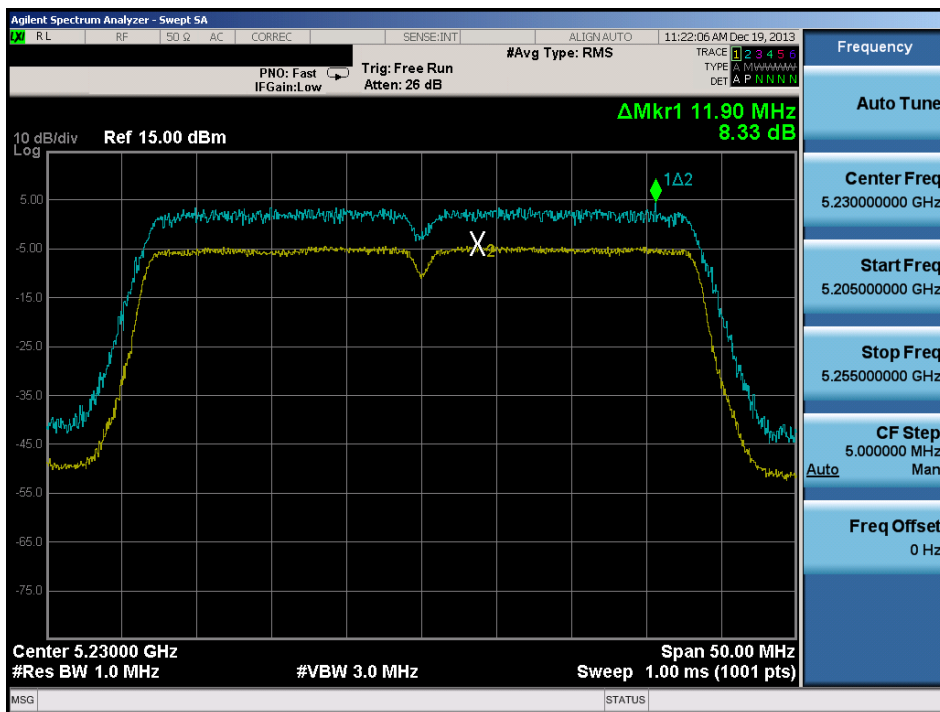
Plot 6-125. Peak Excursion Ratio Plot (40MHz BW 802.11n)
