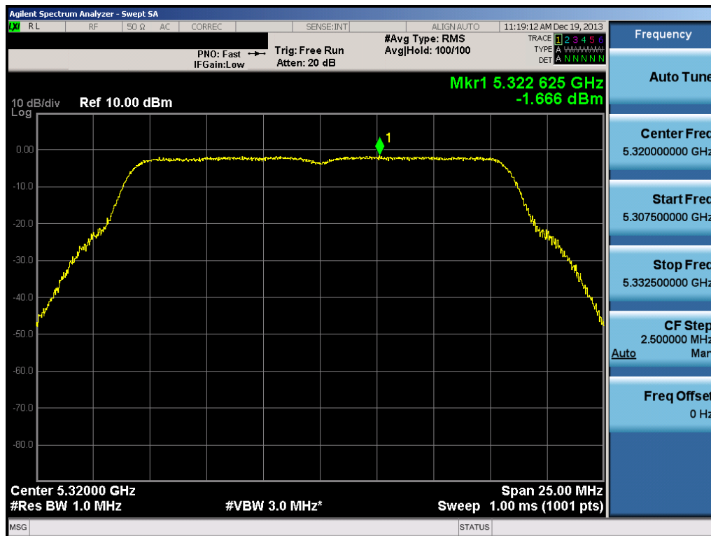
Plot 6-102. Peak Power Spectral Density Plot (802.11a (UNII Band 2A) – Ch. 64)
