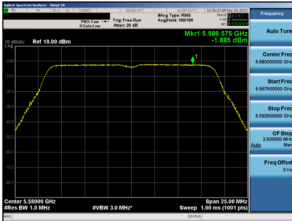
Plot 6-85. Peak Power Spectral Density Plot (20MHz BW 802.11n (UNII Band 2C) – Ch. 116)
