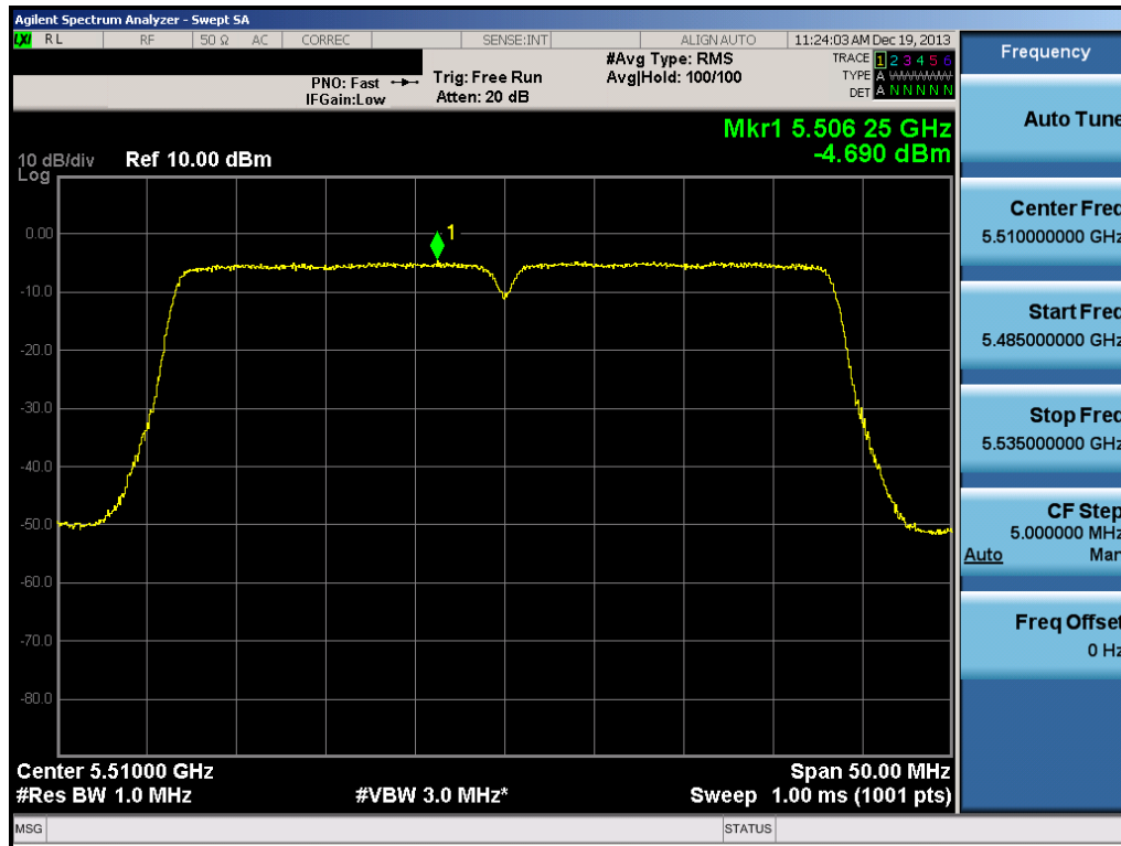
Plot 6-115. Peak Power Spectral Density Plot (40MHz BW 802.11n (UNII Band 2C) – Ch. 102)
