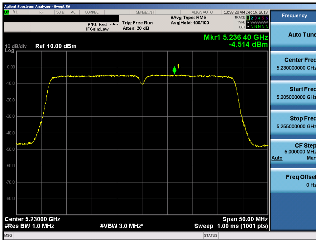
Plot 6-70. Peak Power Spectral Density Plot (40MHz BW 802.11n (UNII Band 1) – Ch. 46)
