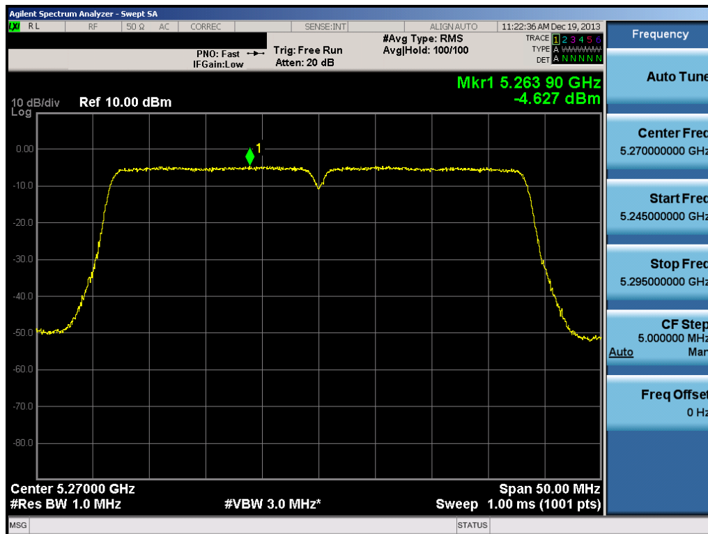
Plot 6-106. Peak Power Spectral Density Plot (40MHz BW 802.11n (UNII Band 2A) – Ch. 54)
