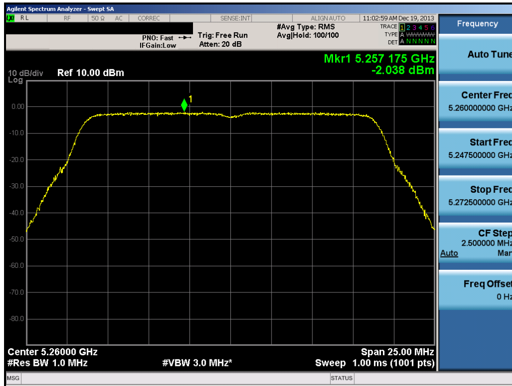
Plot 6-103. Peak Power Spectral Density Plot (20MHz BW 802.11n (UNII Band 2A) – Ch. 52)
