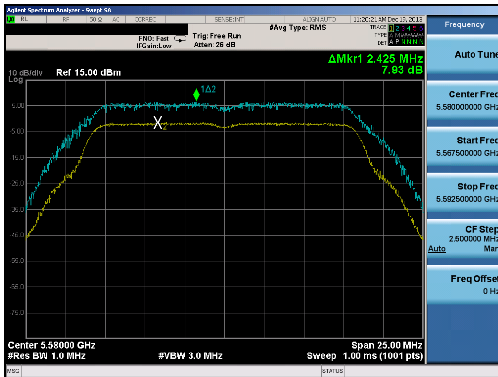
Plot 6-123. Peak Excursion Ratio Plot (802.11a)
