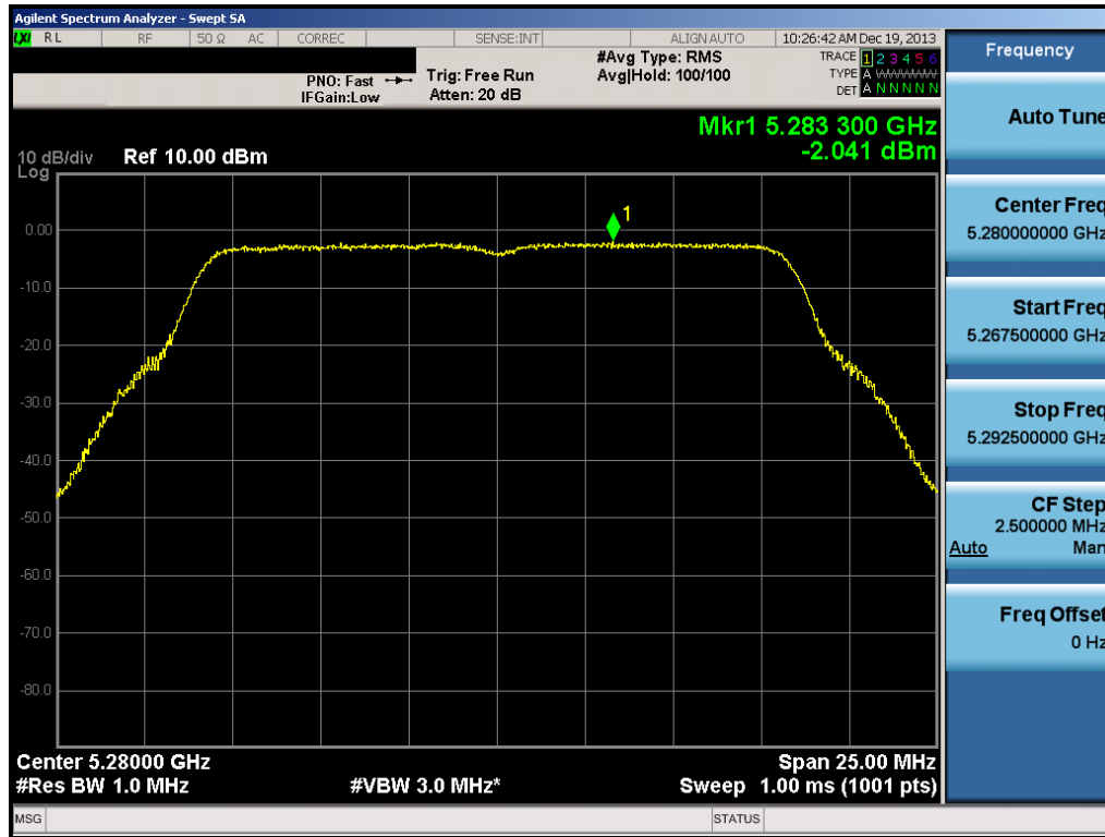
Plot 6-73. Peak Power Spectral Density Plot (802.11a (UNII Band 2A) – Ch. 56)
