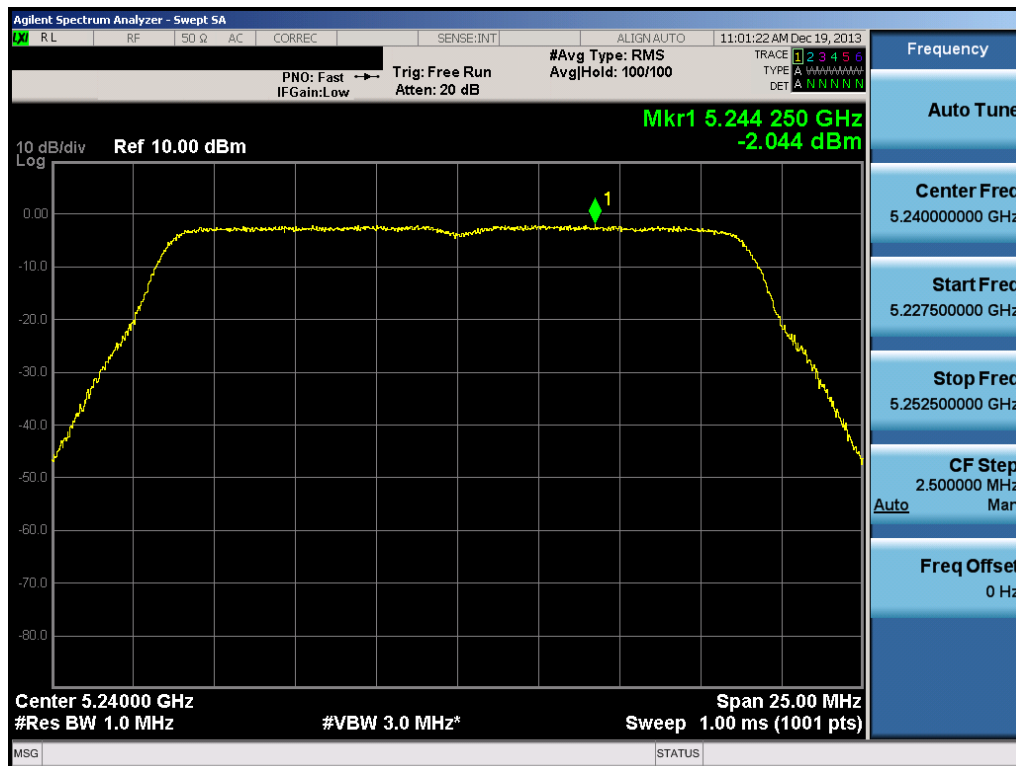
Plot 6-96. Peak Power Spectral Density Plot (20MHz BW 802.11n (UNII Band 1) – Ch. 48)
