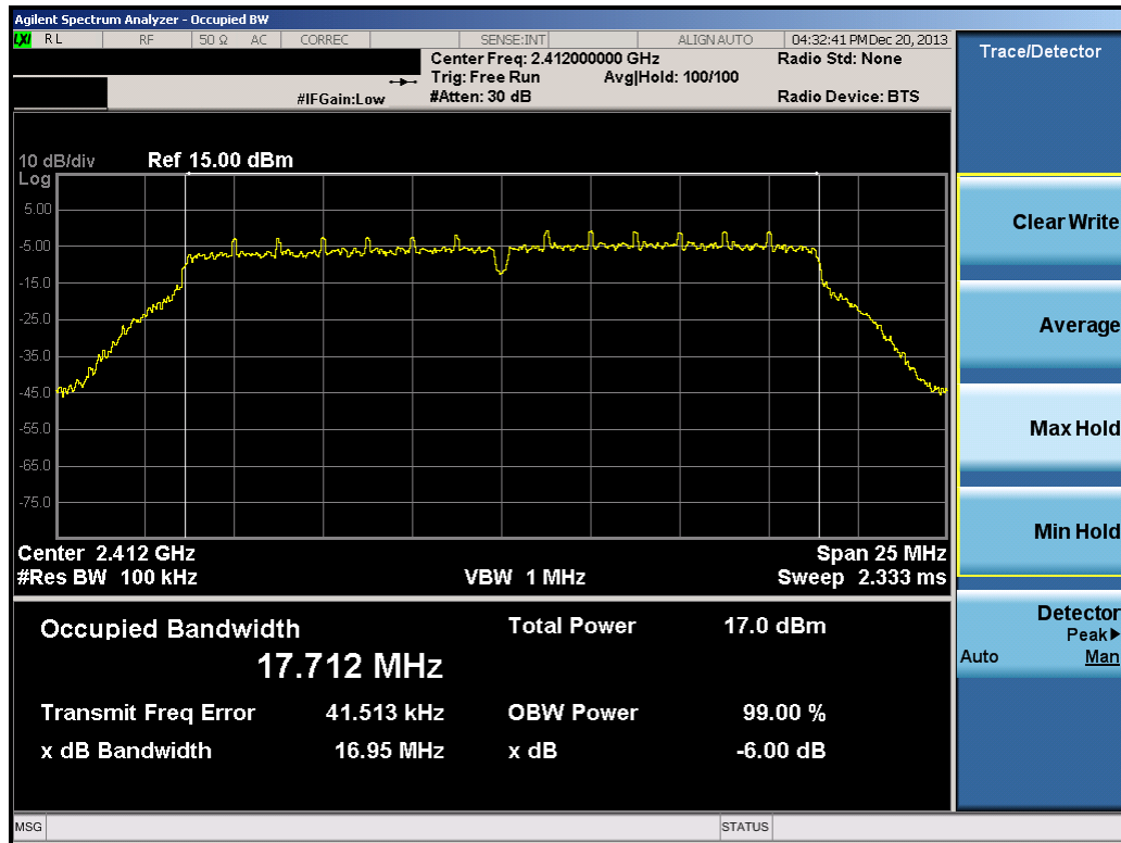
Plot 6-25. 6dB Bandwidth Plot (802.11n (2.4GHz) – Ch. 1)
