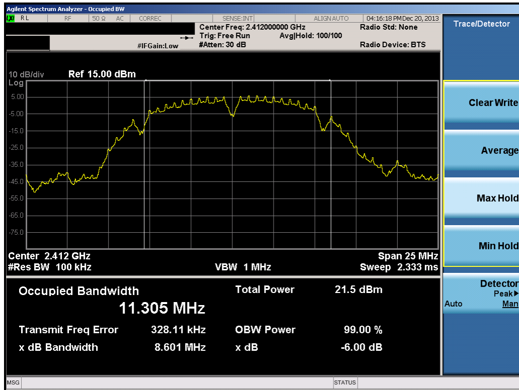
Plot 6-19. 6dB Bandwidth Plot (802.11b – Ch. 1)
