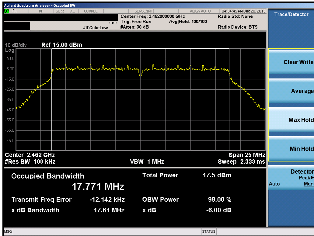
Plot 6-27. 6dB Bandwidth Plot (802.11n (2.4GHz) – Ch. 11)
