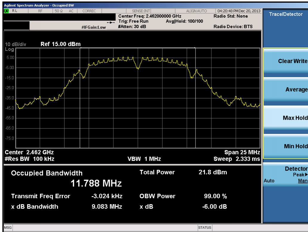
Plot 6-21. 6dB Bandwidth Plot (802.11b – Ch. 11)
