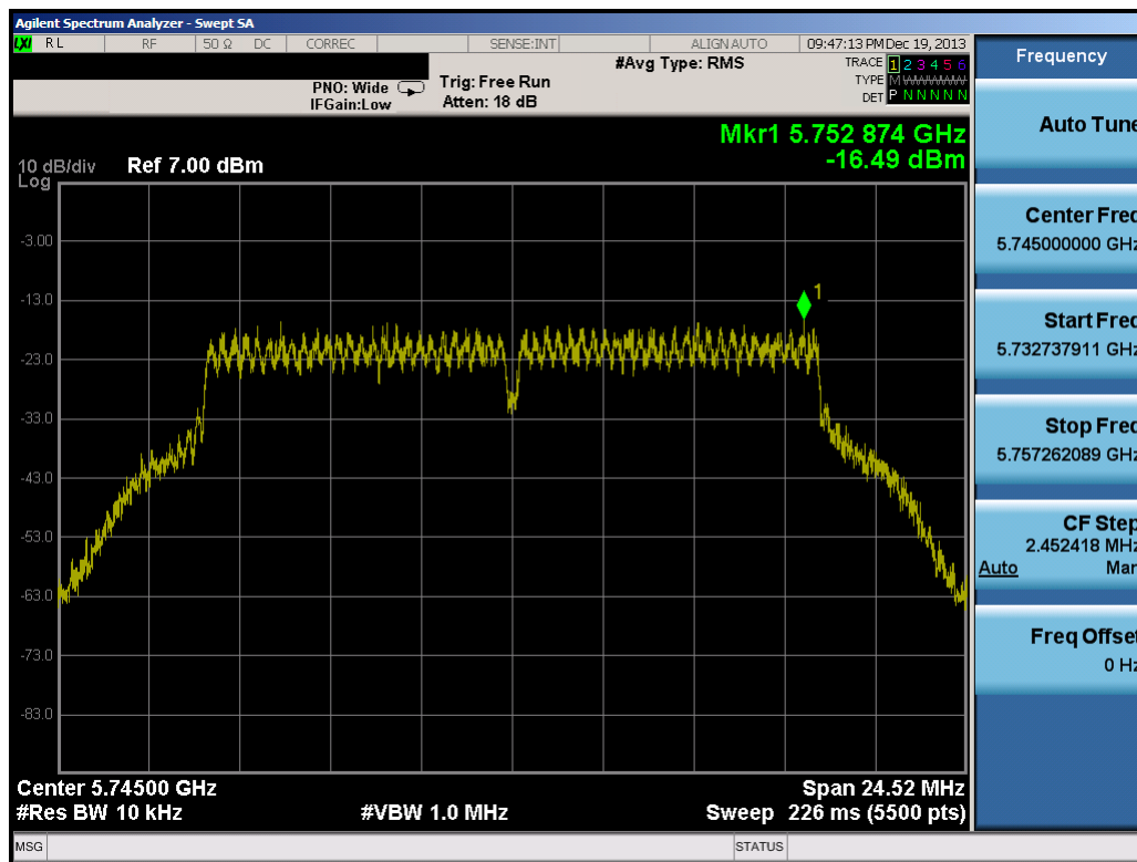
Plot 6-46. Power Spectral Density Plot (802.11a – Ch. 149)
