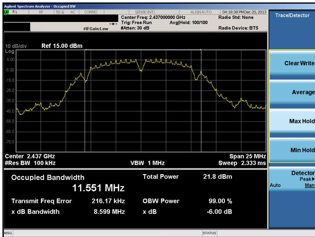
Plot 6-20. 6dB Bandwidth Plot (802.11b – Ch. 6)
