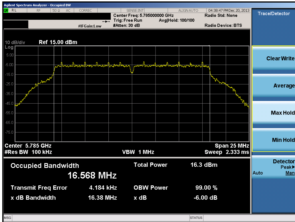
Plot 6-29. 6dB Bandwidth Plot (802.11a – Ch. 157)
