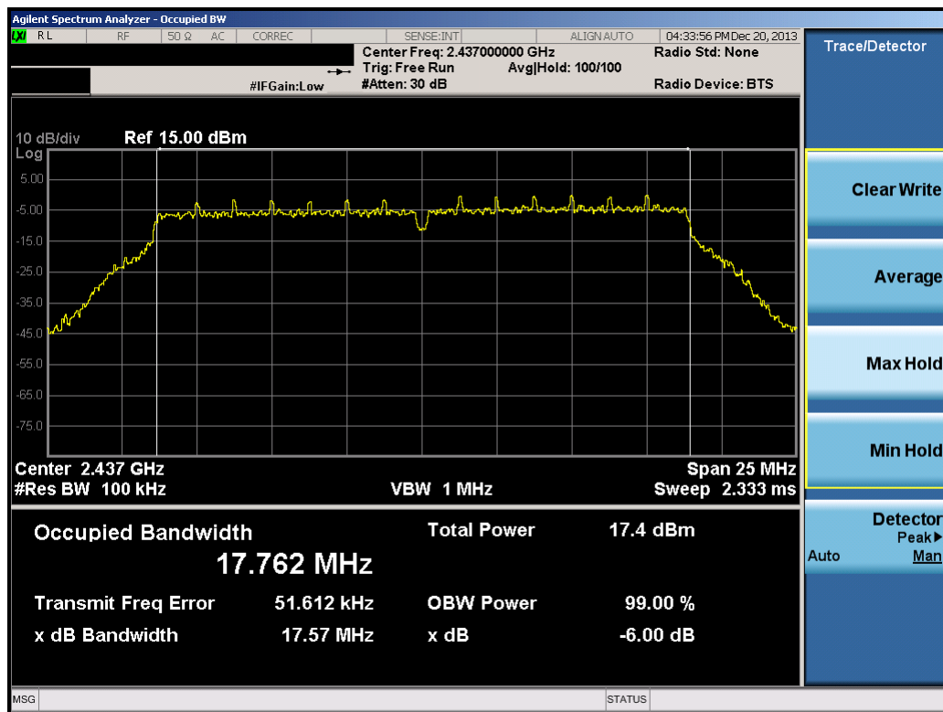
Plot 6-26. 6dB Bandwidth Plot (802.11n (2.4GHz) – Ch. 6)
