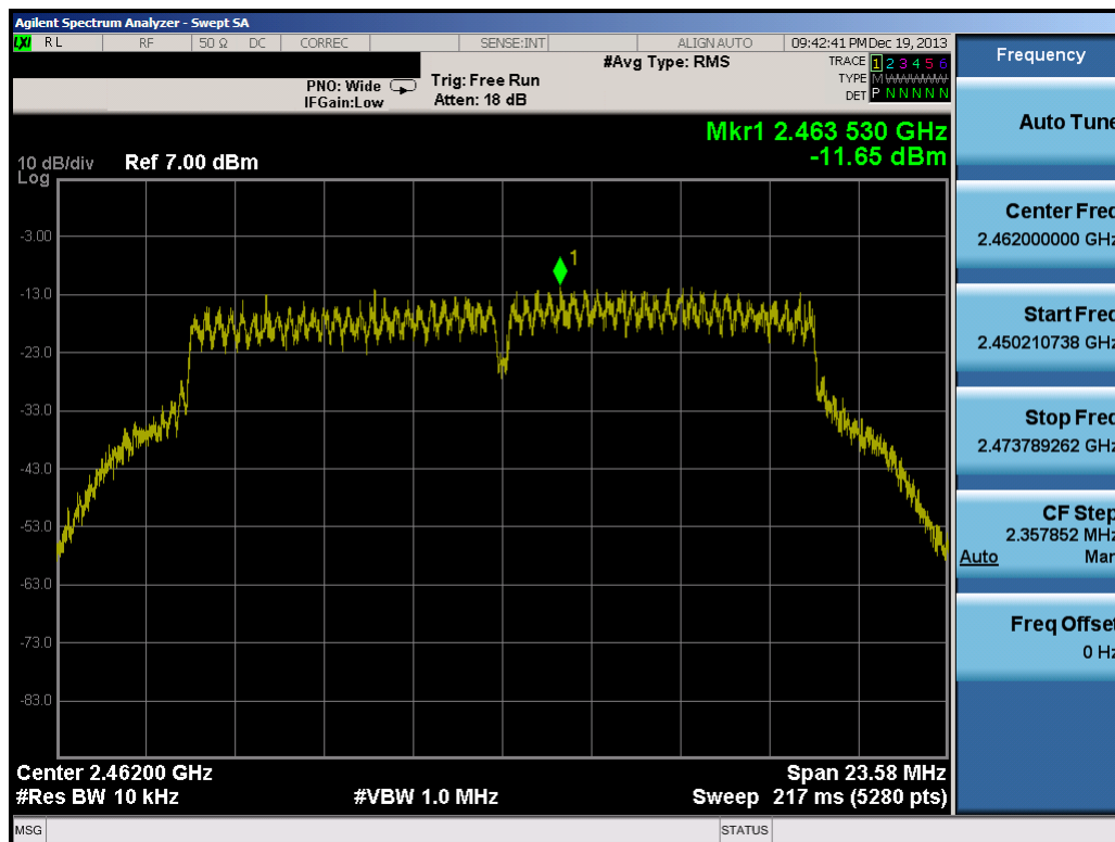
Plot 6-42. Power Spectral Density Plot (802.11g – Ch. 11)
