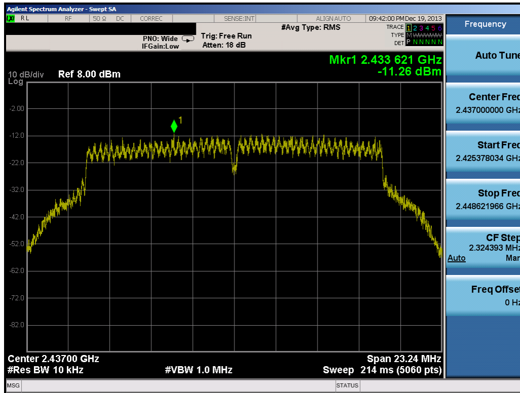
Plot 6-41. Power Spectral Density Plot (802.11g – Ch. 6)
