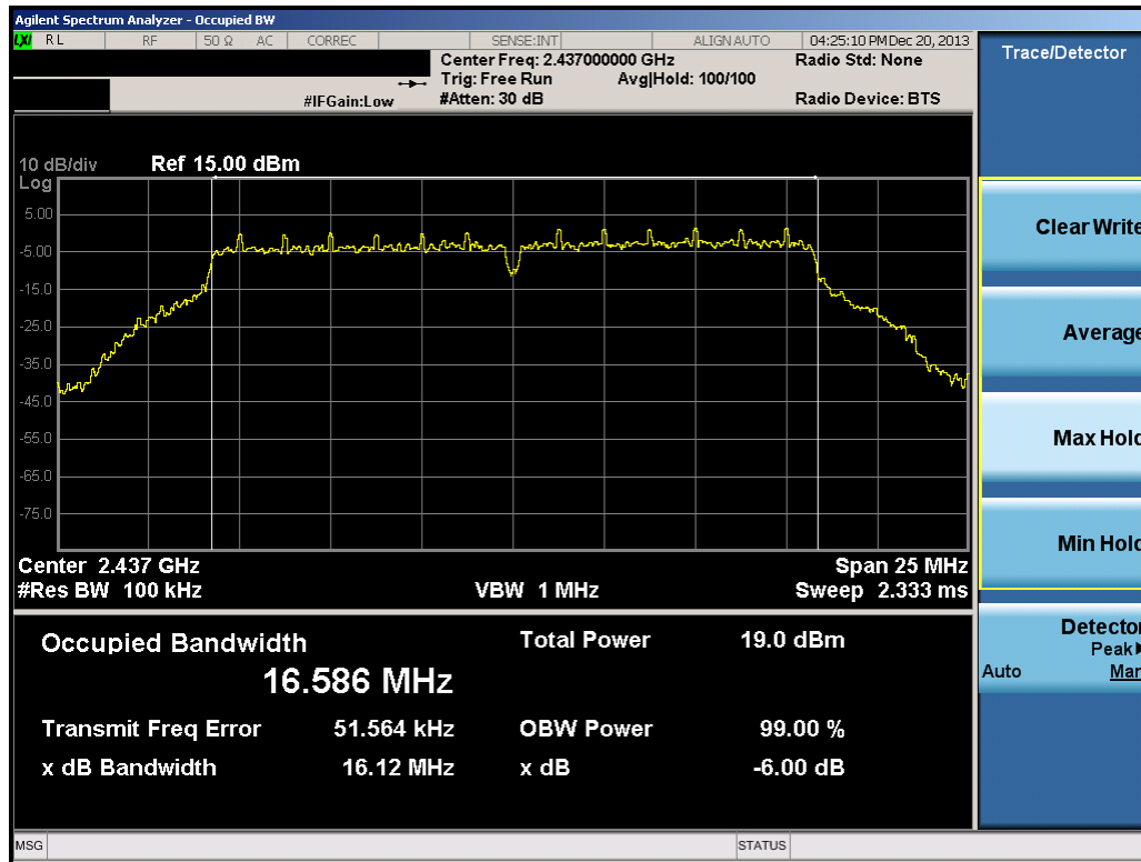
Plot 6-23. 6dB Bandwidth Plot (802.11g – Ch. 6)
