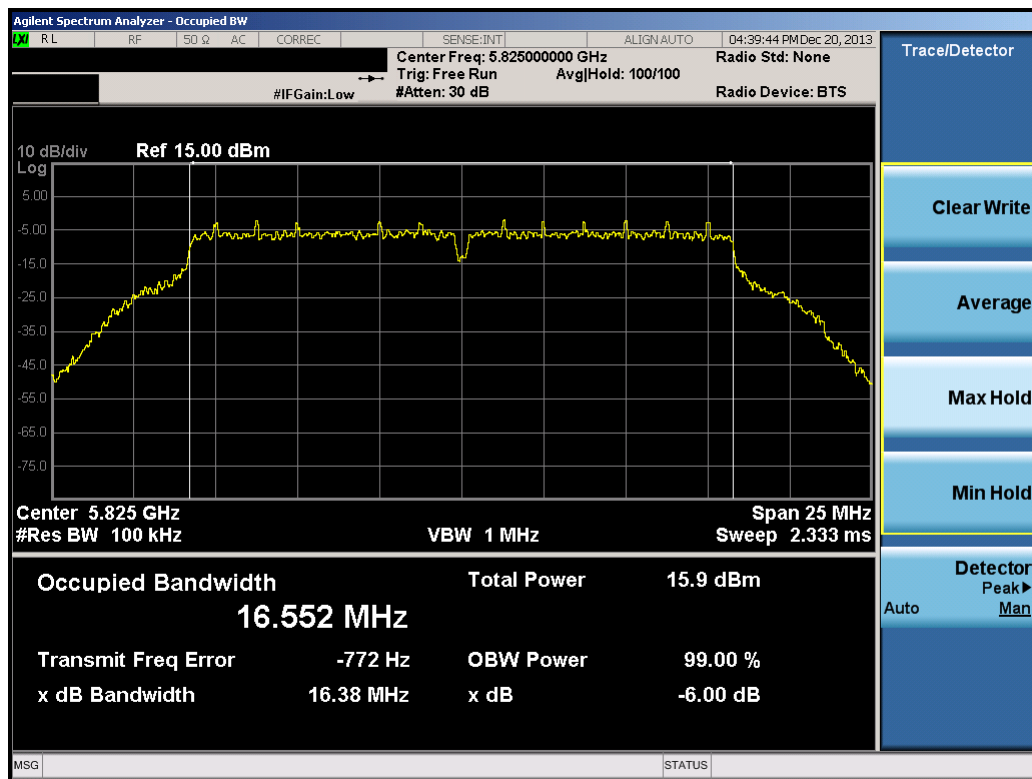
Plot 6-30. 6dB Bandwidth Plot (802.11a – Ch. 165)
