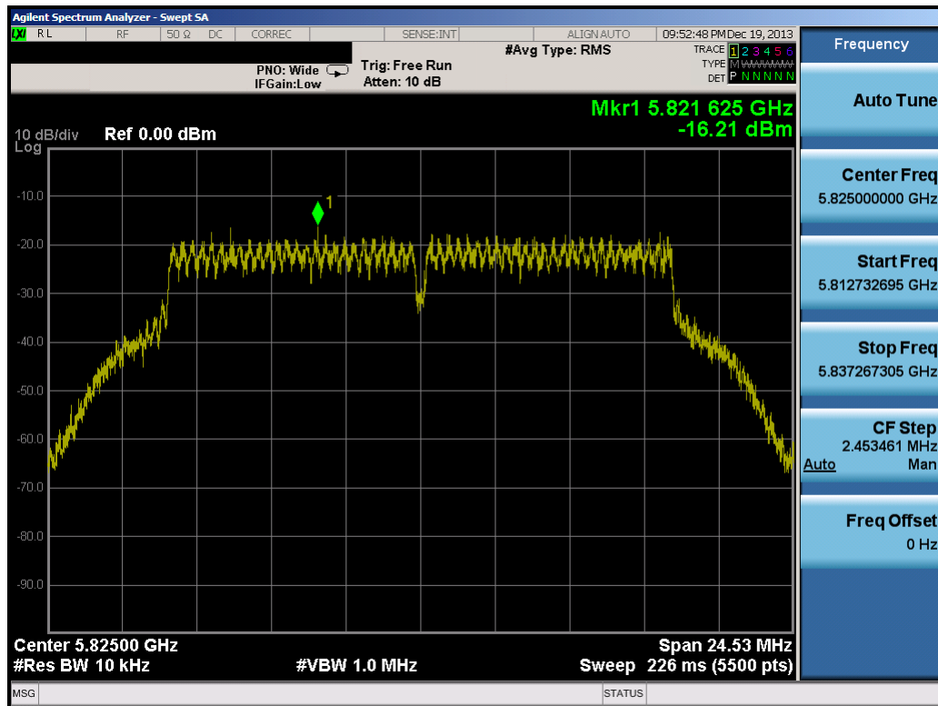
Plot 6-48. Power Spectral Density Plot (802.11a – Ch. 165)
