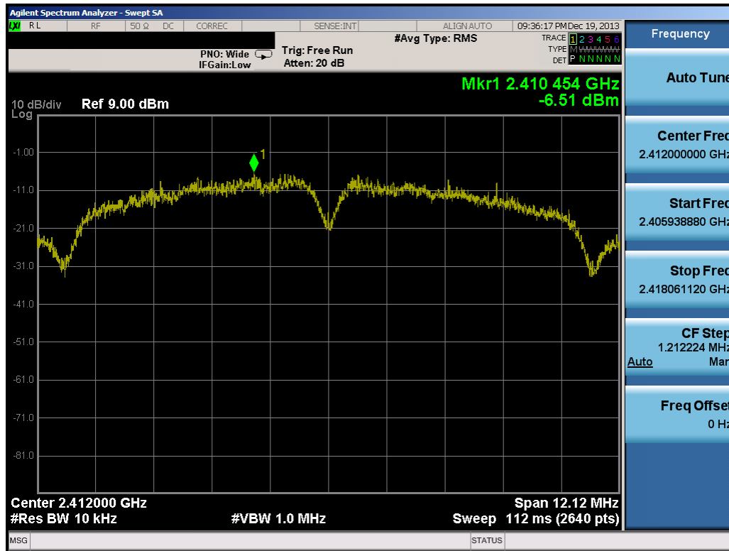
Plot 6-37. Power Spectral Density Plot (802.11b – Ch. 1)
