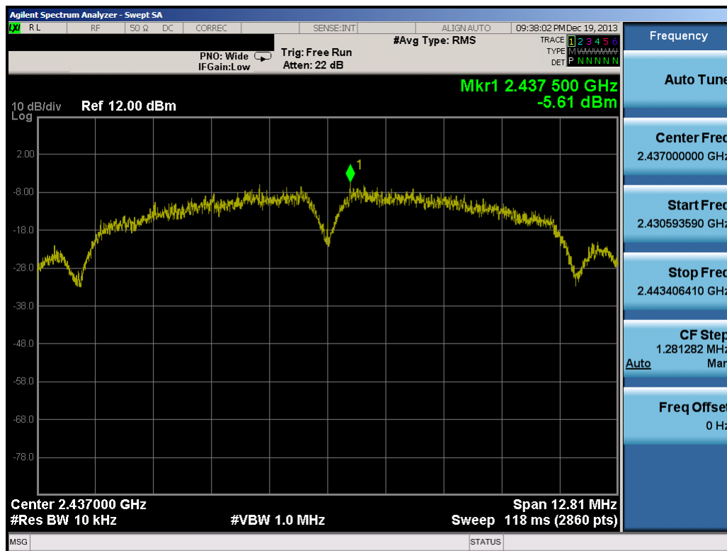
Plot 6-38. Power Spectral Density Plot (802.11b – Ch. 6)
