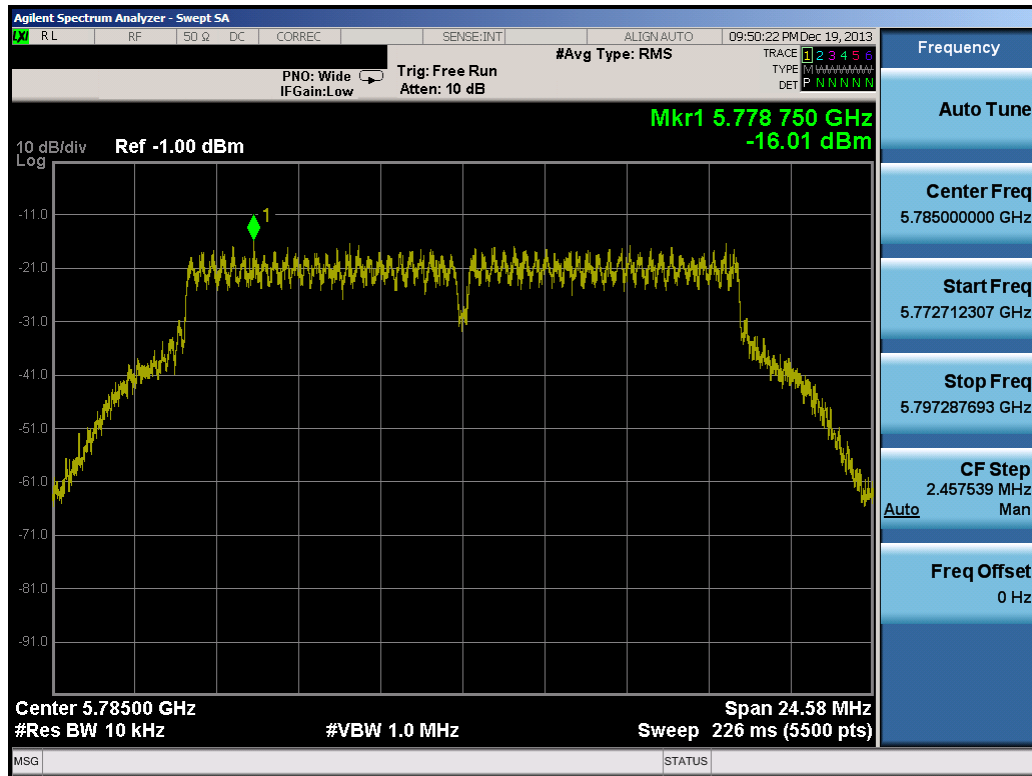
Plot 6-47. Power Spectral Density Plot (802.11a – Ch. 157)
