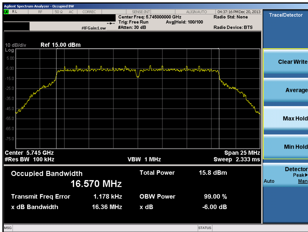
Plot 6-28. 6dB Bandwidth Plot (802.11a – Ch. 149)
