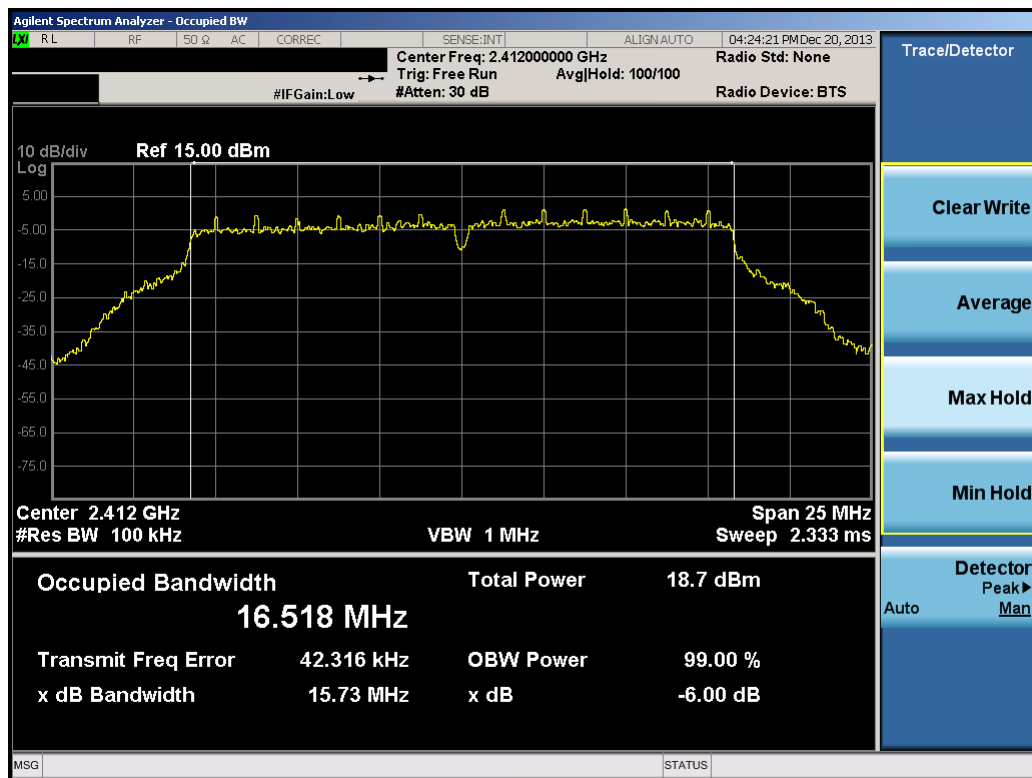
Plot 6-22. 6dB Bandwidth Plot (802.11g – Ch. 1)
