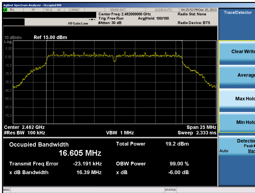
Plot 6-24. 6dB Bandwidth Plot (802.11g – Ch. 11)
