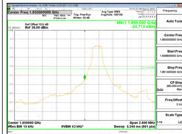
LTE B2 1.4MHz QPSK Low Channel RB1-0
