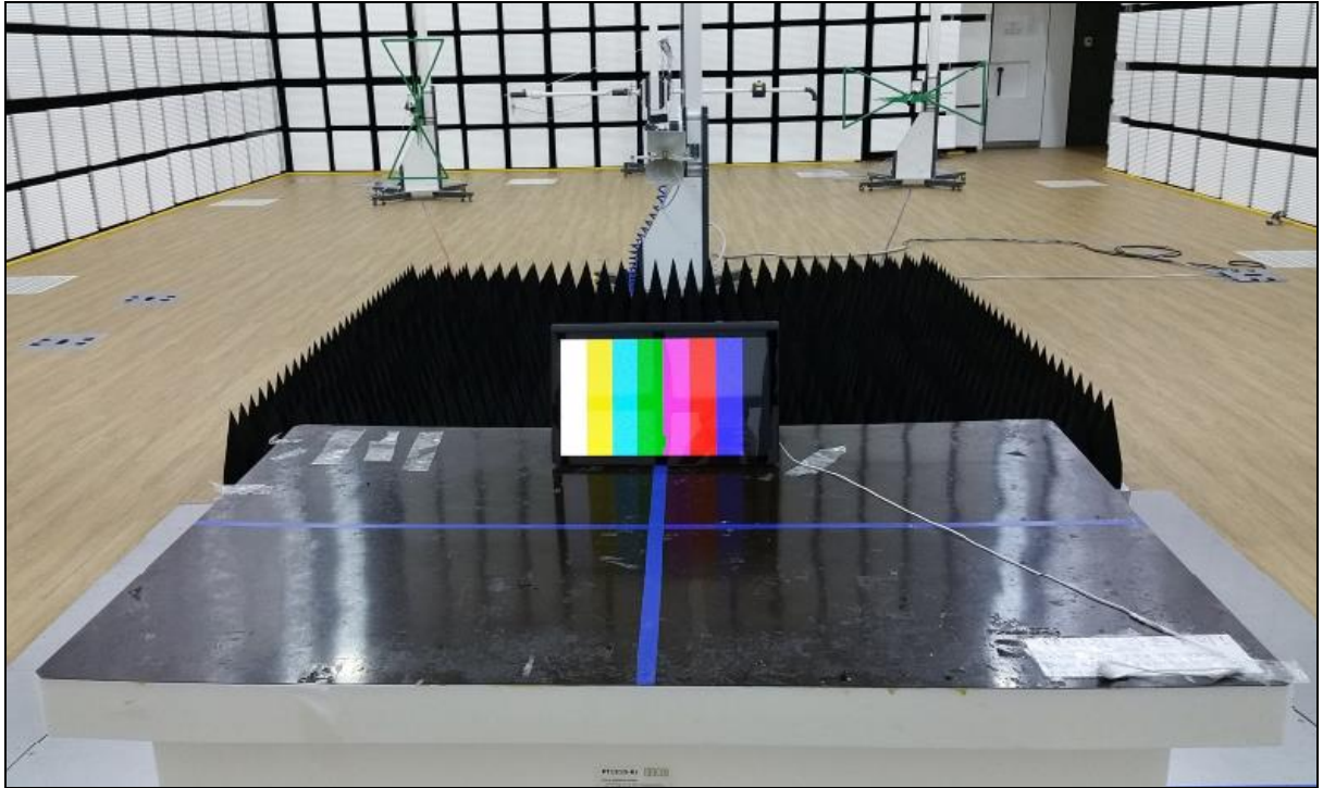
[ Mode 2 : Front ]
