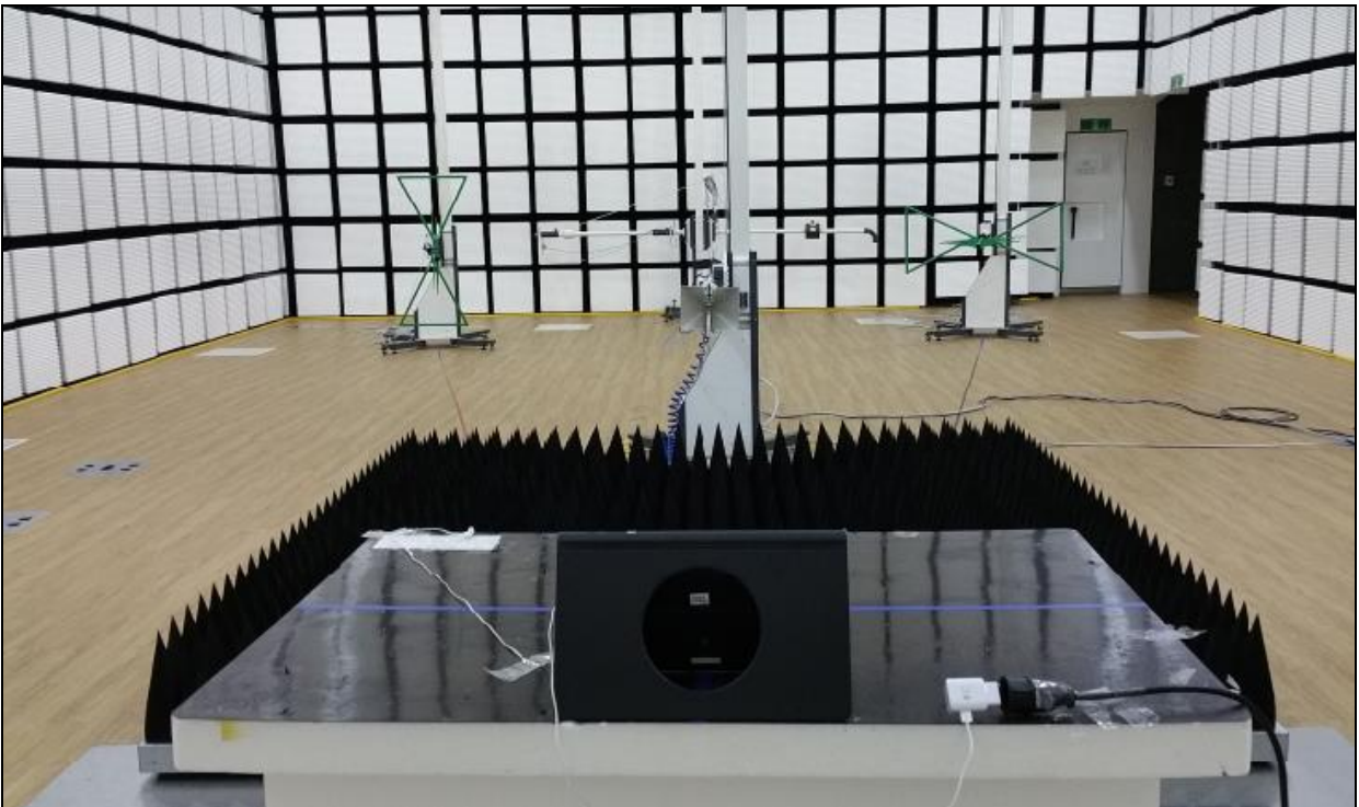
[ Mode 1 : Rear ]
