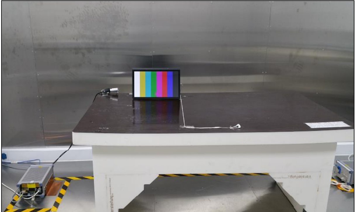
[ Mode 1 – 2 : Front ]
