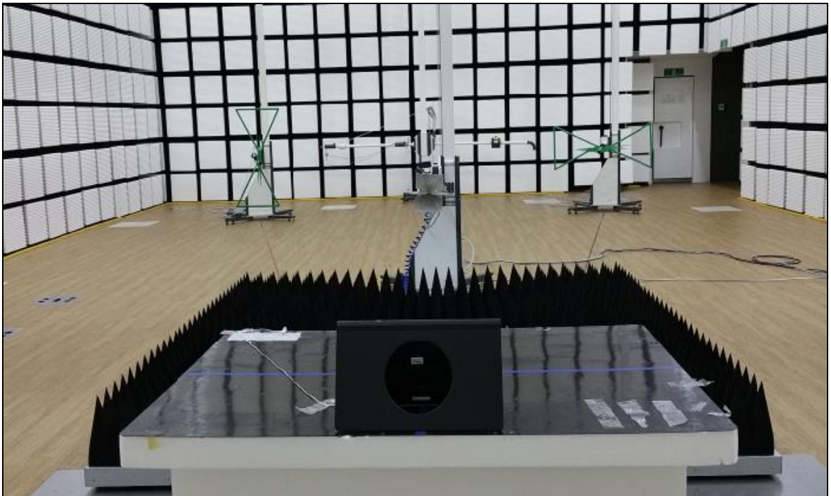
[ Mode 2 : Rear ]
