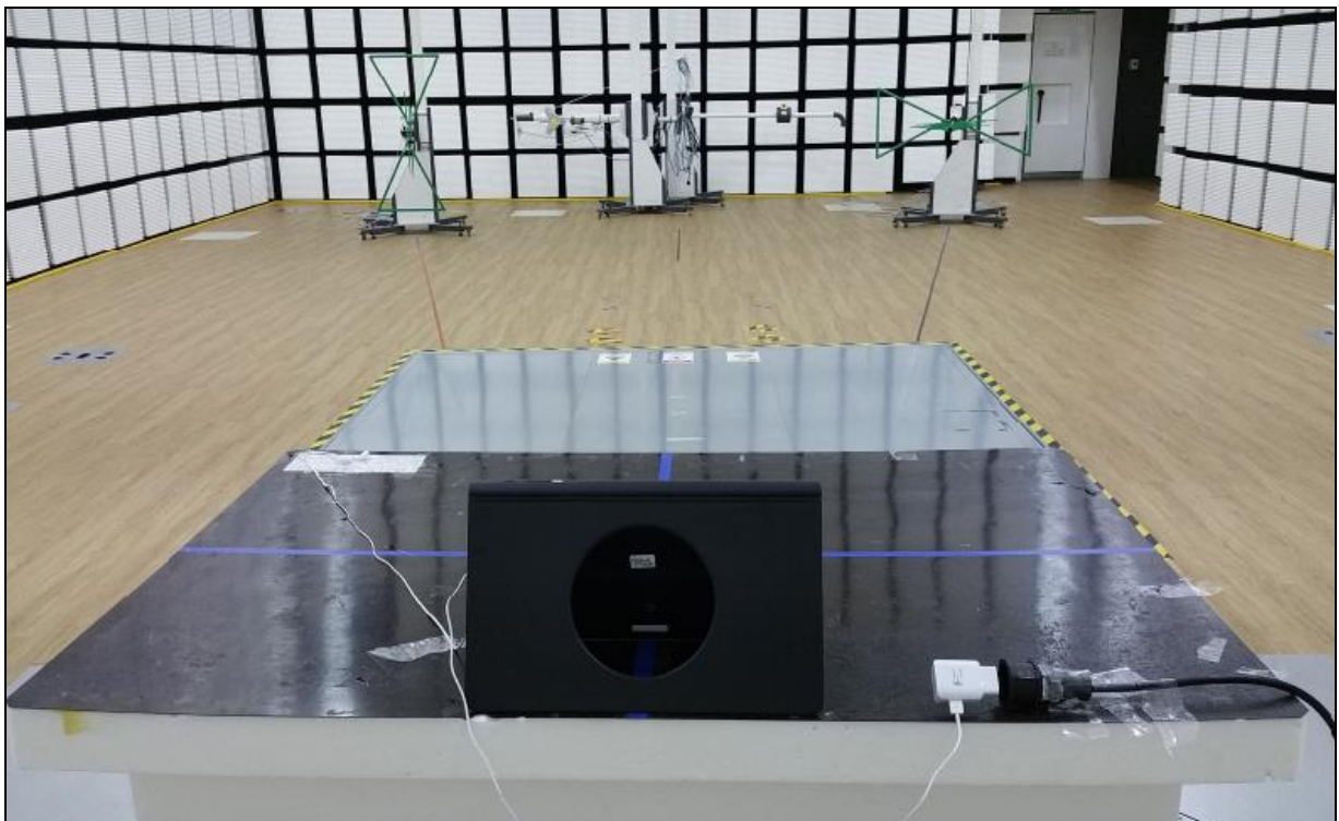
[ Mode 3 : Rear ]
