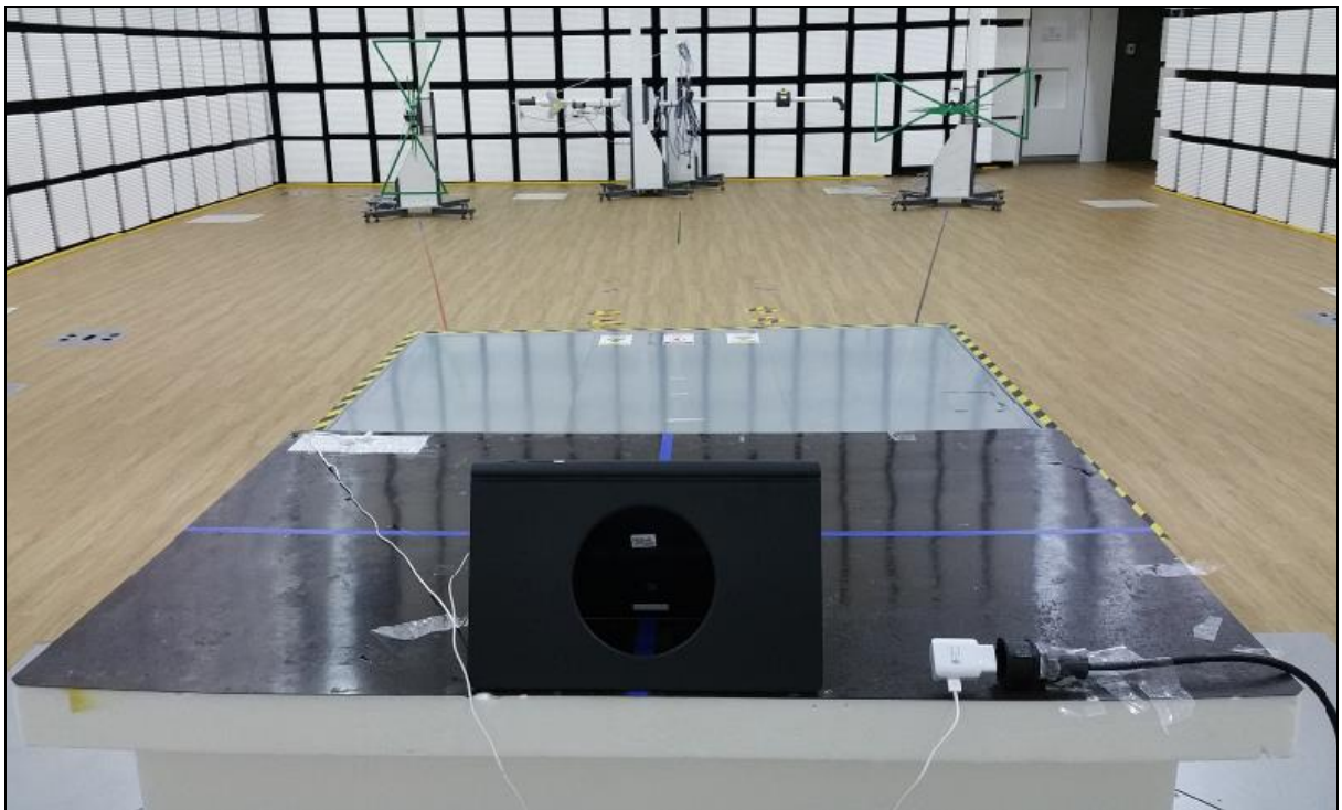
[ Mode 1 : Rear ]
