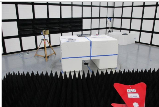
ABOVE 1GHz BACK PHOTO
