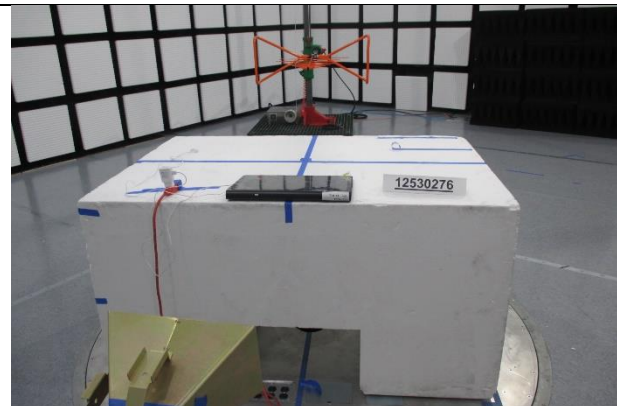
BELOW 1GHz FRONT PHOTO
