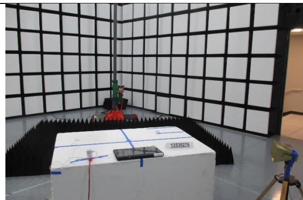
ABOVE 1GHz FRONT PHOTO
