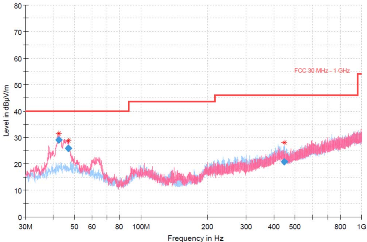
RSE(Below 1 GHz)_MIMO_2.4 GHz WLAN_802.11ax(HE20)_2412
