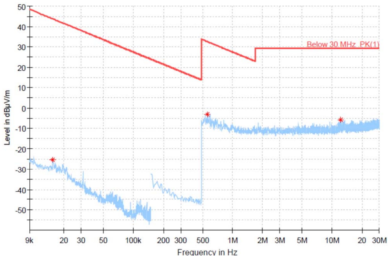
RSE(Below 30 MHz)_MIMO_2.4 GHz WLAN_802.11ax(HE20)_2412_X
