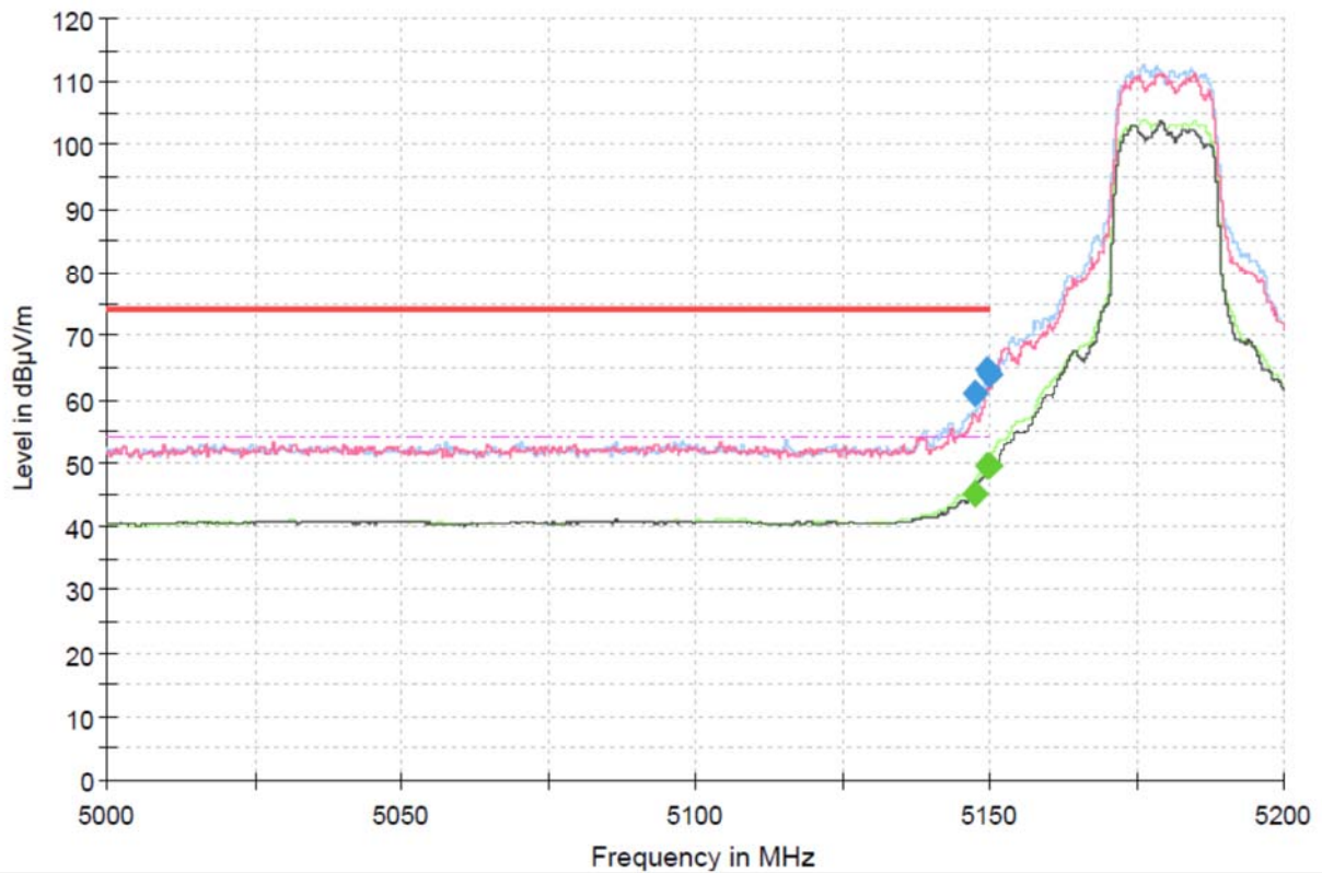
Band Edge_MIMO_UNII-1_802.11a_5180
